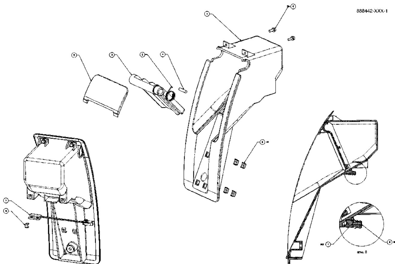
FIGURE 45. 888422-XXX - NOZZLE BOOT ASSY
