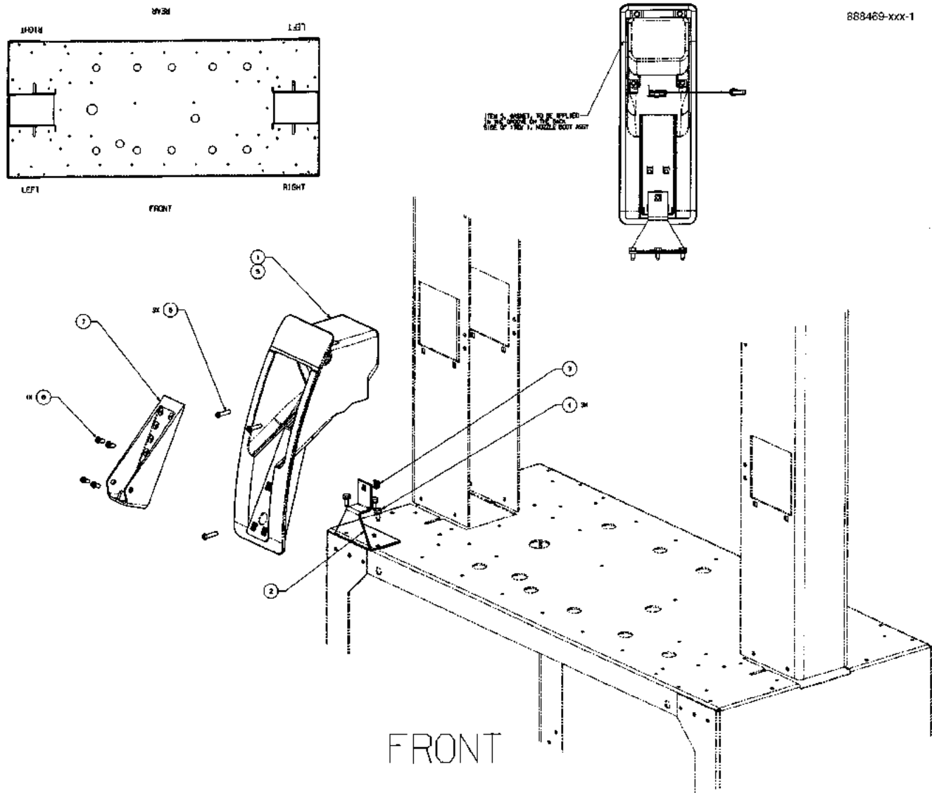
FIGURE 43. 888469-XXX - NOZZLE BOOT MODULE, OVATION
