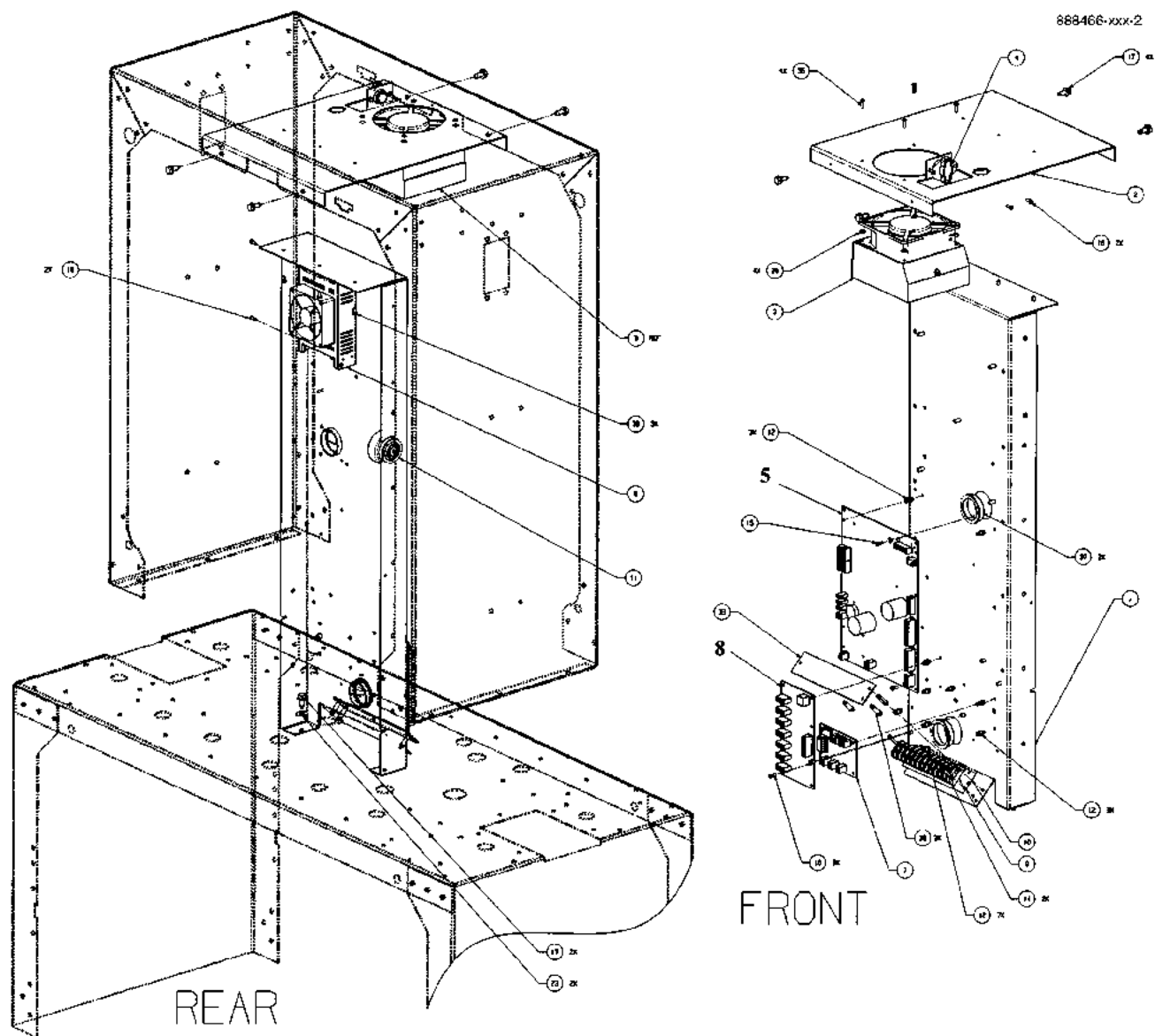
FIGURE 25. 888466-XXX - ELECTRONIC HEAD MODULE, OVATION QVGA
