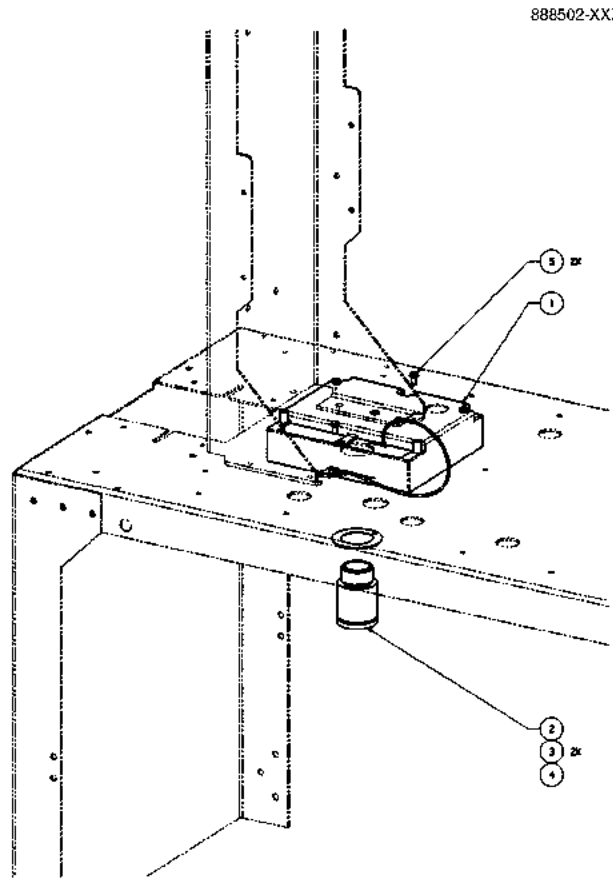
FIGURE 27. 888502-XXX - ELECTRICAL ISB MODULE
