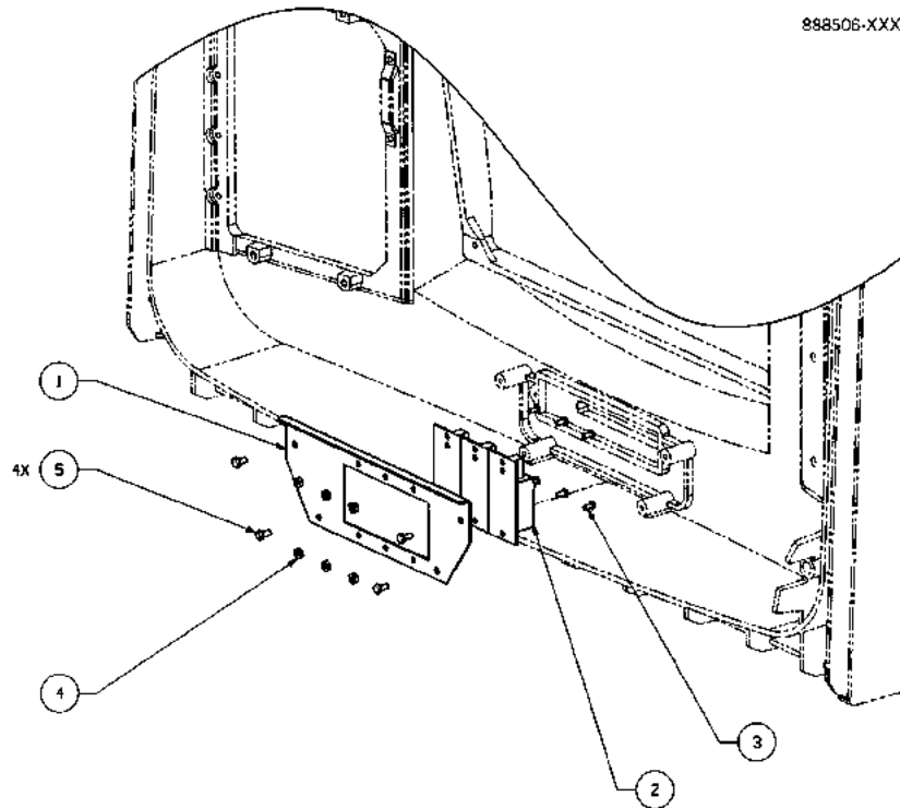
FIGURE 28. 888506-XXX - TOTALIZER MODULE, OVATION
