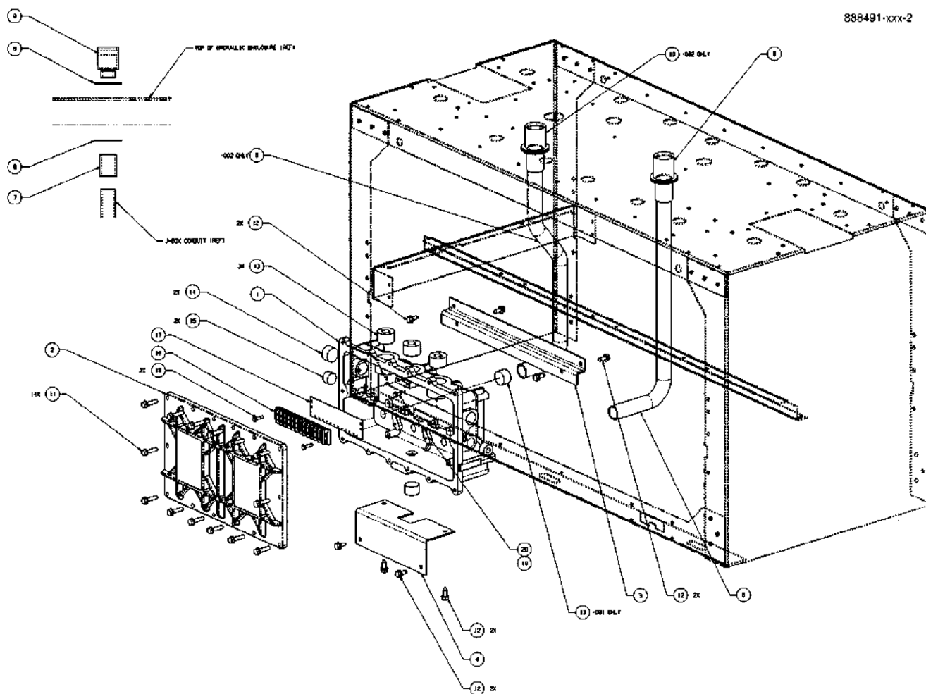
FIGURE 26. 888491-XXX - JUNCTION BOX MODULE, OVATION
