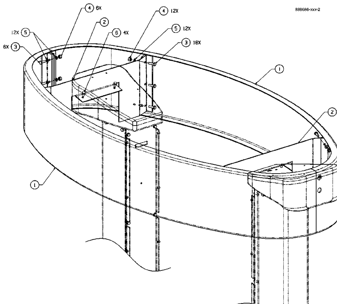
FIGURE 7. 888686-XXX - VALANCE MODULE, OVATION
