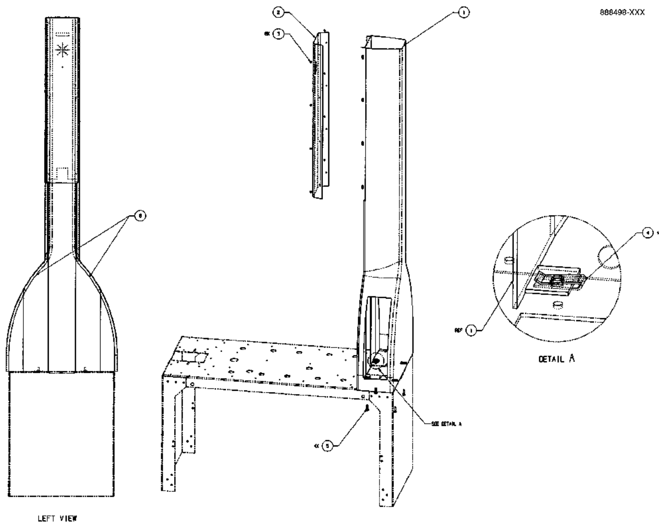
FIGURE 6. 888498-XXX - COLUMN COVER MODULE, OVATION
