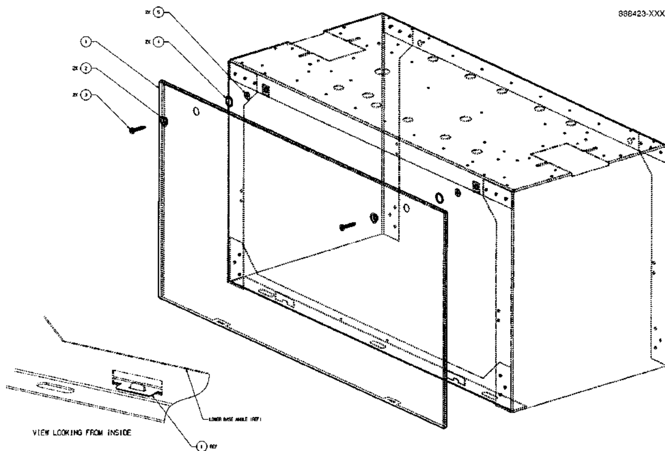
FIGURE 4. 888423-XXX - LOWER DOOR MODULE, OVATION
