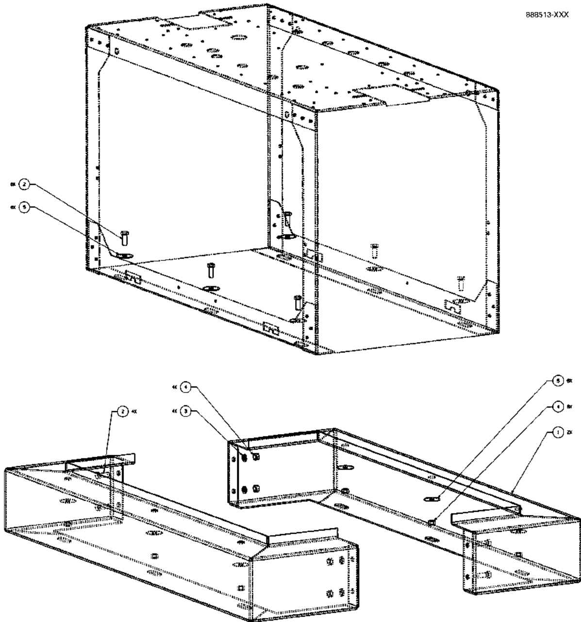
FIGURE 5. 888513-XXX - PEDESTAL MODULE, OVATION
