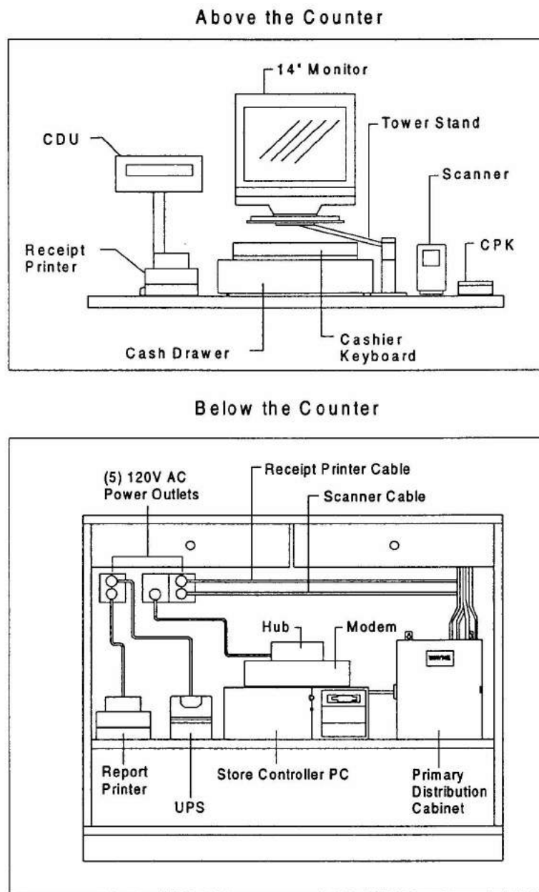
FIGURE 1. NUCLEUS SYSTEM OVERVIEW
