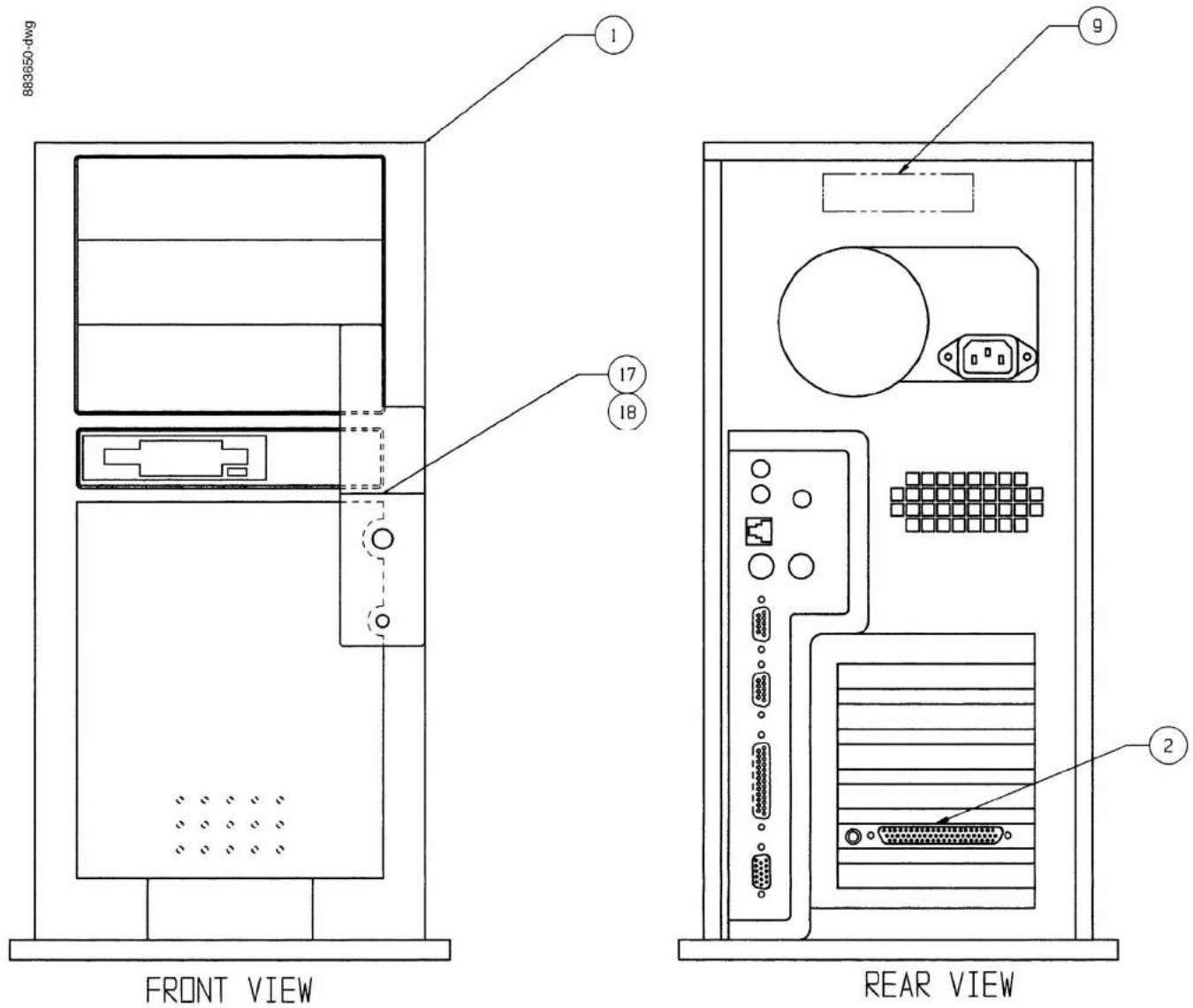
FIGURE 4. 883650-XXX - NUCLEUS IPT PC ASSEMBLY
