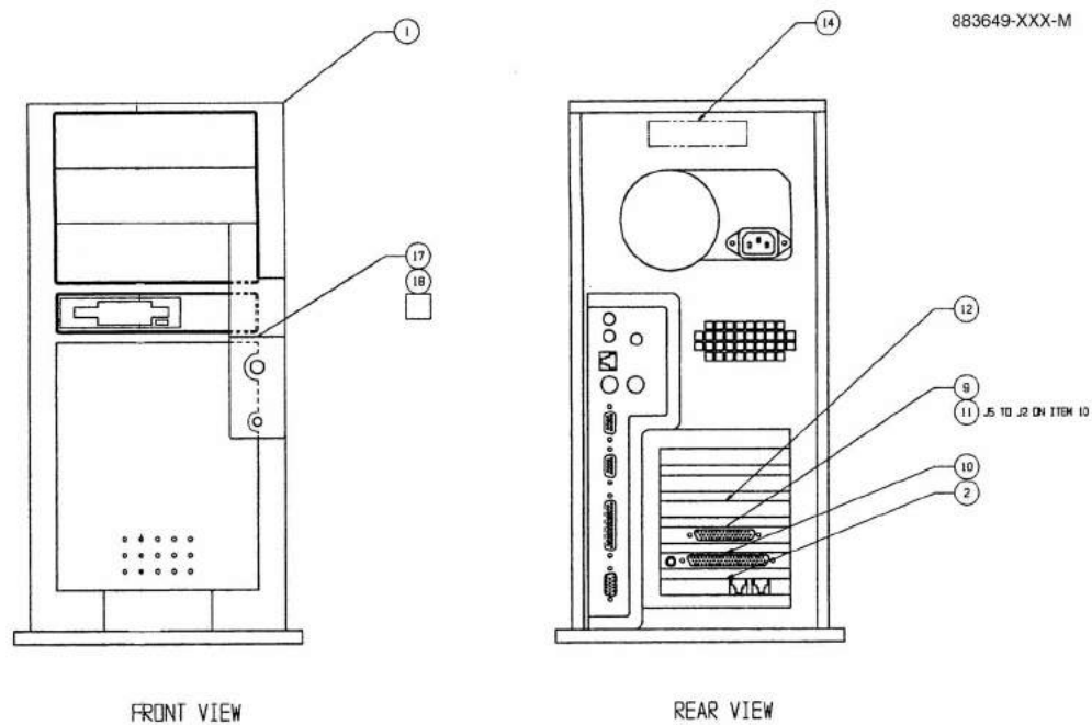
FIGURE 3. 883649-XXX - NUCLEUS SC PC ASSEMBLY SHELL
