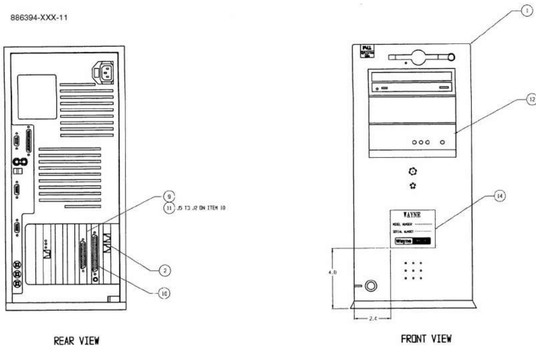
FIGURE 2. 886394-XXX - NUCLEUS SC PC ASSY GX110
