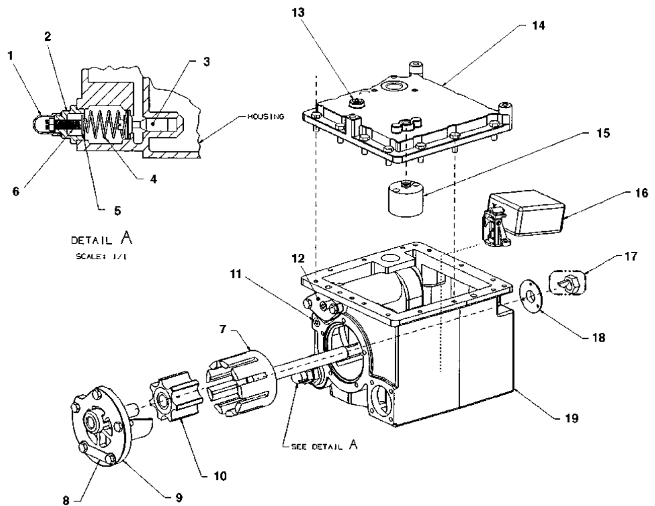
FIGURE 12. 47579-DWG - COMPACT PUMP UNIT ASSEMBLY VISTA & 1/VISTA
