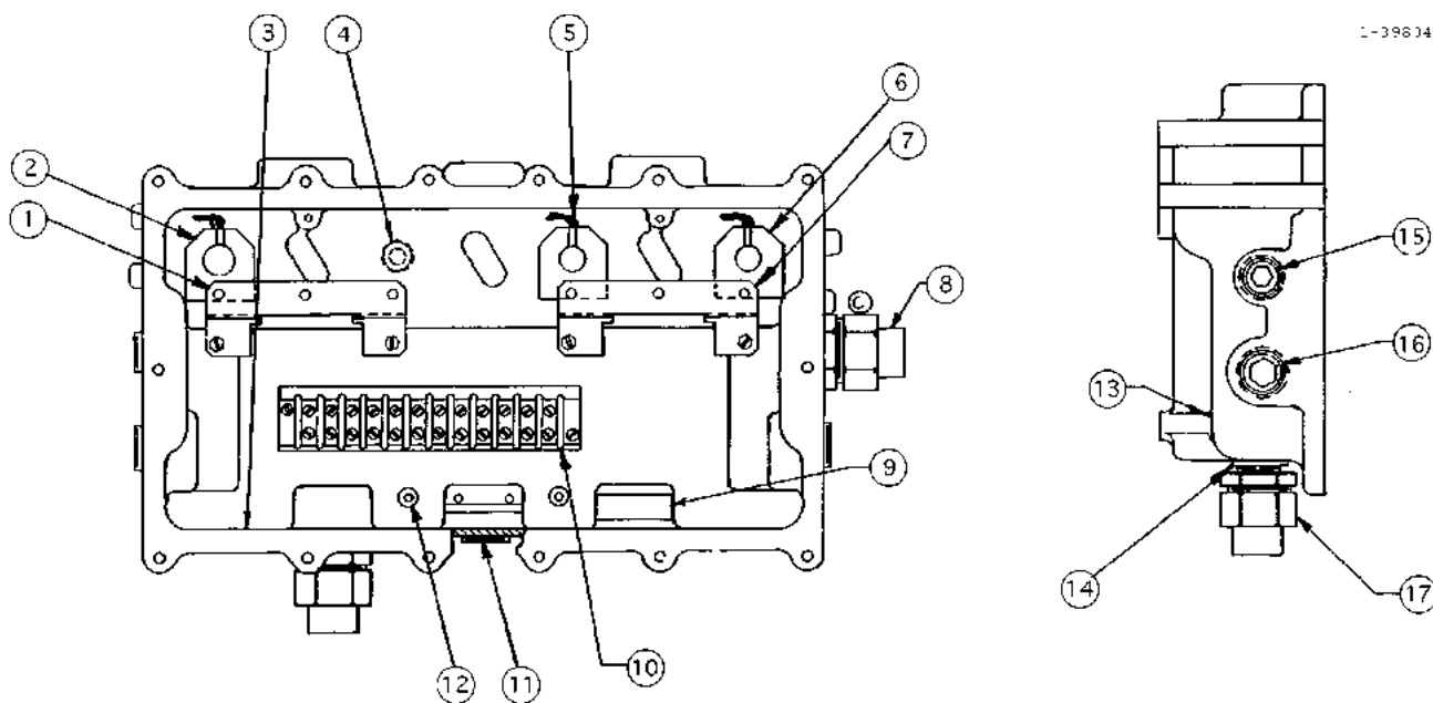
FIGURE 47. 1-39804 - JUNCTION BOX ASSEMBLY
