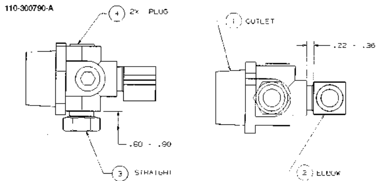
FIGURE 147. 110-300790-DWG - OUTLET BALANCE VAPOR RECOVERY 2/V590, 2/V591
