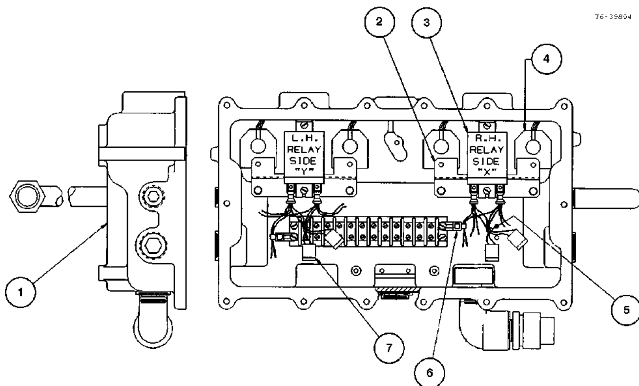
FIGURE 62. 76-39804 - JUNCTION BOX ASSEMBLY
