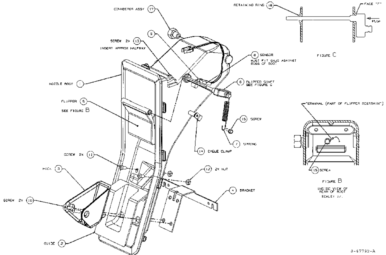
FIGURE 45. 8-47792-DWG - NOZZLE BOOT ASSEMBLY, PTS W/LOW NOZZLE HOOK
