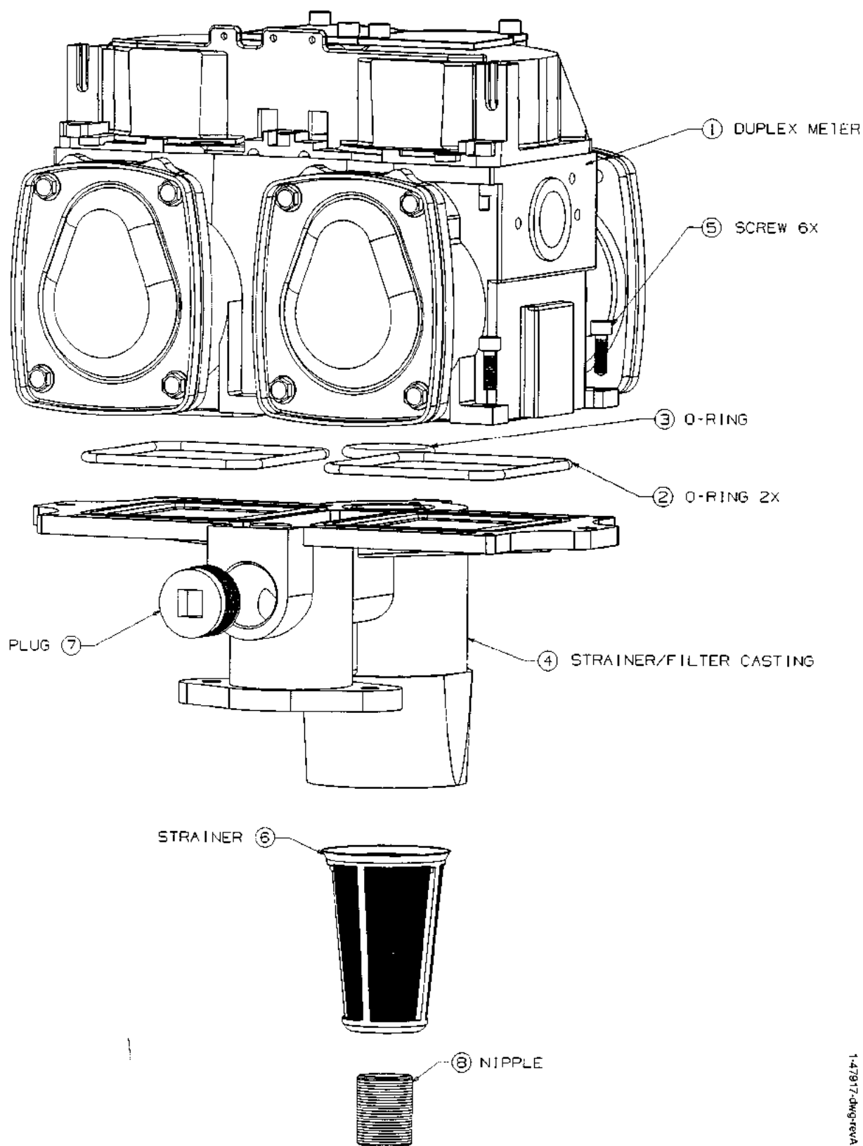
FIGURE 2. 1-47917-DWG - IMETER MODULE, REMOTE
