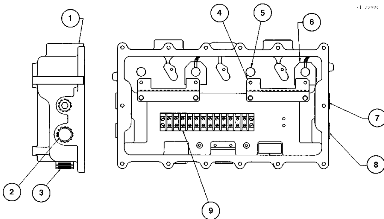
FIGURE 60. 74-39804 - JUNCTION BOX ASSEMBLY
