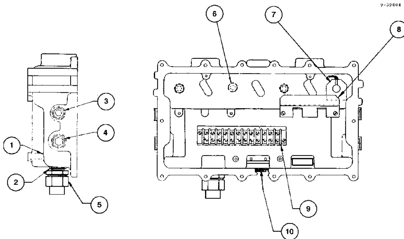
FIGURE 51. 9-39804 - JUNCTION BOX ASSEMBLY
