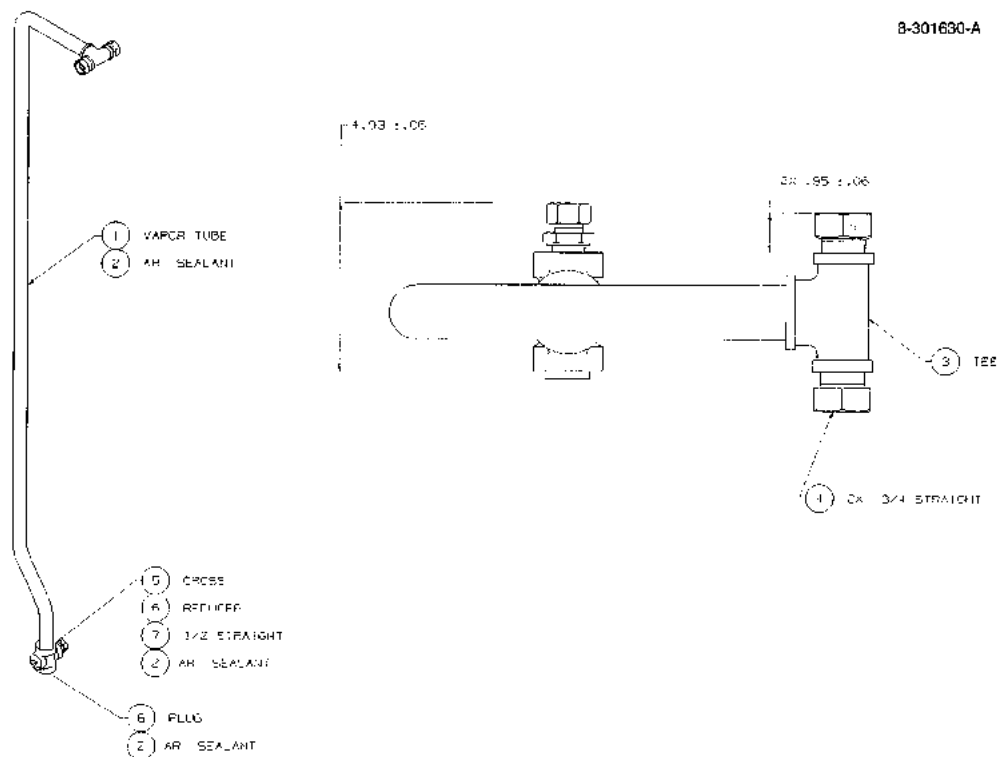
FIGURE 42. 8-301630-DWG - BALANCE VAPOR TUBE ASSEMBLY
