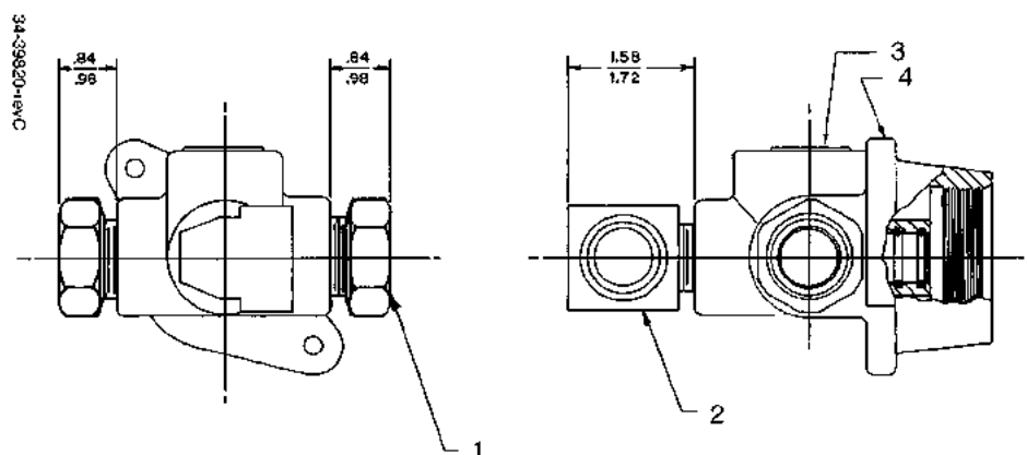
FIGURE 87. 34-39820 - OUTLET CASTING ASSEMBLY
