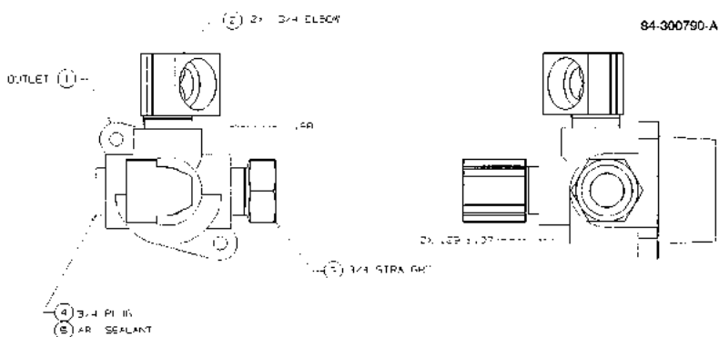
FIGURE 142. 84-300790-DWG - OUTLET BALANCE VAPOR RECOVERY 2/V595
