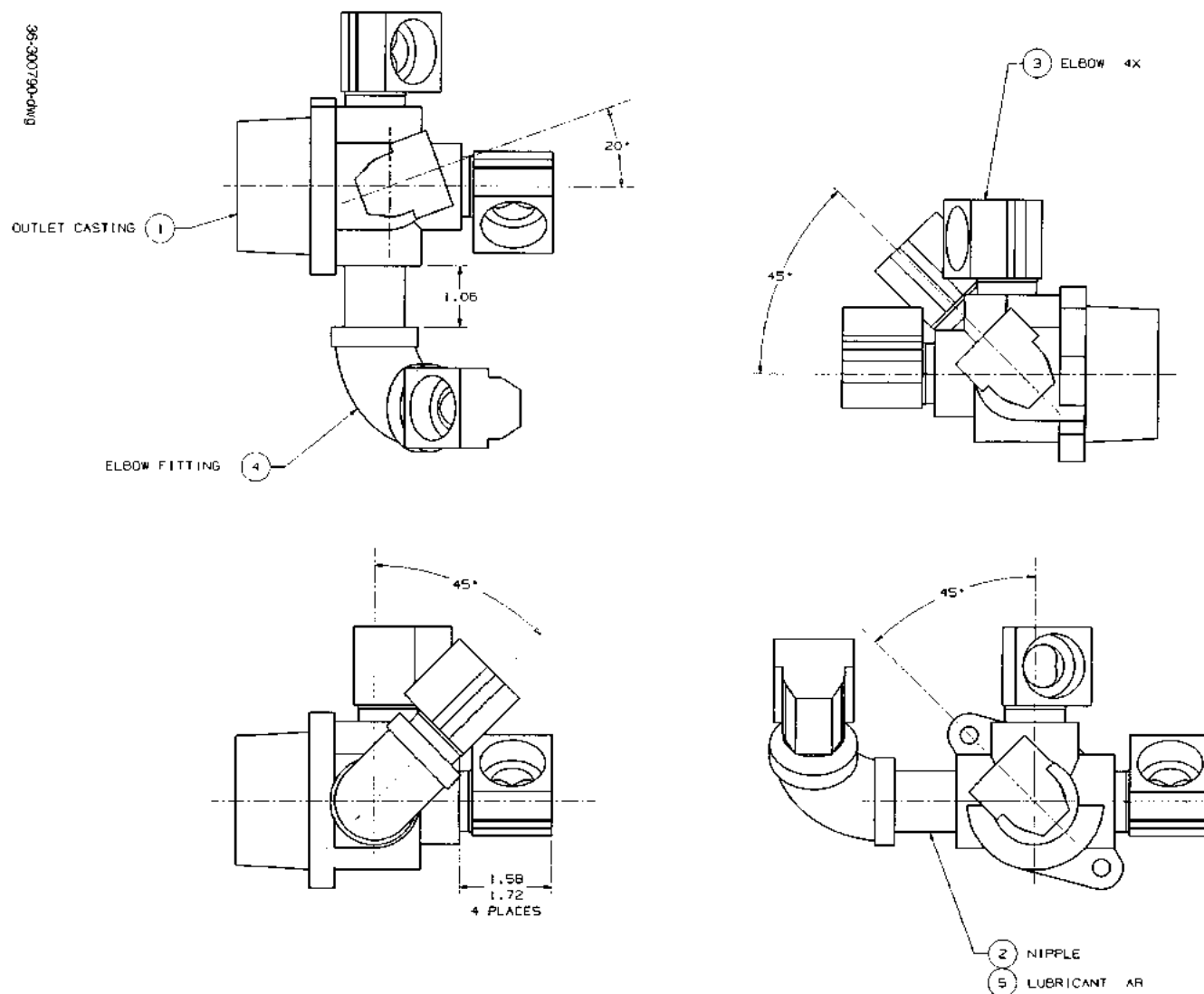
FIGURE 119. 36-300790-DWG - OUTLET & FITTINGS ASSEMBLY
