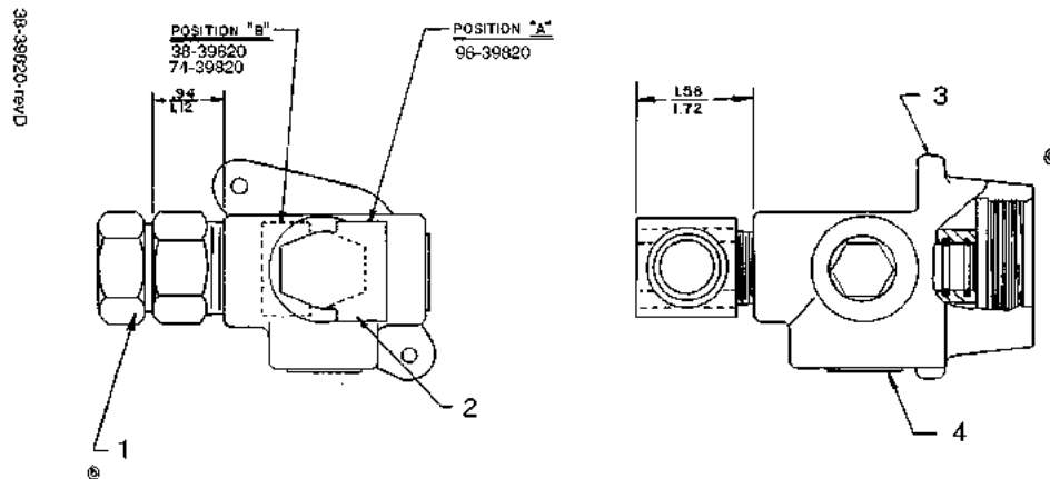
FIGURE 89. 38-39820 - OUTLET CASTING ASSEMBLY
