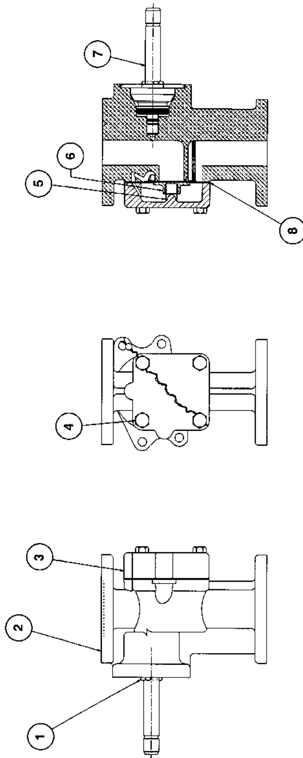
FIGURE 11. 1-47576 - DIAPHRAGM VALVE ASSEMBLY
