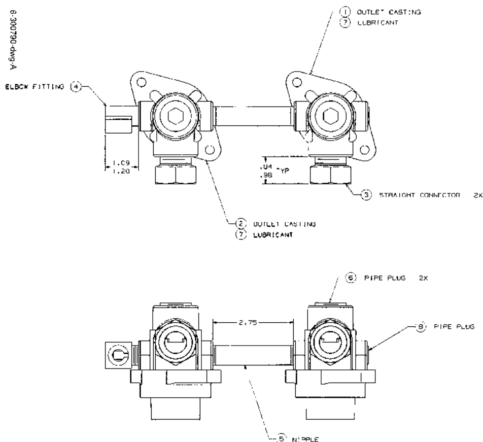
FIGURE 26. 6-300790-DWG - OUTLET AND FITTING ASSEMBLY
