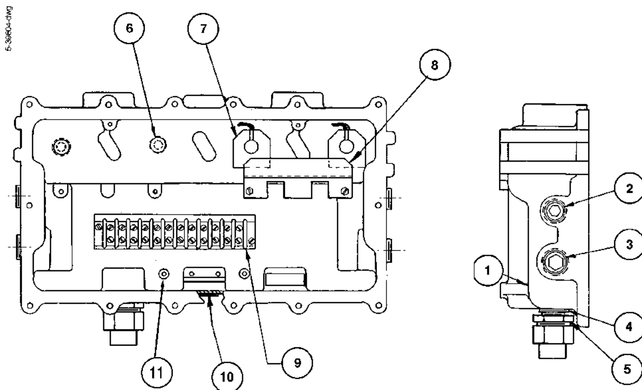
FIGURE 49. 5-39804-DWG - JUNCTION BOX ASSEMBLY
