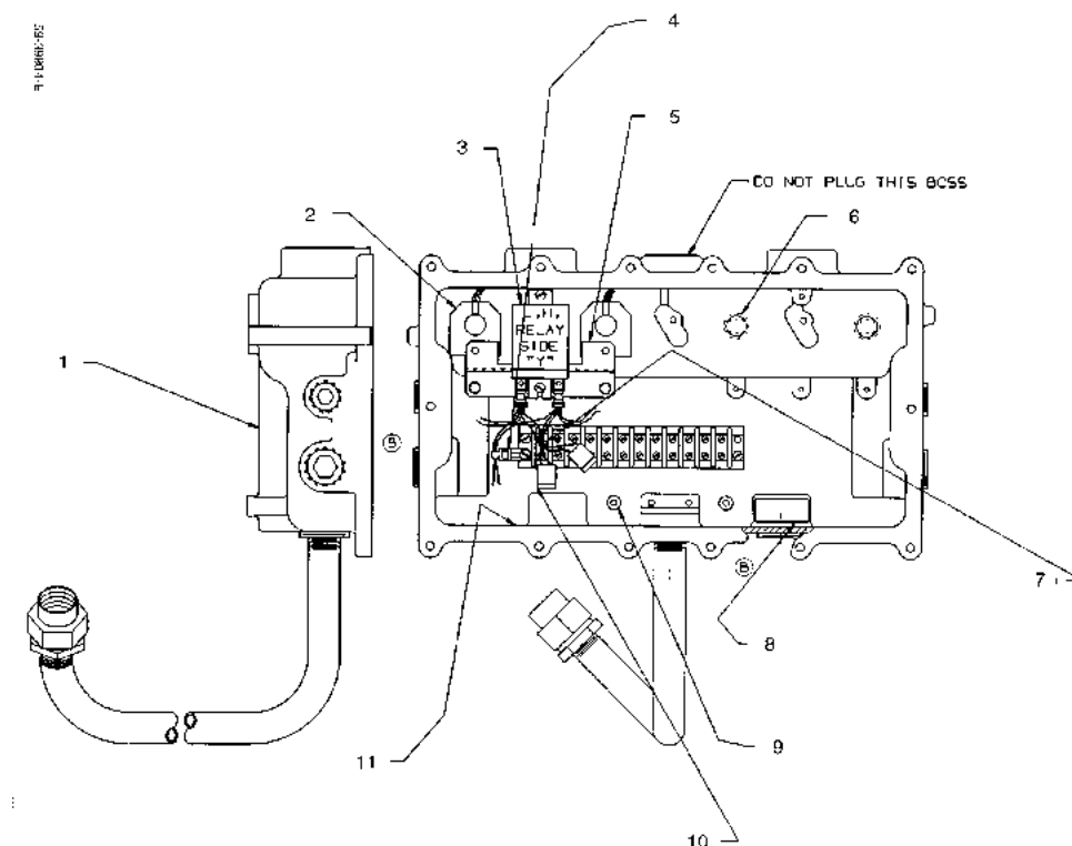
FIGURE 56. 59-39804 - JUNCTION BOX ASSEMBLY
