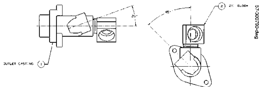
FIGURE 130. 57-300790-DWG - OUTLET & FITTING ASSEMBLY
