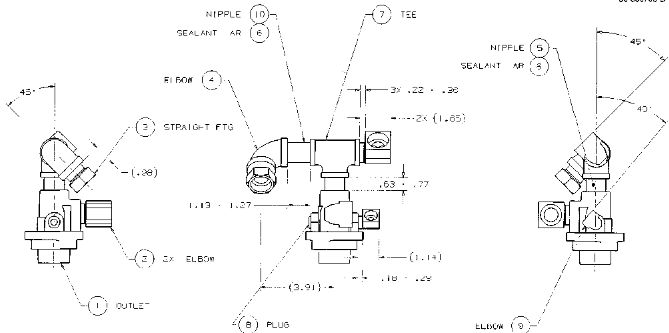
FIGURE 125. 50-300790-DWG - OUTLET &amp; FITTING ASSEMBLY
