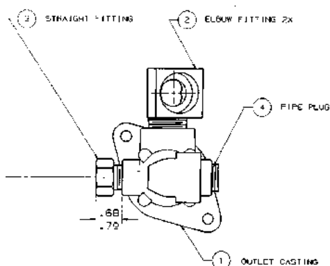
FIGURE 102. 4-300790-DWG - OUTLET &amp; FITTINGS ASSEMBLY
