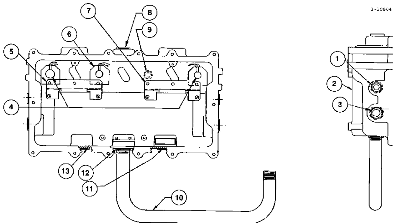
FIGURE 48. 3-39804 - JUNCTION BOX ASSEMBLY
