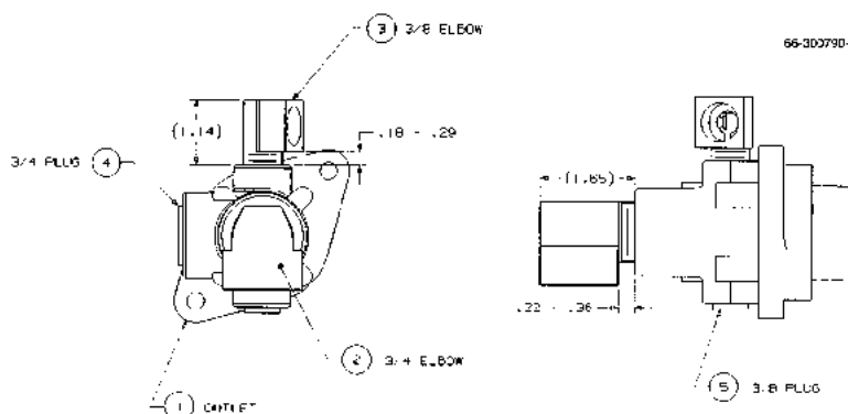
FIGURE 134. 66-300790-DWG - OUTLET WAYNE VAC VAPOR RECOVERY 2/V390
