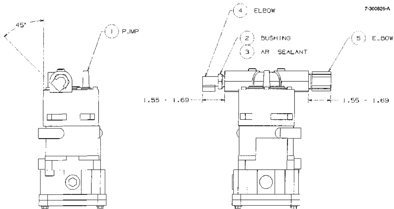
FIGURE 34. 7-300826-DWG - UPPER VACUUM PUMP SUCTION
