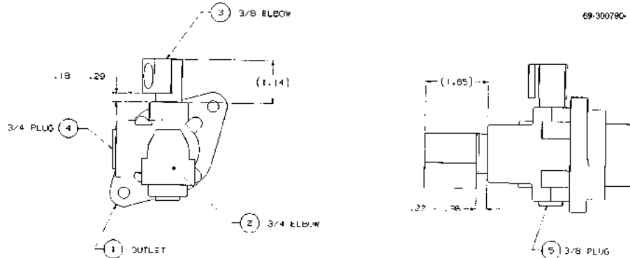
FIGURE 136. 69-300790-DWG - OUTLET WAYNE VAC VAPOR RECOVERY 2/V390
