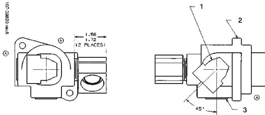
FIGURE 94. 107-39820 - OUTLET CASTING ASSEMBLY
