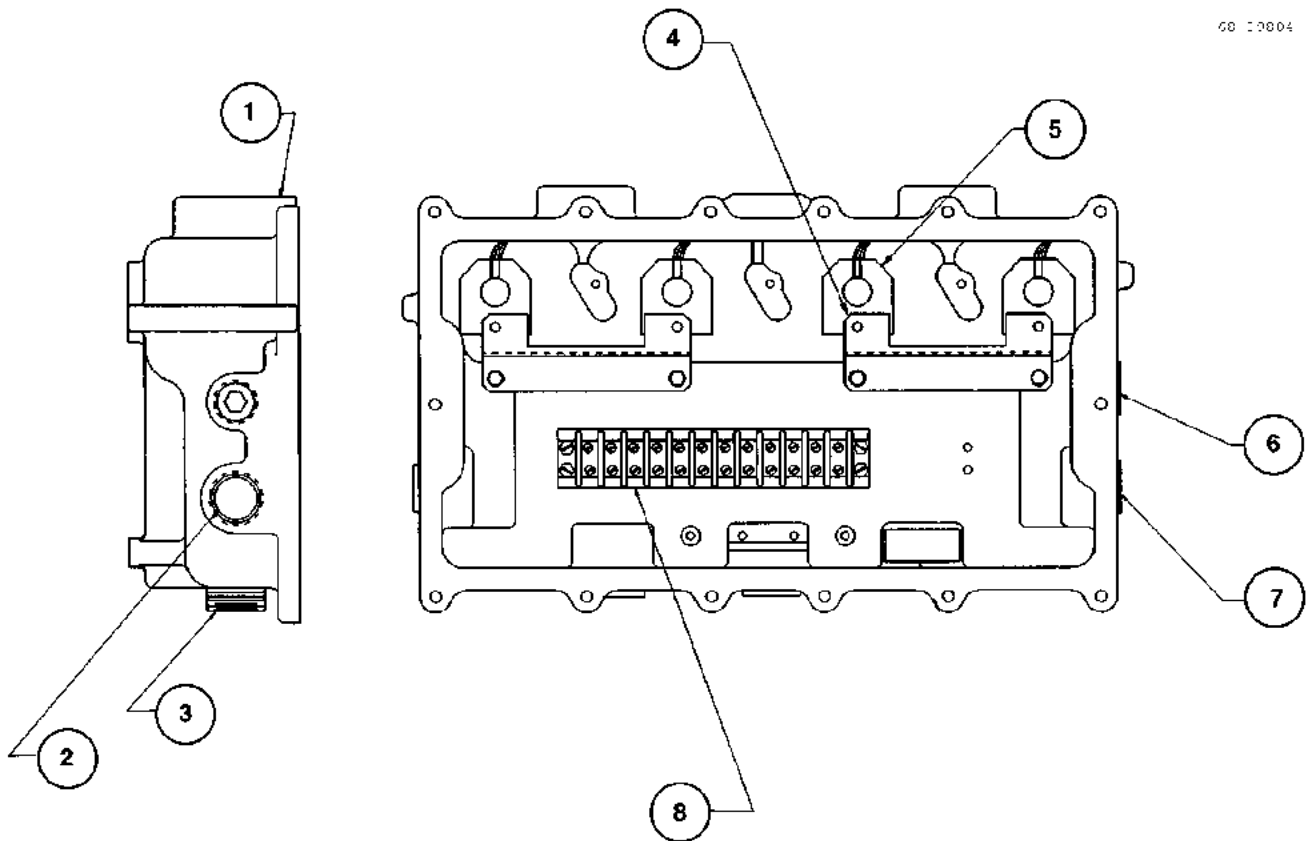
FIGURE 58. 68-39804 - JUNCTION BOX ASSEMBLY
