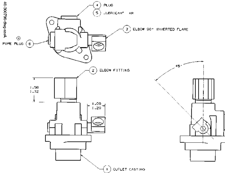
FIGURE 123. 40-300790-DWG - OUTLET & FITTING ASSEMBLY
