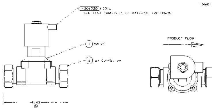
FIGURE 150. 1-301831-DWG - VALVE & FITTINGS
