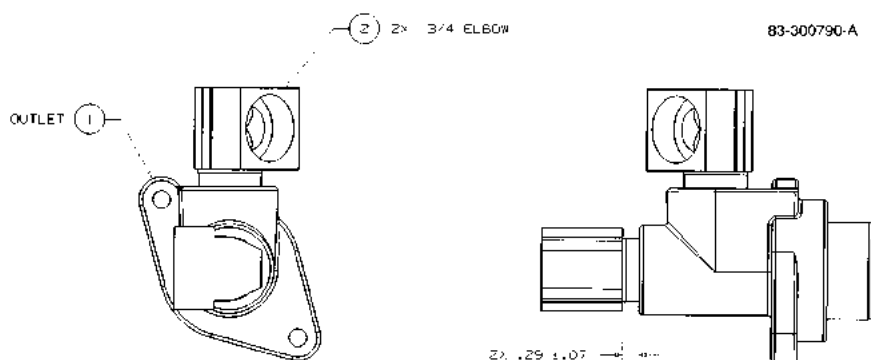
FIGURE 141. 83-300790-DWG - OUTLET NON-VAPOR RECOVERY 2/V595
