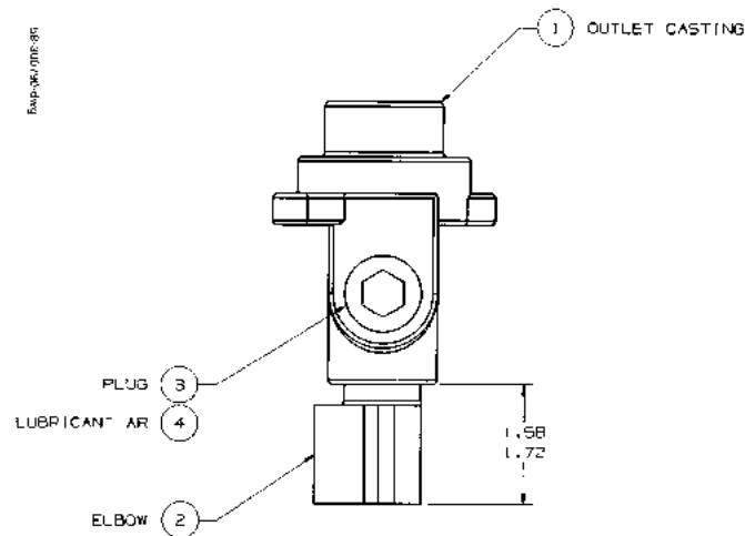
FIGURE 131. 58-300790-DWG - OUTLET & FITTING ASSEMBLY
