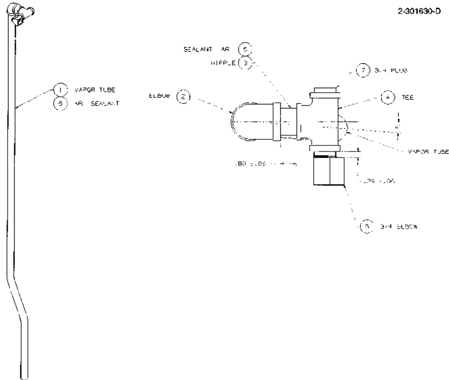
FIGURE 39. 2-301630-DWG - BALANCE VAPOR TUBE ASSEMBLY
