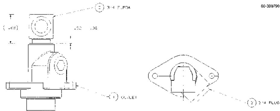
FIGURE 132. 60-300790-DWG - OUTLET NON-VAPOR RECOVERY 2/V390
