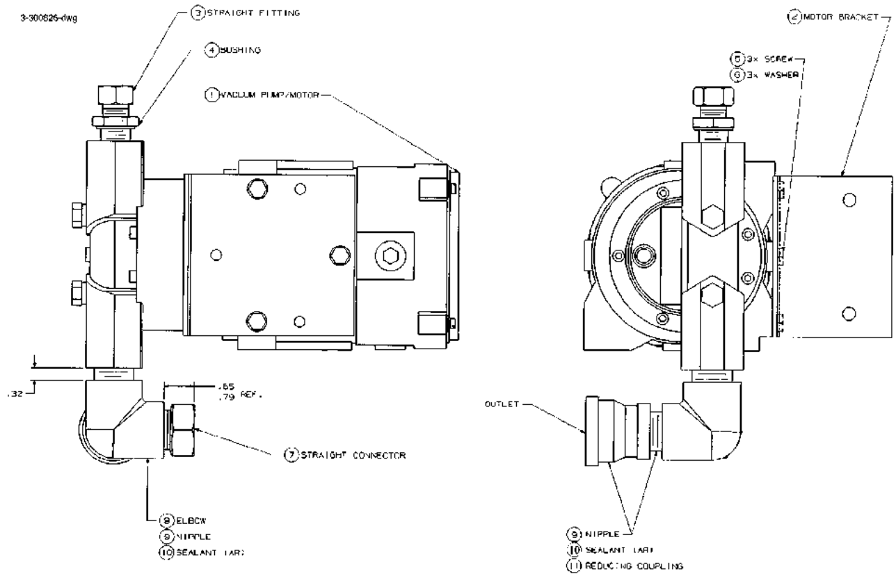
FIGURE 31. 3-300826-DWG - PUMP/MOTOR & BRACKET ASSEMBLY
