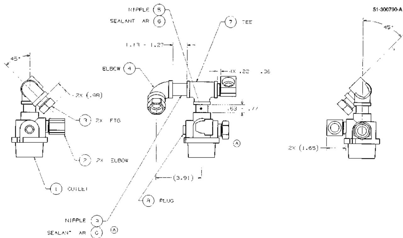
FIGURE 126. 51-300790-DWG - OUTLET & FITTING ASSEMBLY
