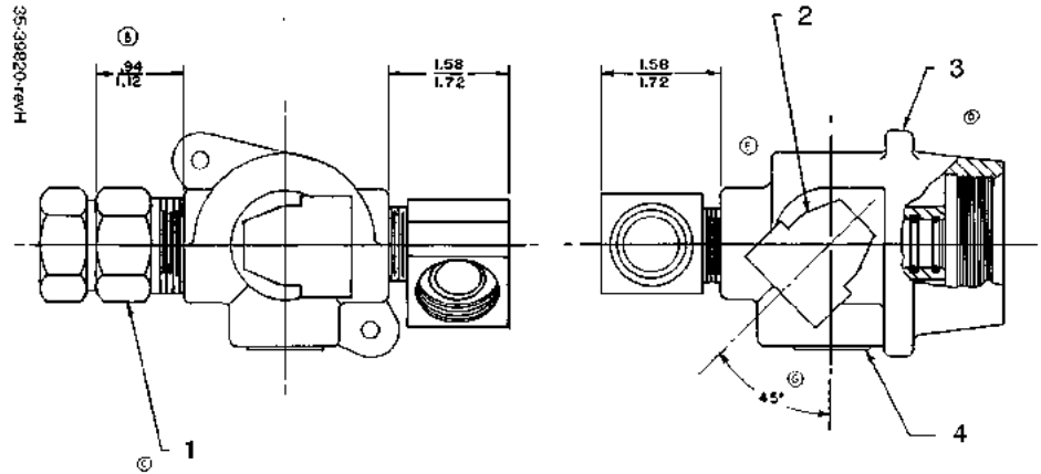
FIGURE 88. 35-39820 - OUTLET CASTING ASSEMBLY
