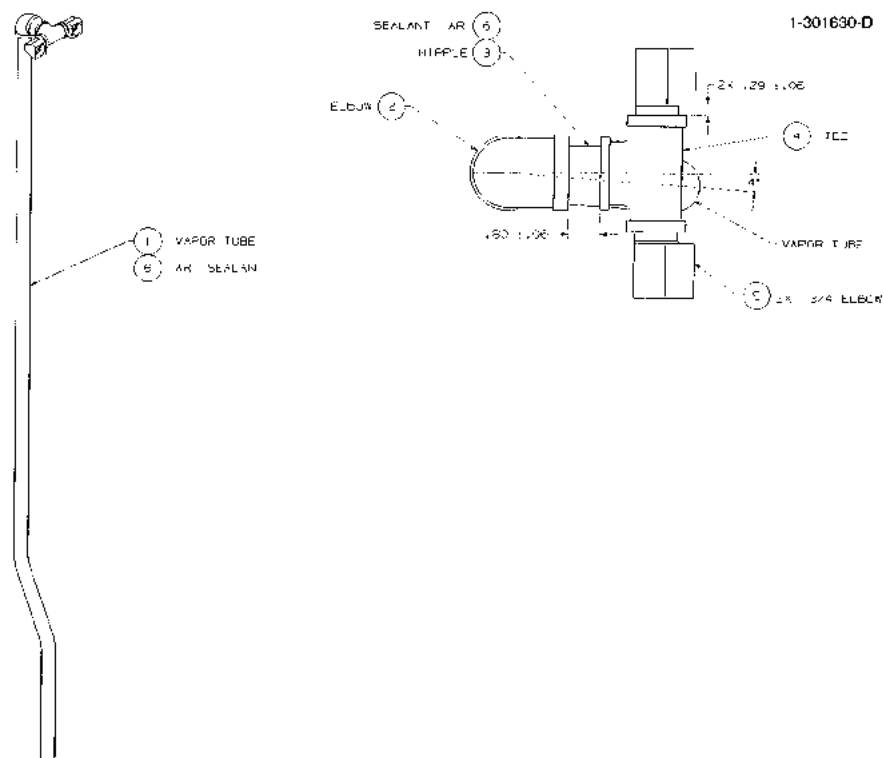
FIGURE 38. 1-301630-DWG - BALANCE VAPOR TUBE ASSEMBLY
