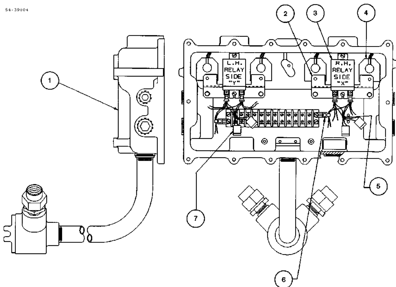
FIGURE 55. 54-39804 - JUNCTION BOX ASSEMBLY
