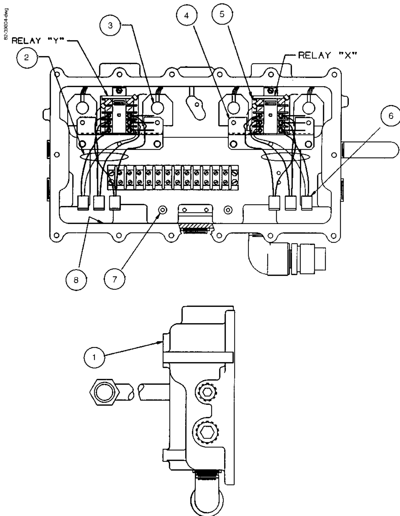
FIGURE 63. 82-39804-DWG - JUNCTION BOX ASSEMBLY
