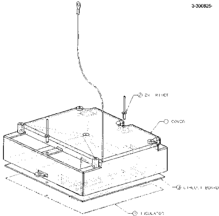
FIGURE 75. 3-300825-DWG - INTRINSIC SAFE BOARD & COVER ASSEMBLY
