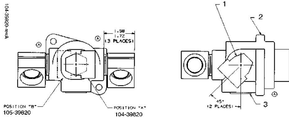
FIGURE 92. 104 & 105-39820 - OUTLET CASTING ASSEMBLY
