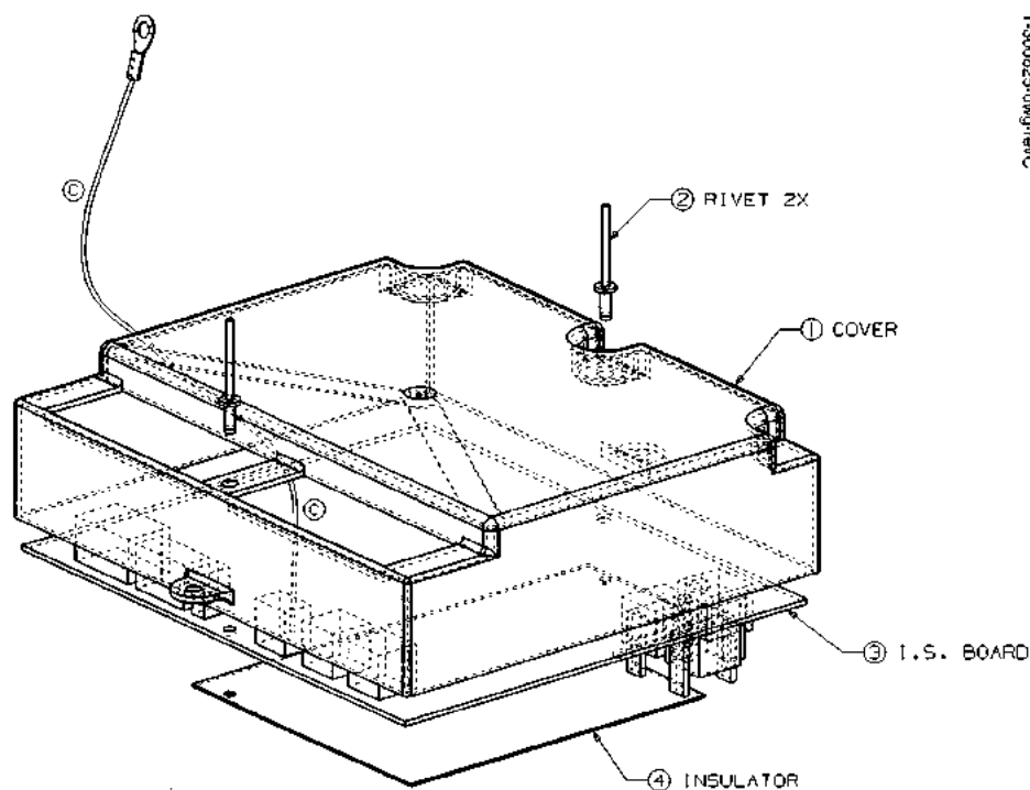
FIGURE 74. 1-300825-DWG - INTRINSIC SAFE BOARD & COVER ASSEMBLY
