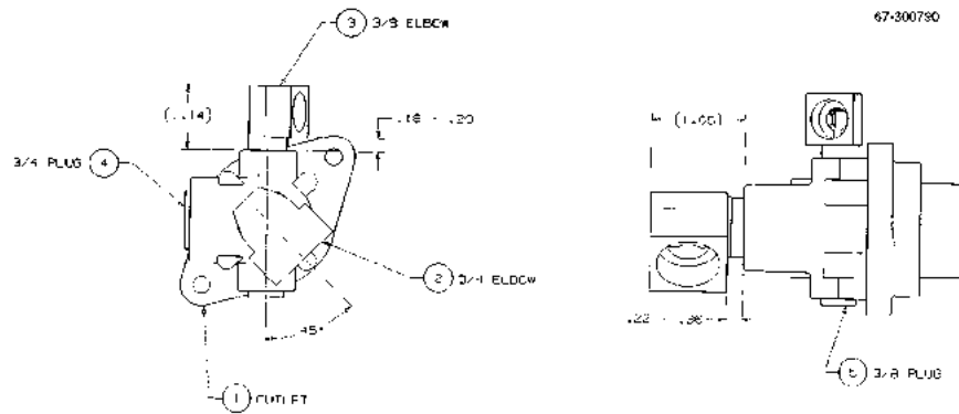
FIGURE 135. 67-300790-DWG - OUTLET WAYNE VAC VAPOR RECOVERY 2/V390
