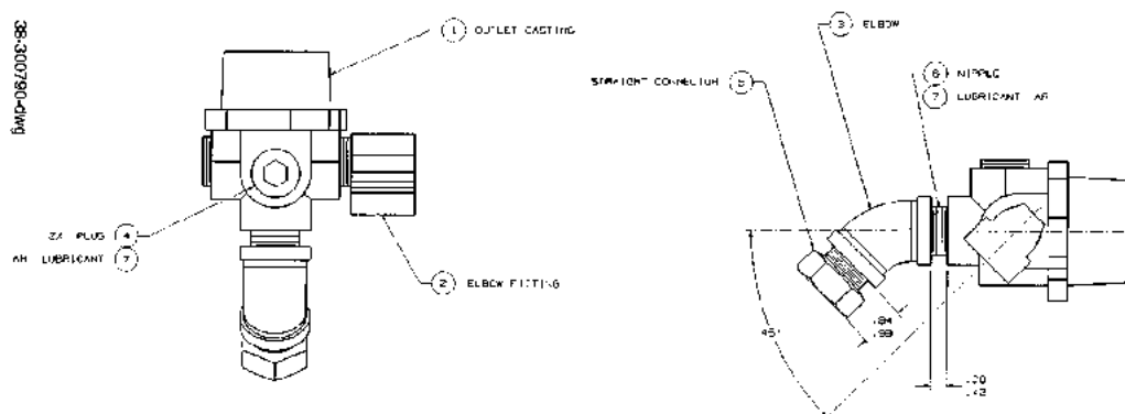
FIGURE 121. 38-300790-DWG - OUTLET &amp; FITTINGS ASSEMBLY
