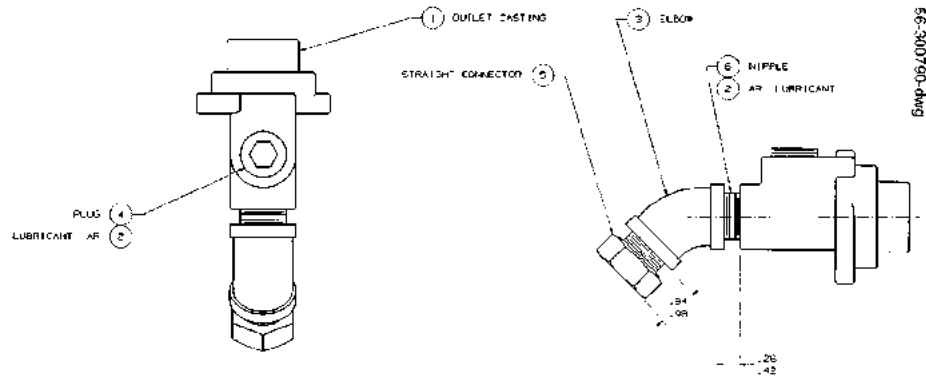
FIGURE 129. 56-300790-DWG - OUTLET & FITTING ASSEMBLY
