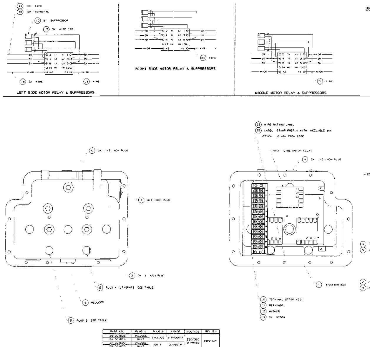
FIGURE 69. 25-301825-DWG - JUNCTION BOX ASSY THREE PRODUCT 3 PHASE
