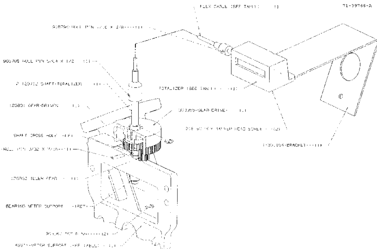
FIGURE 9. 71-39786-DWG - METER SUPPORT & TOTALIZER ASSY
