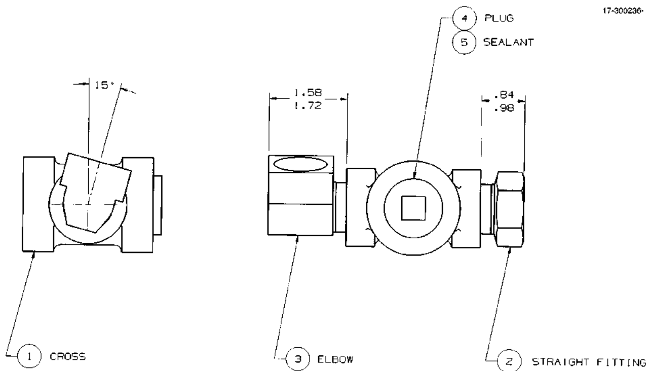
FIGURE 24. 17-300236-DWG - CROSS AND INVERTED FLARE FITTINGS ASSY
