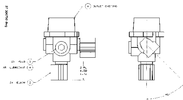
FIGURE 120. 37-300790-DWG - OUTLET &amp; FITTINGS ASSEMBLY
