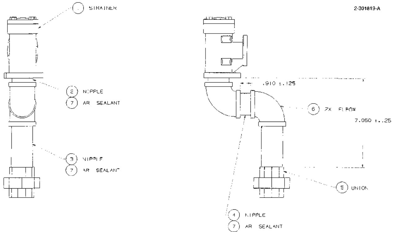
FIGURE 7. 2-301819-DWG - STRAINER ASSEMBLY SUCTION
