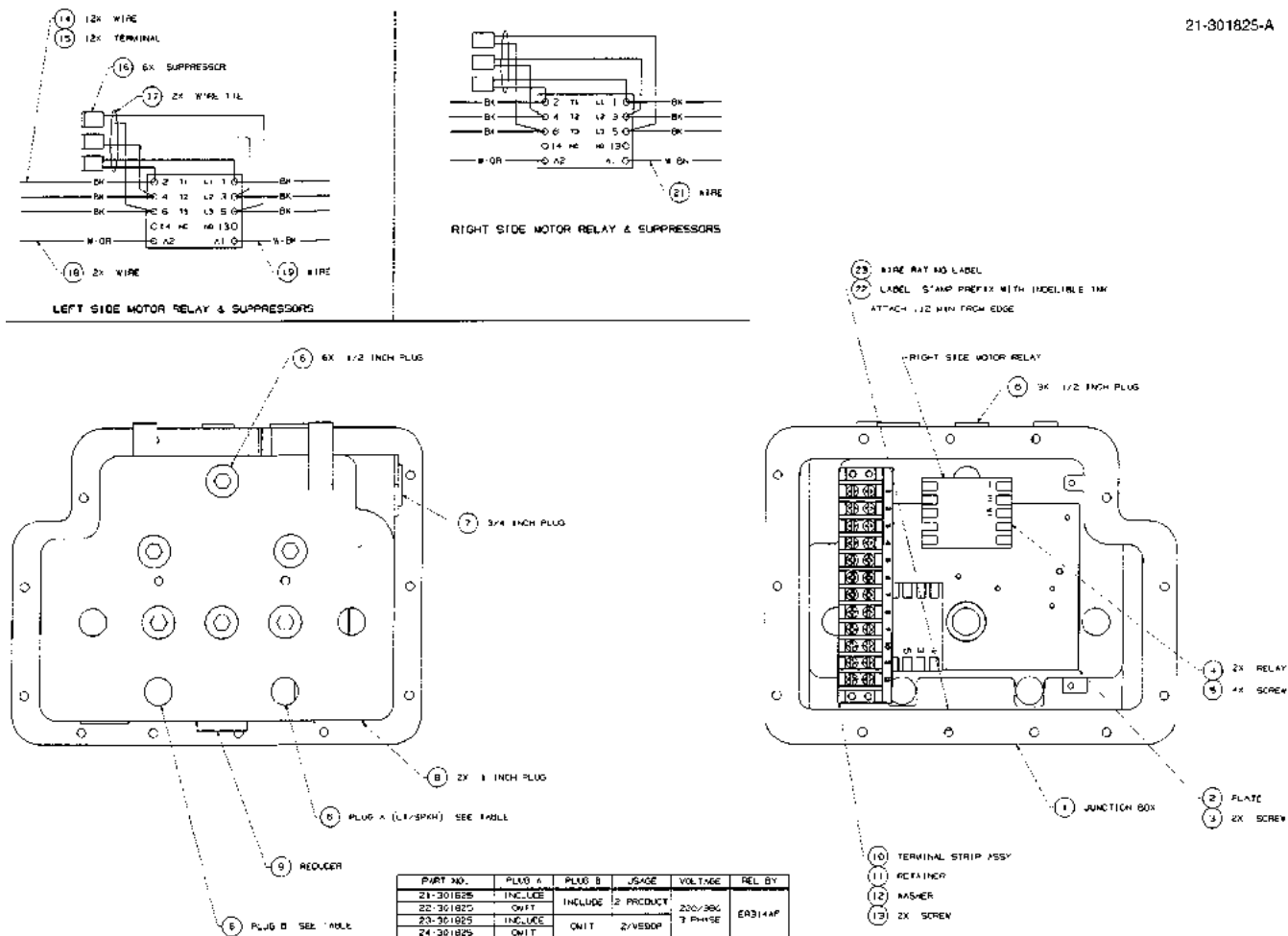
FIGURE 68. 21-301825-DWG - JUNCTION BOX ASSY TWO PRODUCT 3 PHASE
