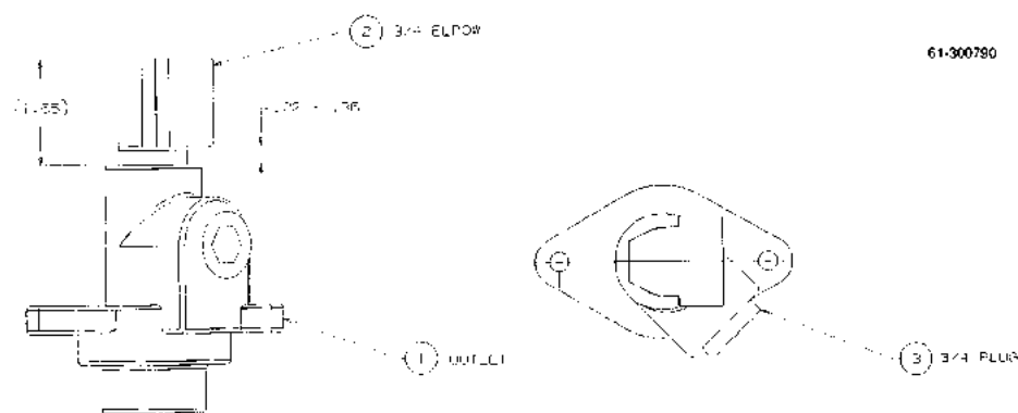
FIGURE 133. 61-300790-DWG - OUTLET NON-VAPOR RECOVERY 2/V490
