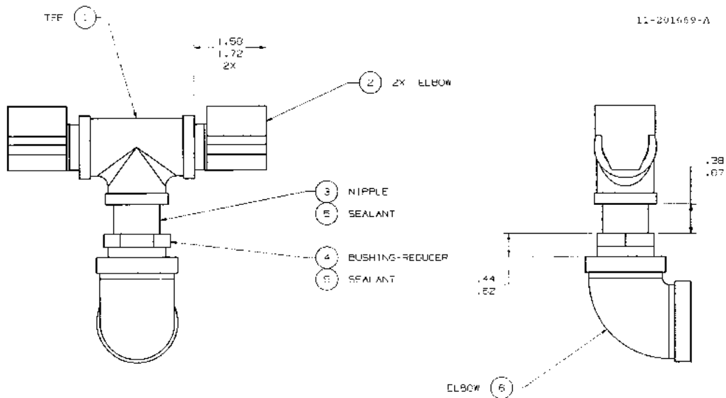
FIGURE 20. 11-201669-DWG - TEE ASSEMBLY
