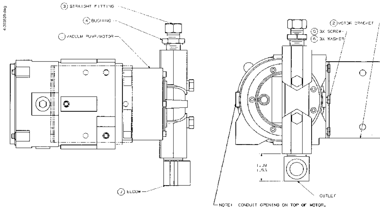
FIGURE 32. 4-300826-DWG - PUMP MOTOR & BRACKET ASSEMBLY
