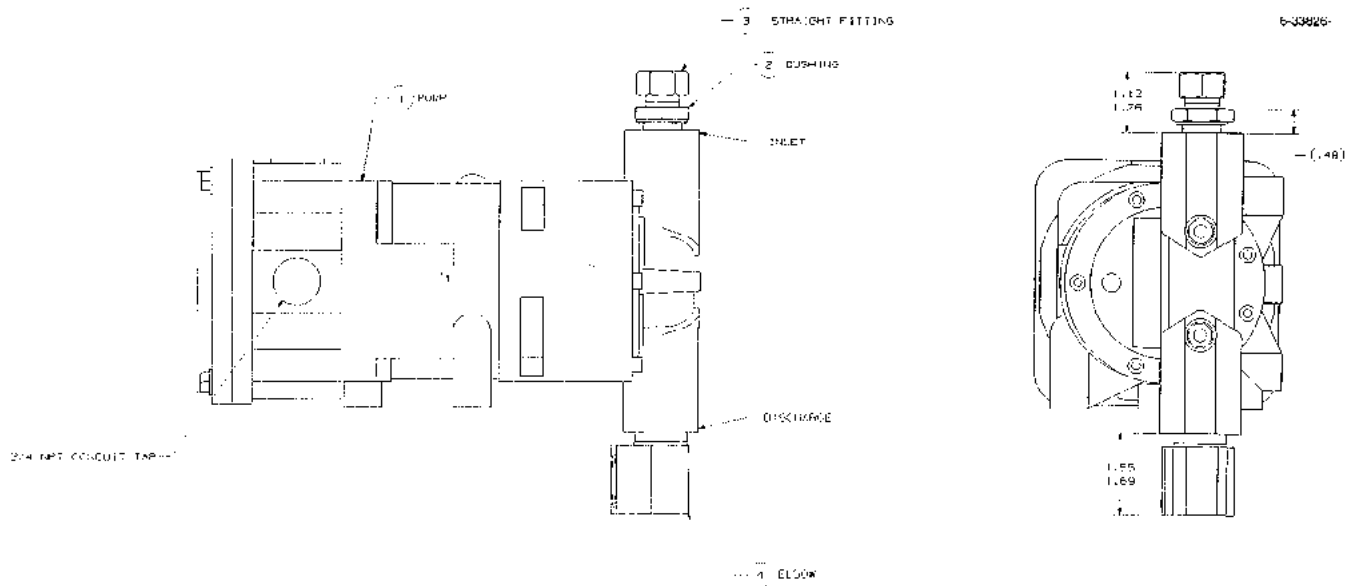
FIGURE 33. 6-300826-DWG - VACUUM PUMP AND FITTINGS ASSEMBLY
