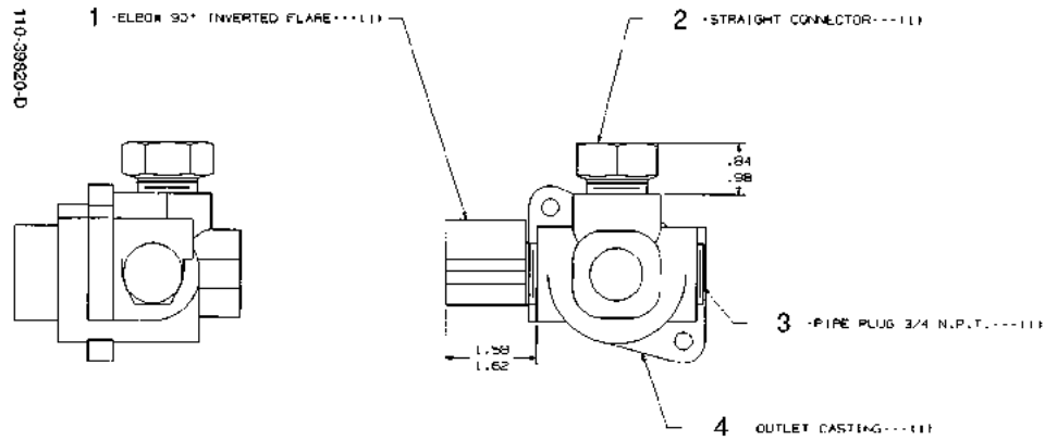
FIGURE 17. 110-39820 - OUTLET CASTING ASSEMBLY
