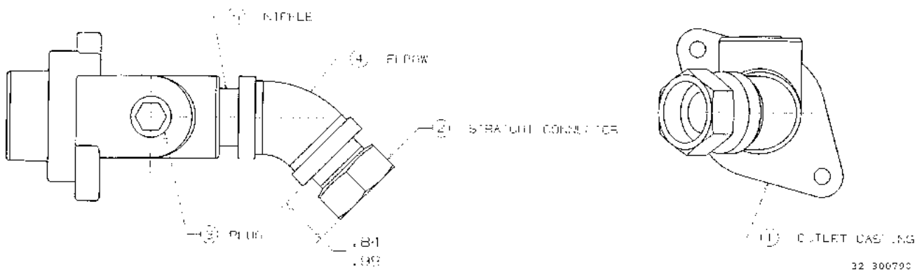
FIGURE 118. 32-300790-DWG - OUTLET & FITTING ASSY
