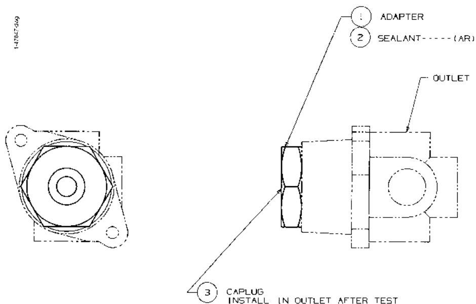
FIGURE 19. 1-47847-DWG - VAPOR READY MODULE
