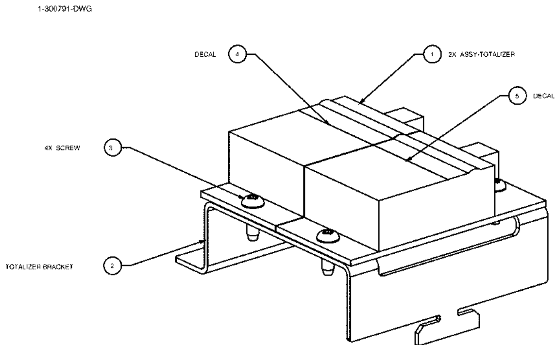
FIGURE 71. 1-300791-DWG - TOTALIZER & BRACKET ASSEMBLY
