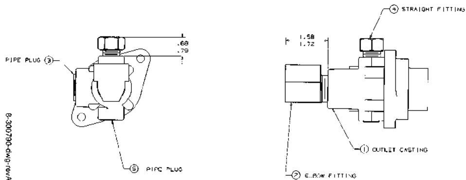
FIGURE 104. 8-300790-DWG - OUTLET & FITTING ASSEMBLY
