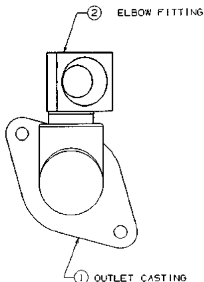
FIGURE 108. 12-300790-DWG - OUTLET & FITTINGS ASSEMBLY
