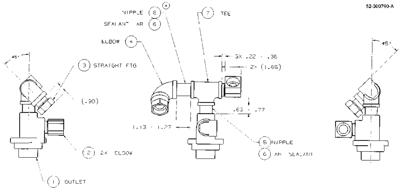
FIGURE 127. 52-300790-DWG - OUTLET & FITTING ASSEMBLY
