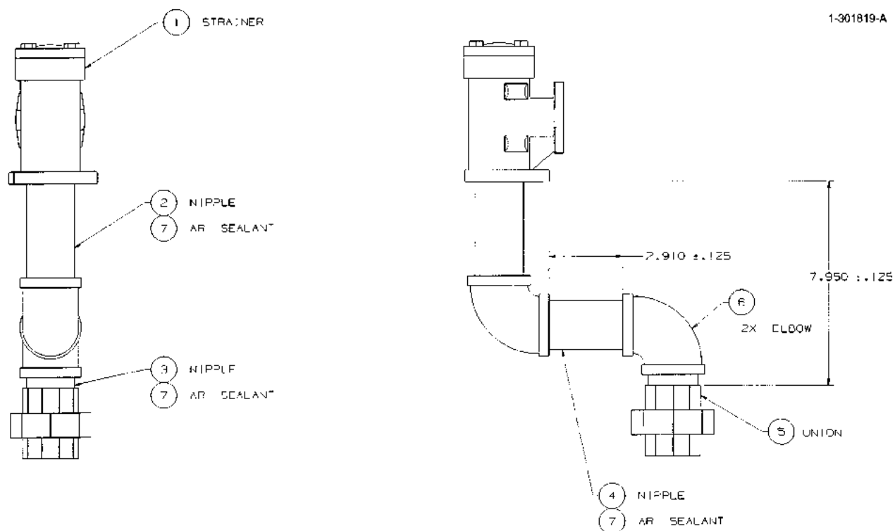
FIGURE 6. 1-301819-DWG - STRAINER ASSEMBLY
