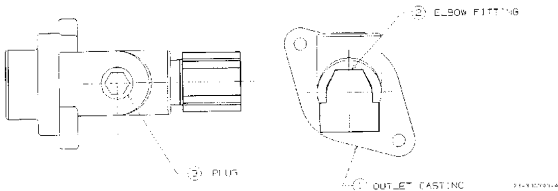
FIGURE 116. 23-300790-DWG - OUTLET & FITTING ASSY
