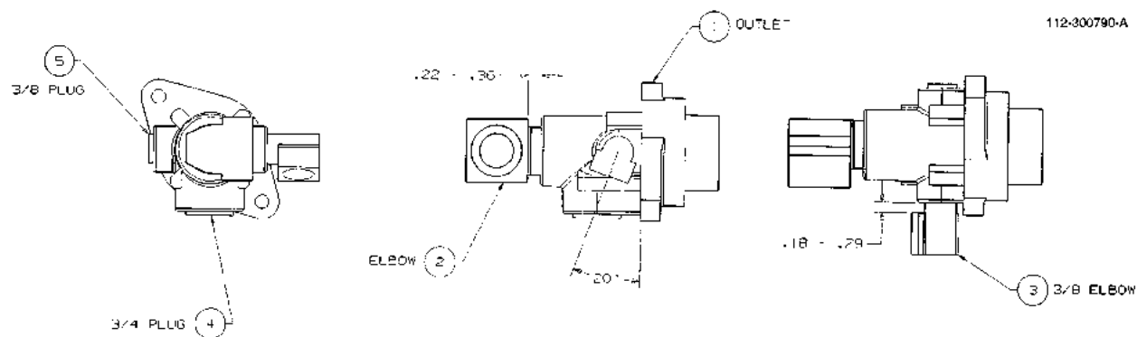
FIGURE 149. 112-300790-DWG - OUTLET WAYNE VAC VAPOR RECOVERY 2/V590
