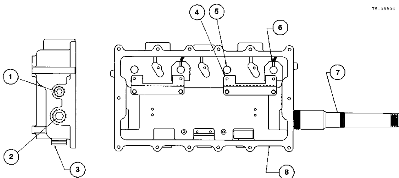
FIGURE 61. 75-39804 - JUNCTION BOX ASSEMBLY
