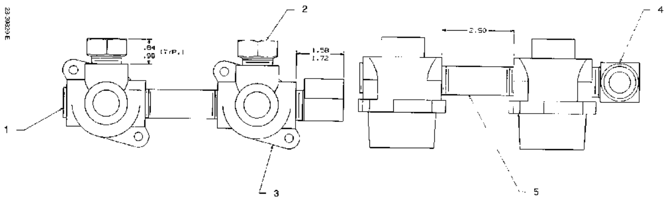
FIGURE 16. 28-39820 - OUTLET CASTING ASSEMBLY
