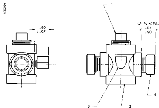
FIGURE 21. 9-300236 - CROSS & INVERTED FLARE ASSEMBLY
