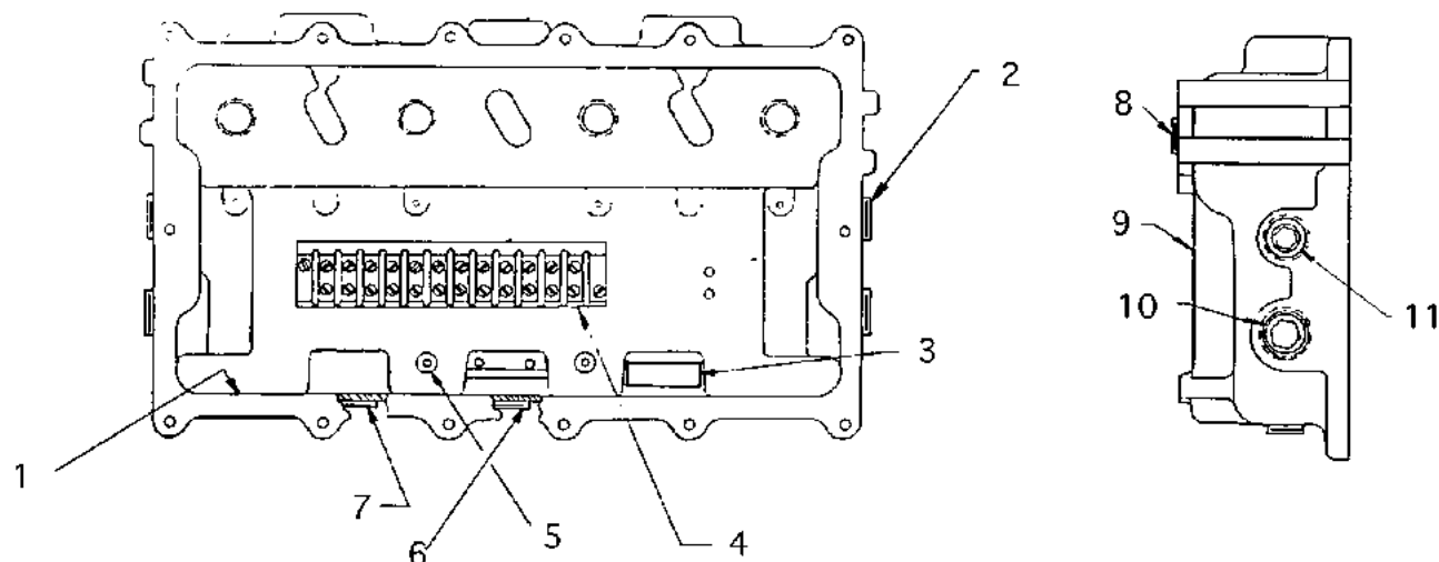
FIGURE 52. 17-39804 - JUNCTION BOX ASSEMBLY
