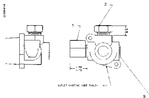
FIGURE 15. 14-39820 - OUTLET CASTING ASSEMBLY
