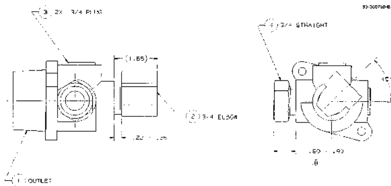
FIGURE 144. 93-300790-DWG - OUTLET & FITTING ASSEMBLY
