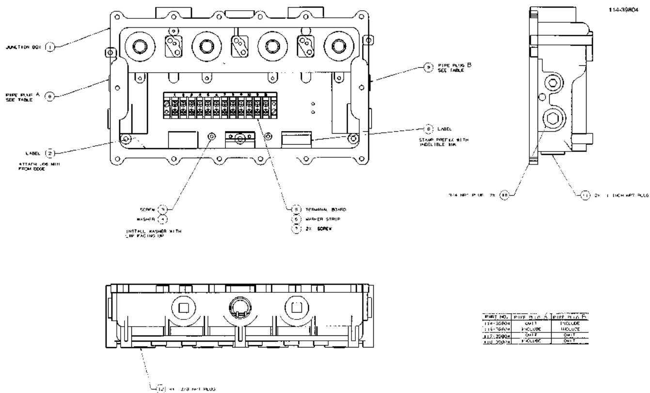
FIGURE 64. 114-39804-DWG - JUNCTION BOX ASSEMBLY
