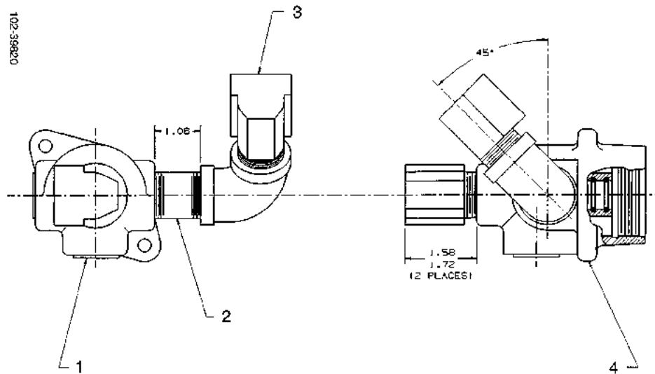
FIGURE 91. 102 &amp; 103-39820 - OUTLET CASTING ASSEMBLY
