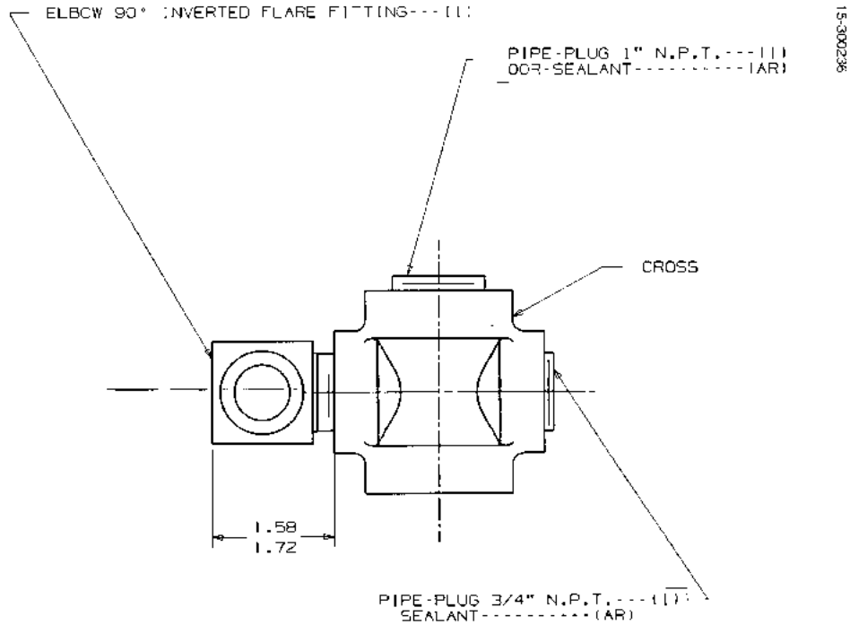
FIGURE 23. 15-300236 - CROSS & INVERTED FLARE FITTING ASSEMBLY
