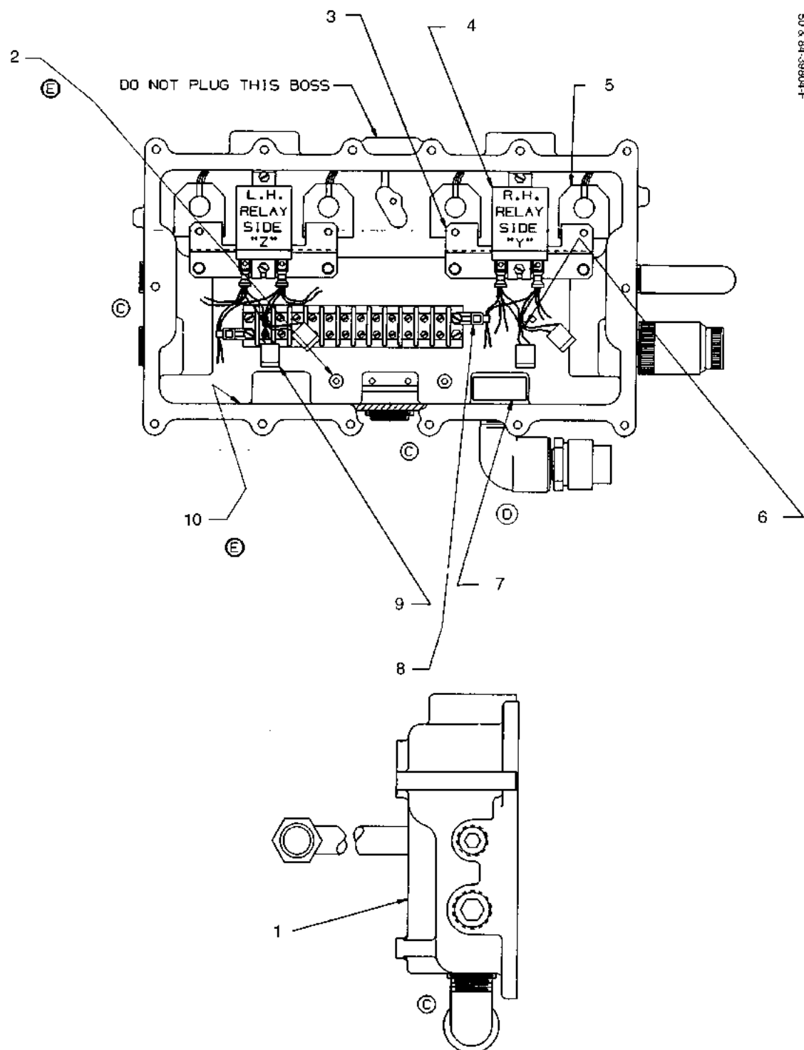
FIGURE 54. 50 & 84-39804 - JUNCTION BOX ASSEMBLY
