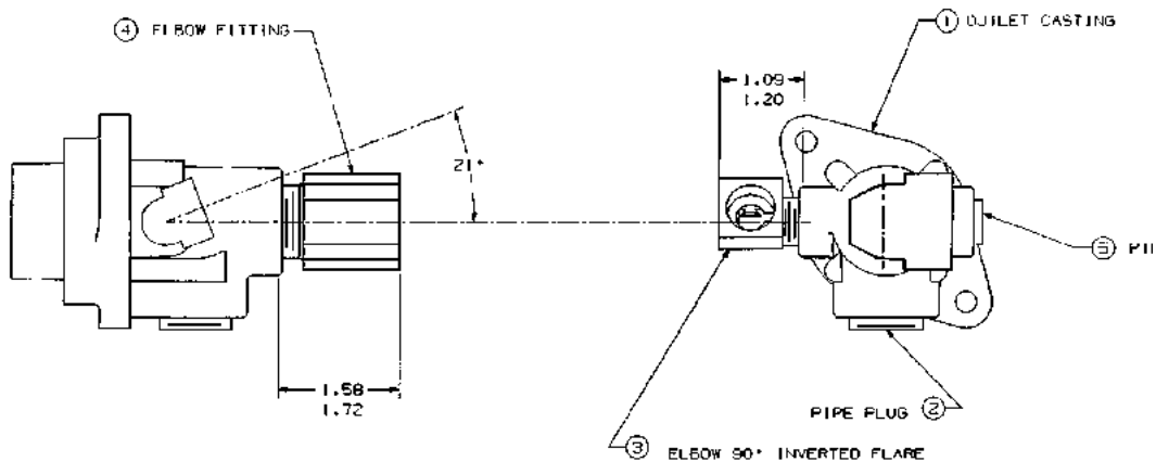
FIGURE 110. 15-300790-DWG - OUTLET &amp; FITTINGS ASSEMBLY
