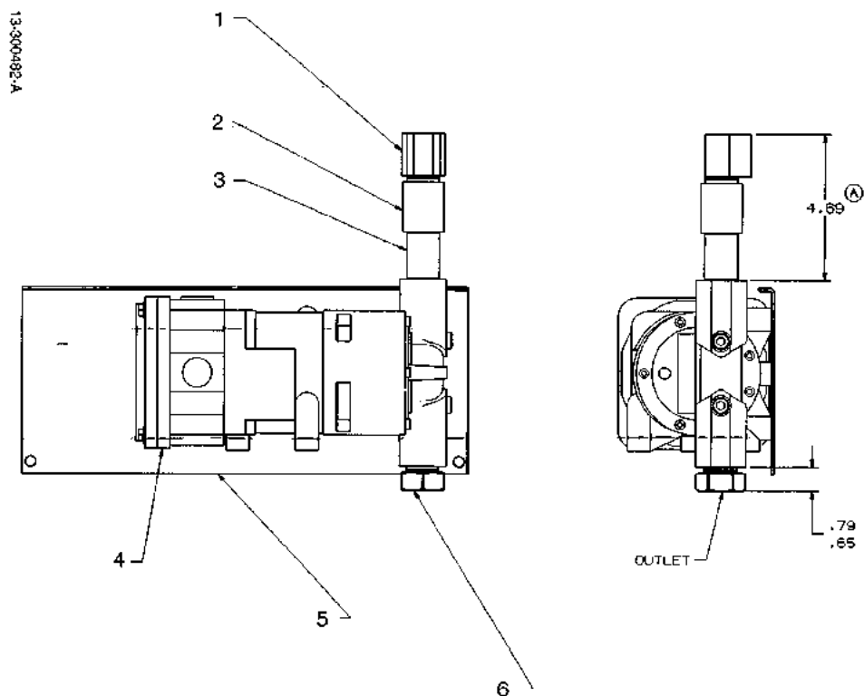
FIGURE 28. 13-300482 PUMP/MOTOR & BRACKET ASSEMBLY
