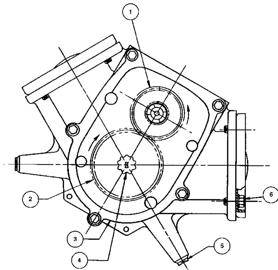
FIGURE 1. 23-39310 - METER ASSEMBLY 2PM-6K
