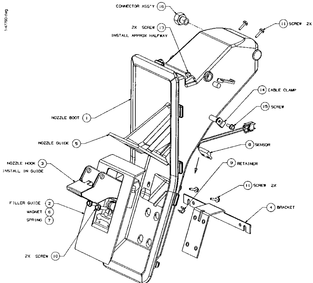
FIGURE 43. 1-47790-DWG - NOZZLE BOOT ASSEMBLY LIFT TO START
