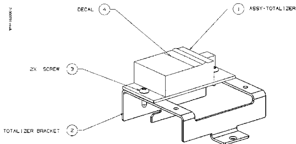
FIGURE 72. 2-300791-DWG - TOTALIZER & BRACKET ASSEMBLY
