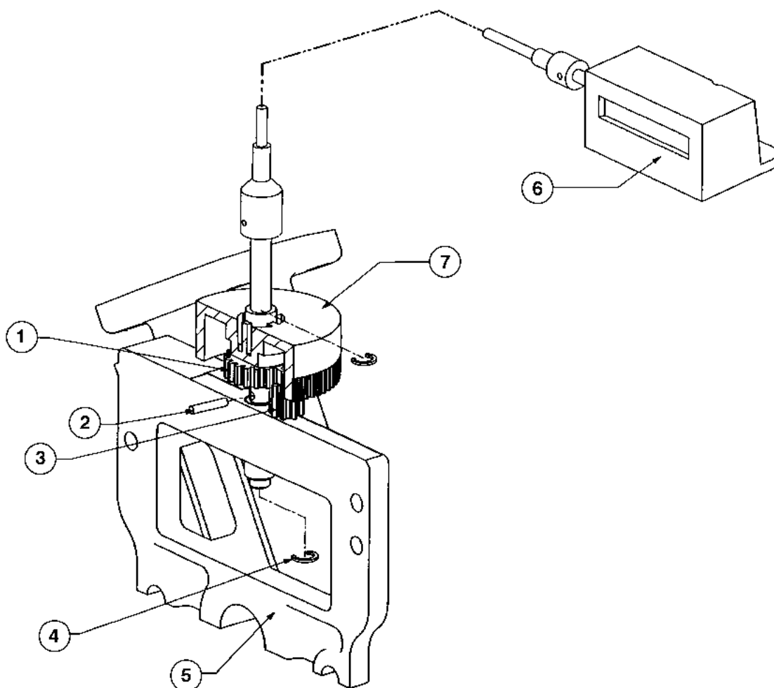
FIGURE 8. 39786 - METER SUPPORT & TOTALIZER GEAR DRIVE ASSEMBLY
