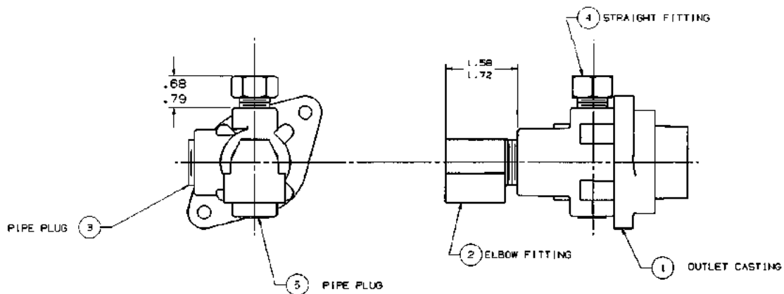
FIGURE 103. 7-300790-DWG - OUTLET & FITTINGS ASSEMBLY
