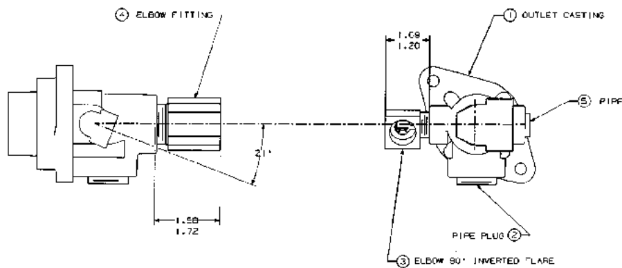
FIGURE 111. 16-300790-DWG - OUTLET & FITTING ASSEMBLY
