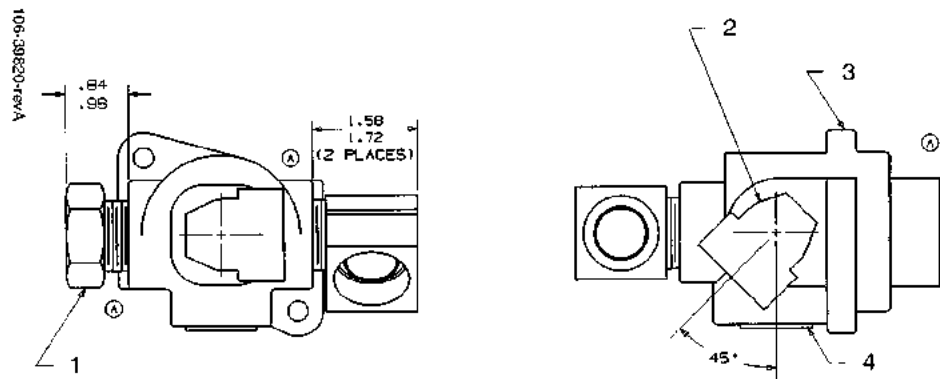
FIGURE 93. 106-39820 - OUTLET CASTING ASSEMBLY
