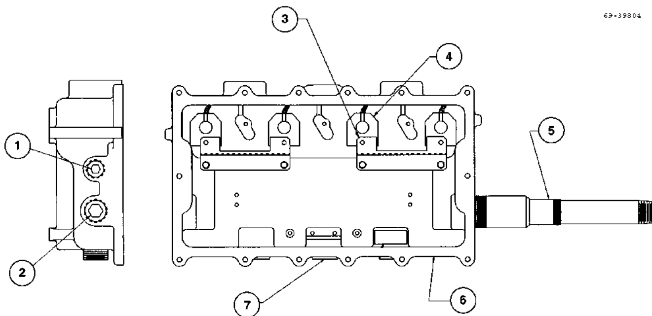
FIGURE 59. 69-39804 - JUNCTION BOX ASSEMBLY
