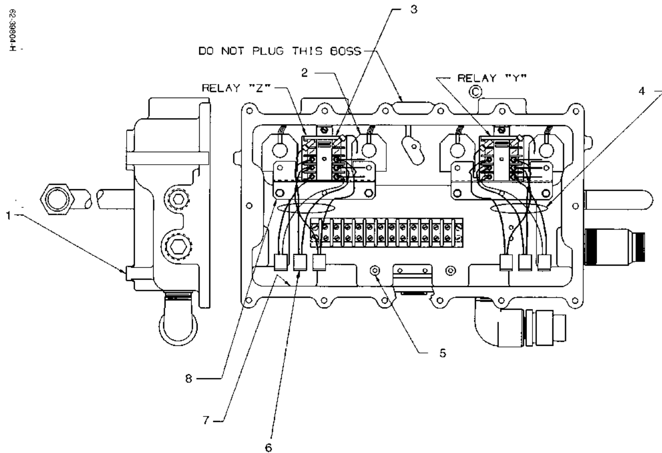
FIGURE 57. 62-39804 - JUNCTION BOX ASSEMBLY
