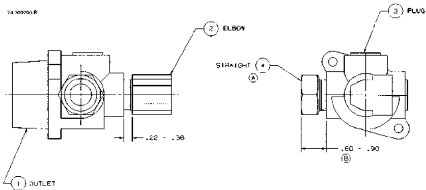
FIGURE 139. 74-300790-DWG - OUTLET BALANCE VAPOR RECOVERY 2/V387
