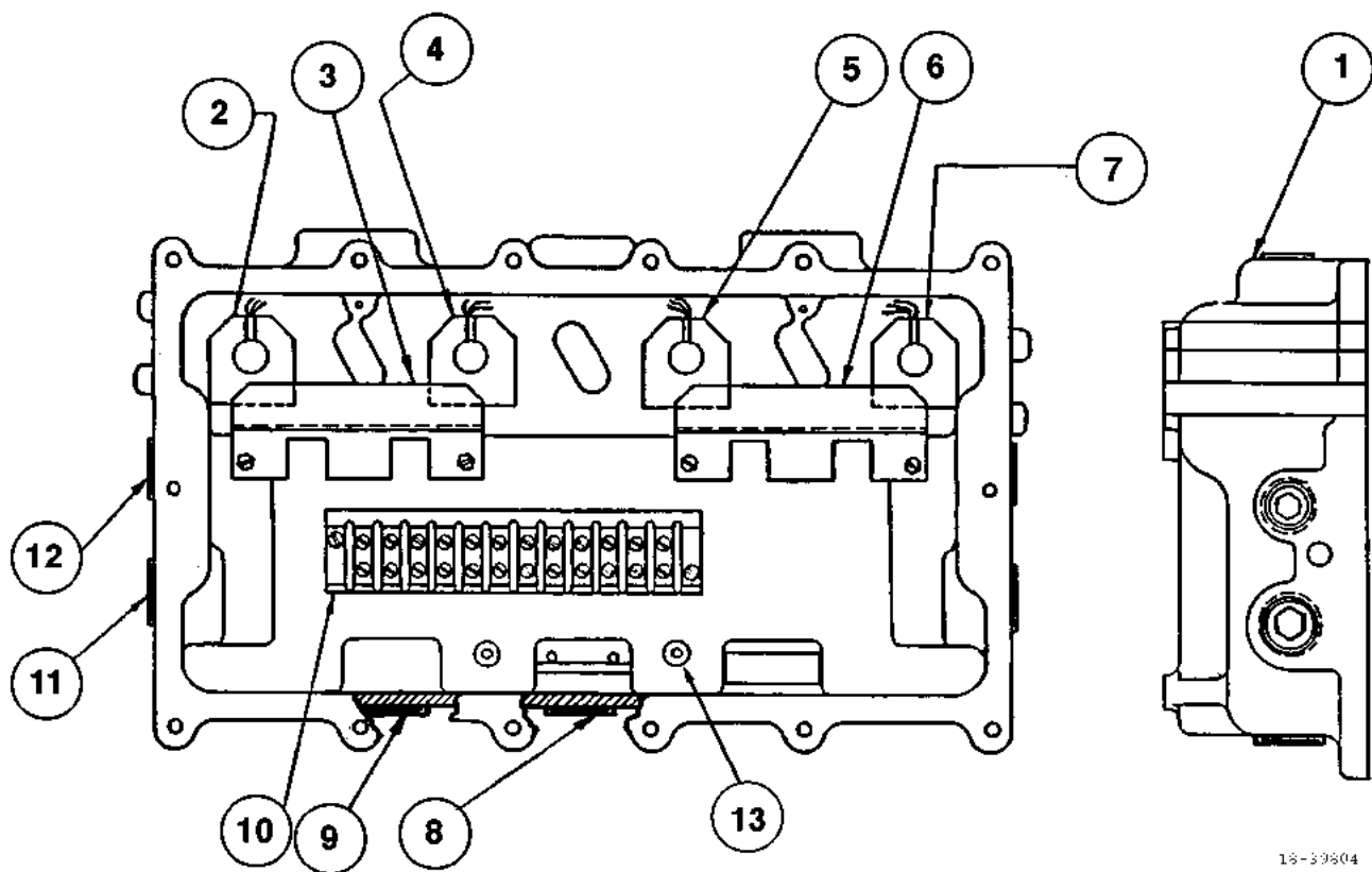
FIGURE 53. 18-39804 - JUNCTION BOX ASSEMBLY
