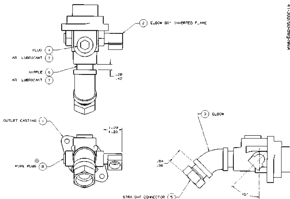
FIGURE 124. 41-300790-DWG - OUTLET & FITTING ASSEMBLY
