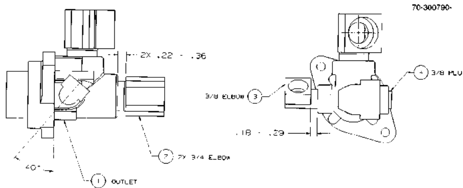
FIGURE 137. 70-300790-DWG - OUTLET WAYNE VAC VAPOR RECOVERY 2/V590/U
