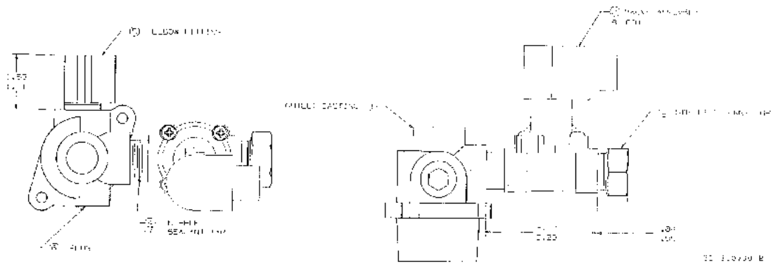
FIGURE 117. 31-300790-DWG - OUTLET & VALVE ASSY
