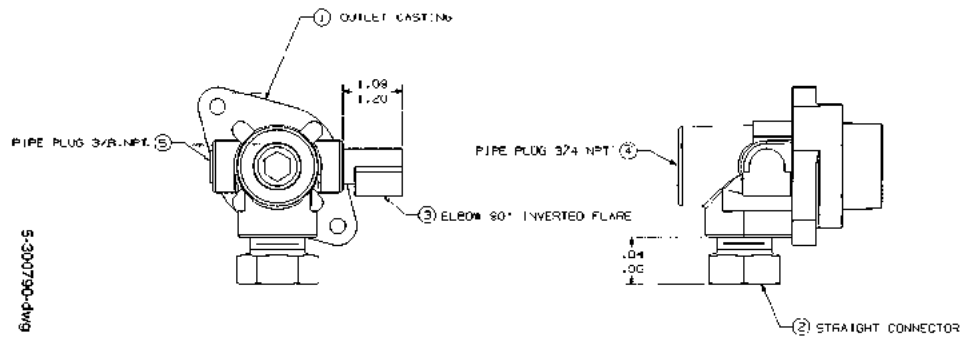
FIGURE 25. 5-300790-DWG - OUTLET AND FITTING ASSEMBLY
