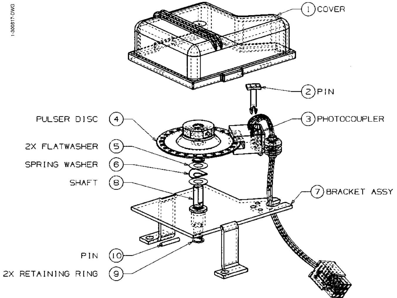
FIGURE 14. 1-300817-DWG - PULSER ASSEMBLY
