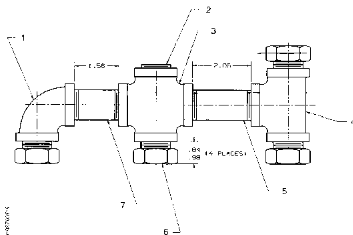
FIGURE 101. 5-300236 - CROSS &amp; INVERTED FLARE FITTINGS ASSEMBLY
