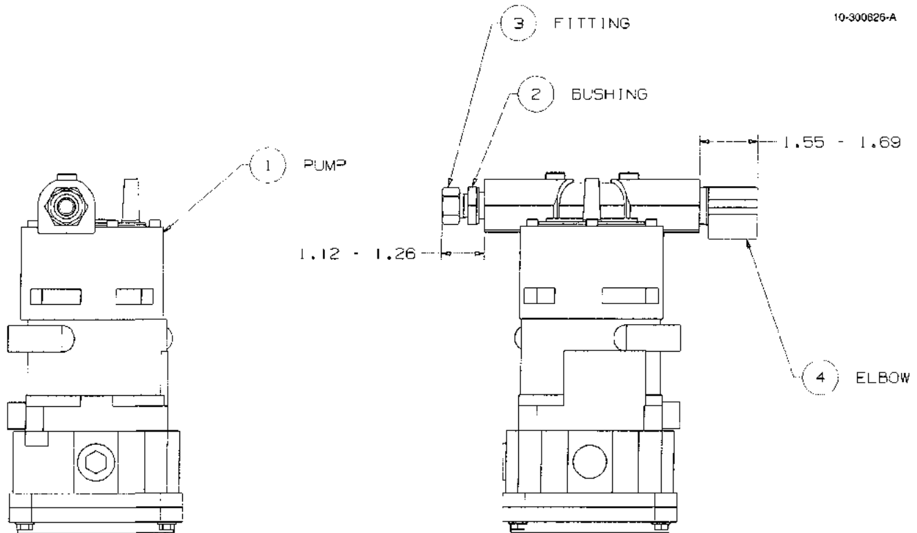
FIGURE 37. 10-300826-DWG - RIGHT VACUUM PUMP SUCTION
