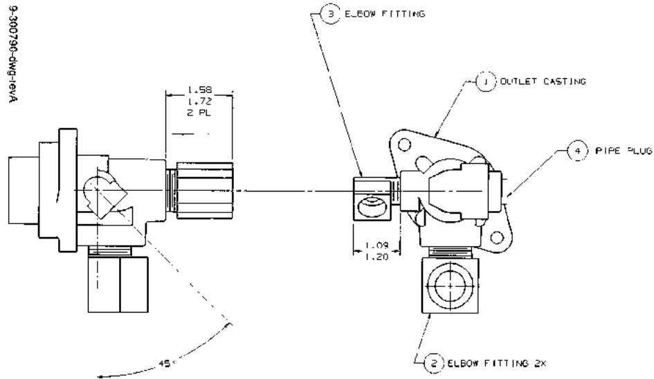
FIGURE 105. 9-300790-DWG - FITTINGS & OUTLET ASSEMBLY
