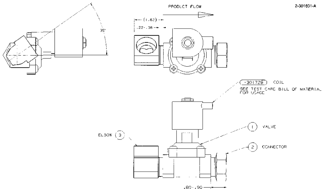
FIGURE 151. 2-301831-DWG - VALVE & FITTINGS
