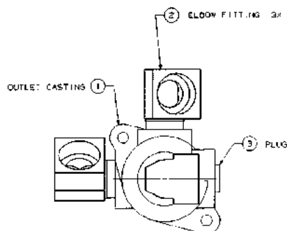
FIGURE 107. 11-300790-DWG - OUTLET & FITTINGS ASSEMBLY
