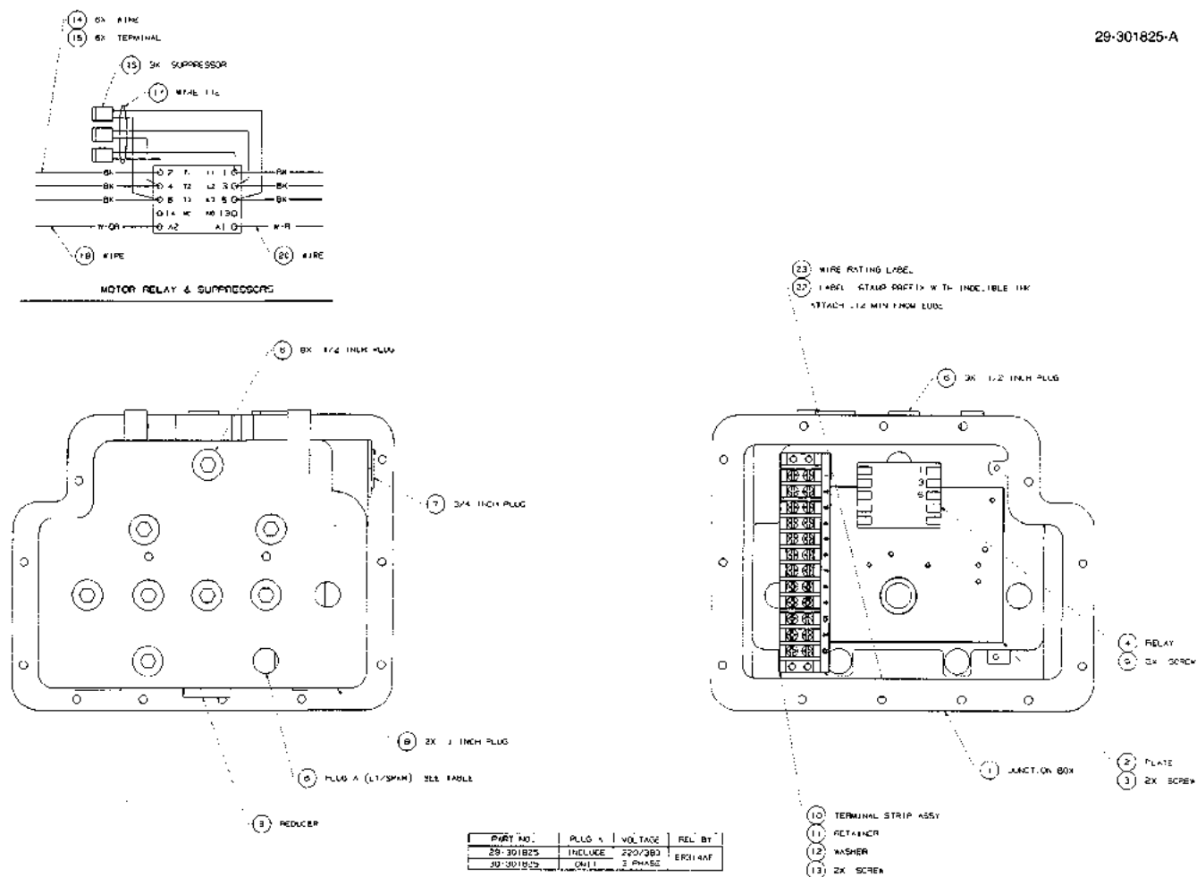
FIGURE 70. 29-301825-DWG - JUNCTION BOX ASSY ONE PRODUCT 3 PHASE
