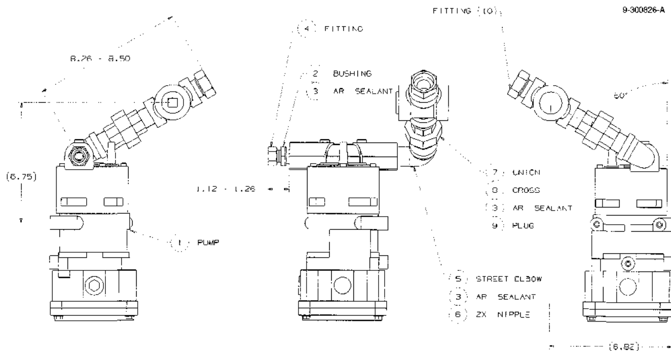
FIGURE 36. 9-300826-DWG - LEFT VACUUM PUMP SUCTION
