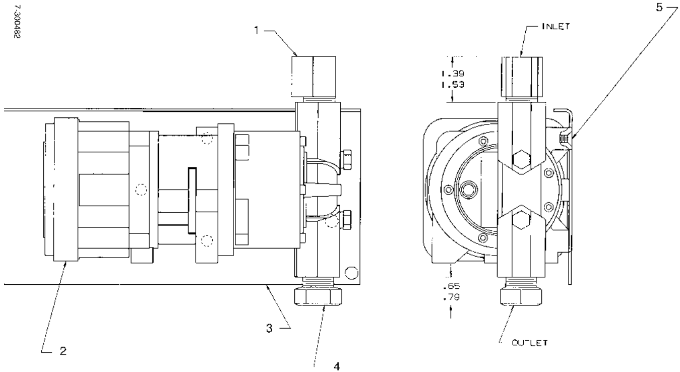
FIGURE 27. 7-300482 - PUMP/MOTOR & BRACKET ASSEMBLY
