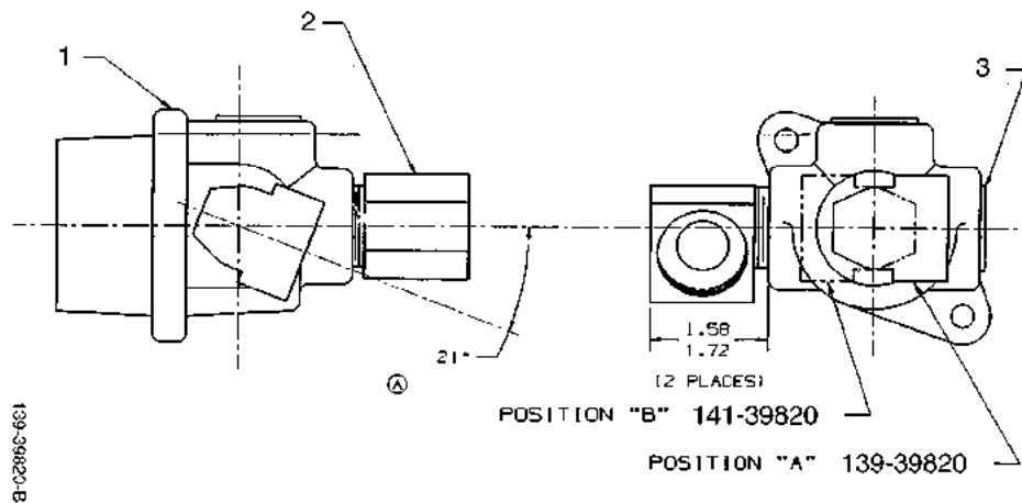
FIGURE 96. 139 & 141-39820 - OUTLET CASTING ASSEMBLY
