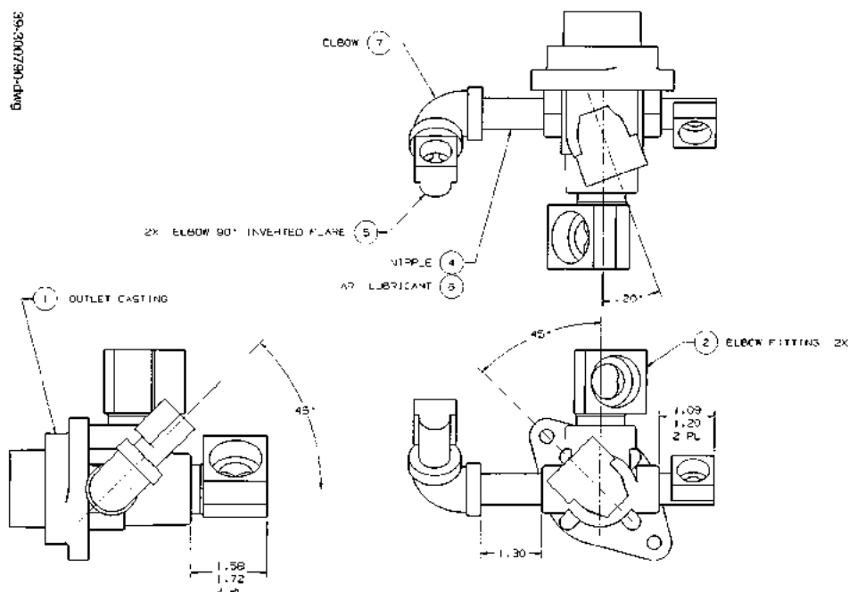
FIGURE 122. 39-300790-DWG - OUTLET & FITTINGS ASSEMBLY
