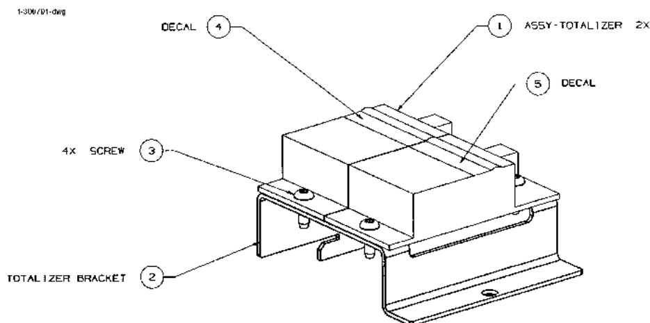
FIGURE 73. 4-300791-DWG - TOTALIZER & BRACKET ASSEMBLY
