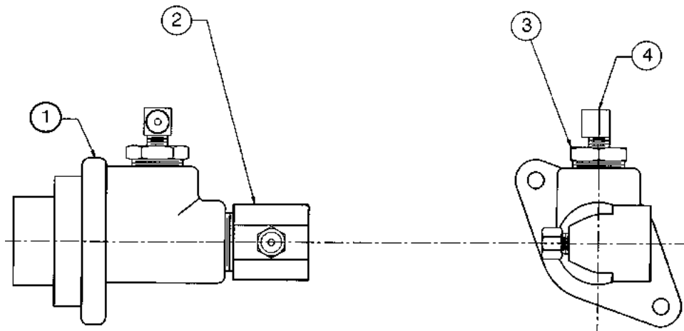
FIGURE 98. 168-39820-DWG - OUTLET CASTING ASSEMBLY
