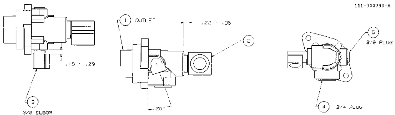
FIGURE 148. 111-300790-DWG - OUTLET WAYNE VAC VAPOR RECOVERY 2/V590, 2/V591
