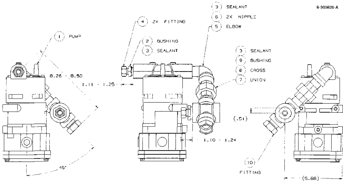
FIGURE 35. 8-300826-DWG - LOWER VACUUM PUMP SUCTION
