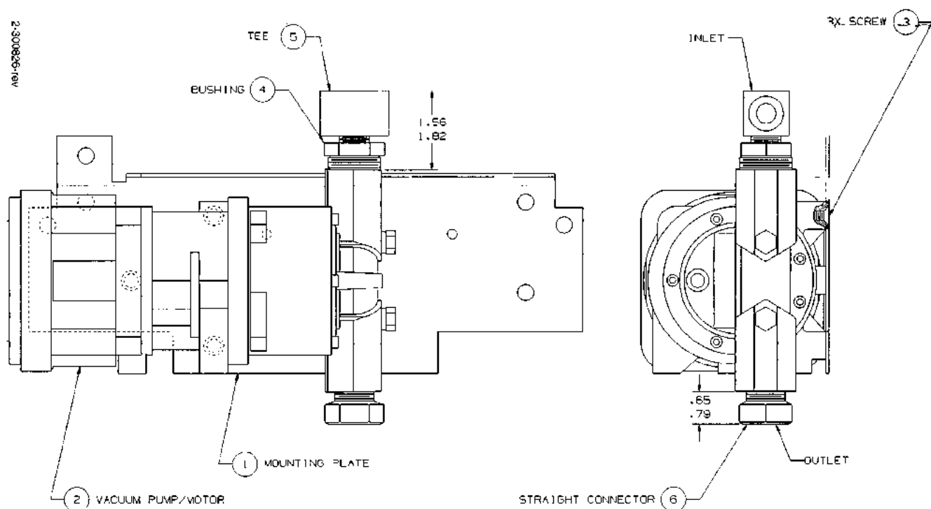
FIGURE 30. 2-300826-DWG - PUMP/MOTOR AND BRACKET ASSEMBLY
