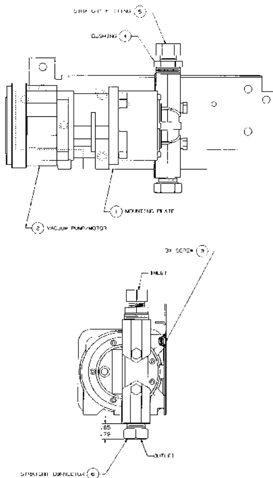
FIGURE 29. 1-300826-DWG - PUMP/MOTOR AND BRACKET ASSEMBLY
