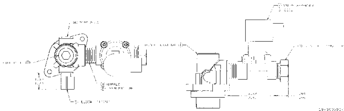
FIGURE 113. 19-300790-DWG - OUTLET & VALVE ASSY
