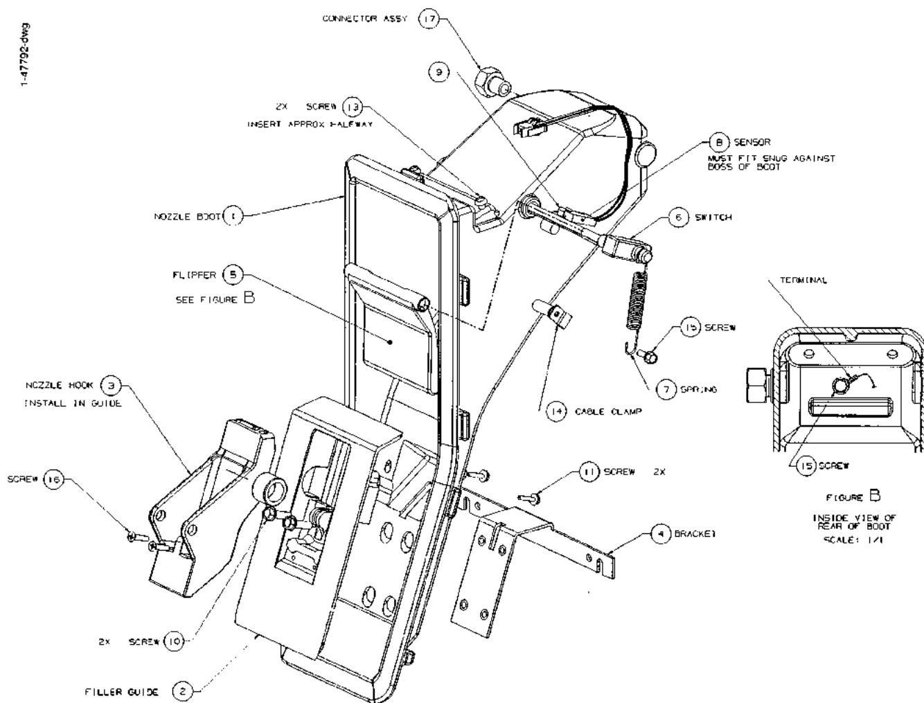
FIGURE 44. 1-47792-DWG - NOZZLE BOOT ASSEMBLY PUSH TO START
