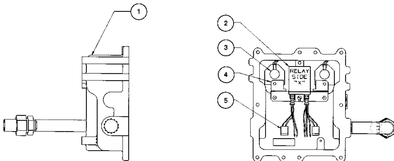
FIGURE 65. 5-300116 - JUNCTION BOX ASSEMBLY
