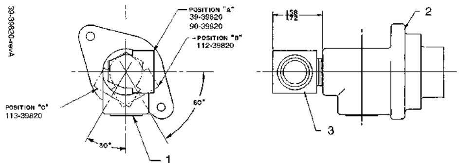
FIGURE 90. 39 & 90-39820 - OUTLET CASTING ASSEMBLY
