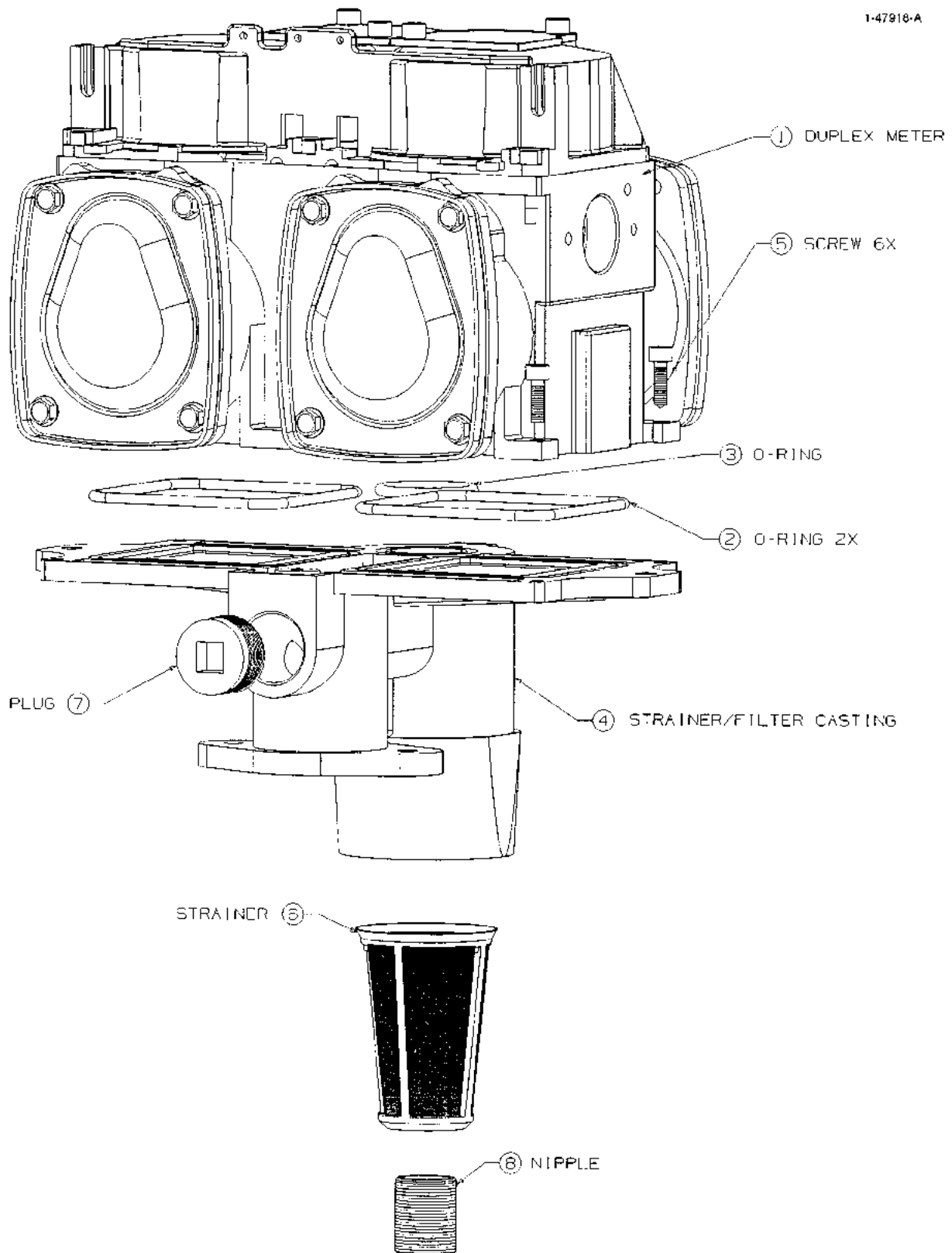
FIGURE 3. 1-47918-DWG - IMETER MODULE REMOTE SINGLE SIDED
