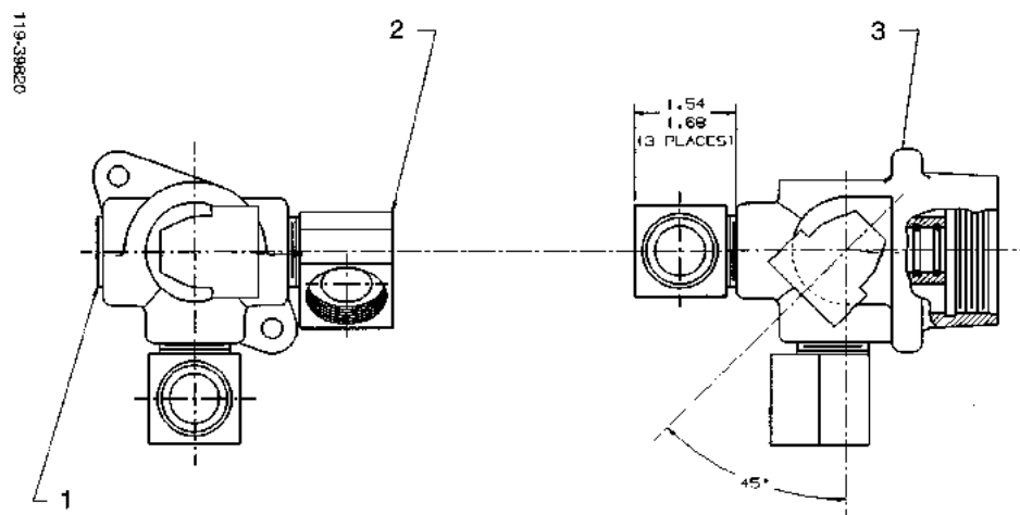
FIGURE 95. 119-39820 - OUTLET CASTING ASSEMBLY
