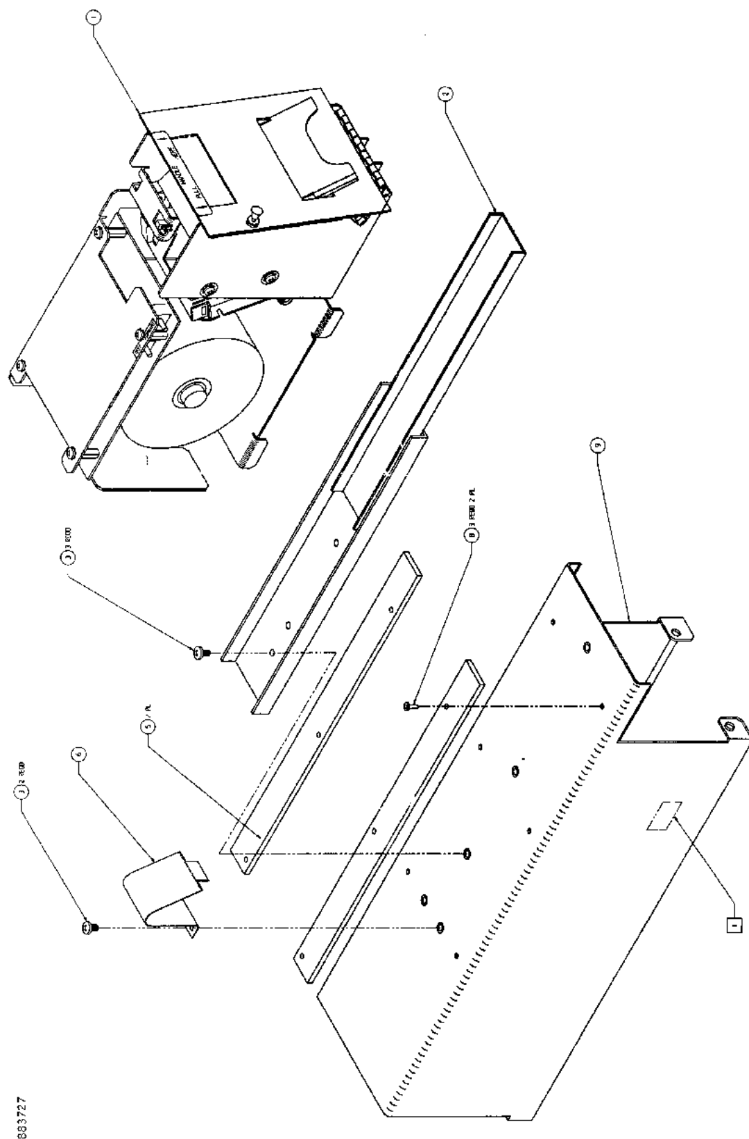
FIGURE 82. 883727 - TEARBAR PRINTER ASSEMBLY
