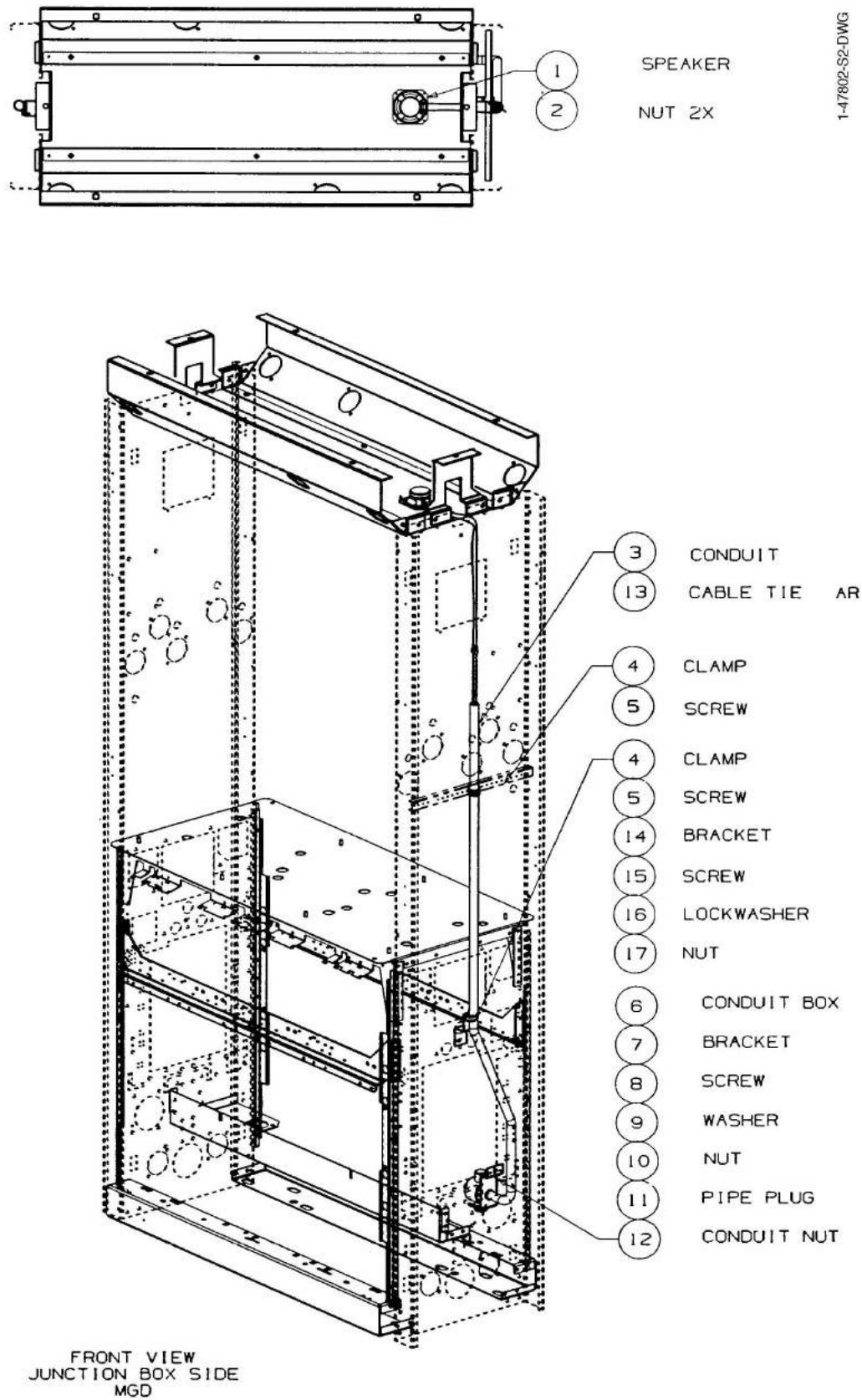
FIGURE 38. 1-47802-S2-DWG - SPEAKER MODULE
