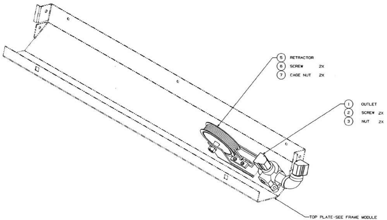
FIGURE 92. 37-47816-DWG - TOP MODULE V390/QU/HIGH HOSE W/RETRACTOR
