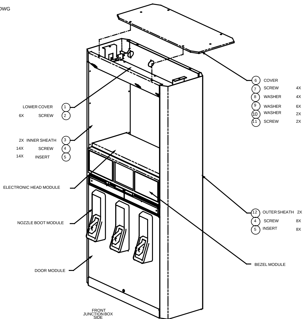
FIGURE 2. 1-47809-DWG - WIDE HOUSING MODULE
