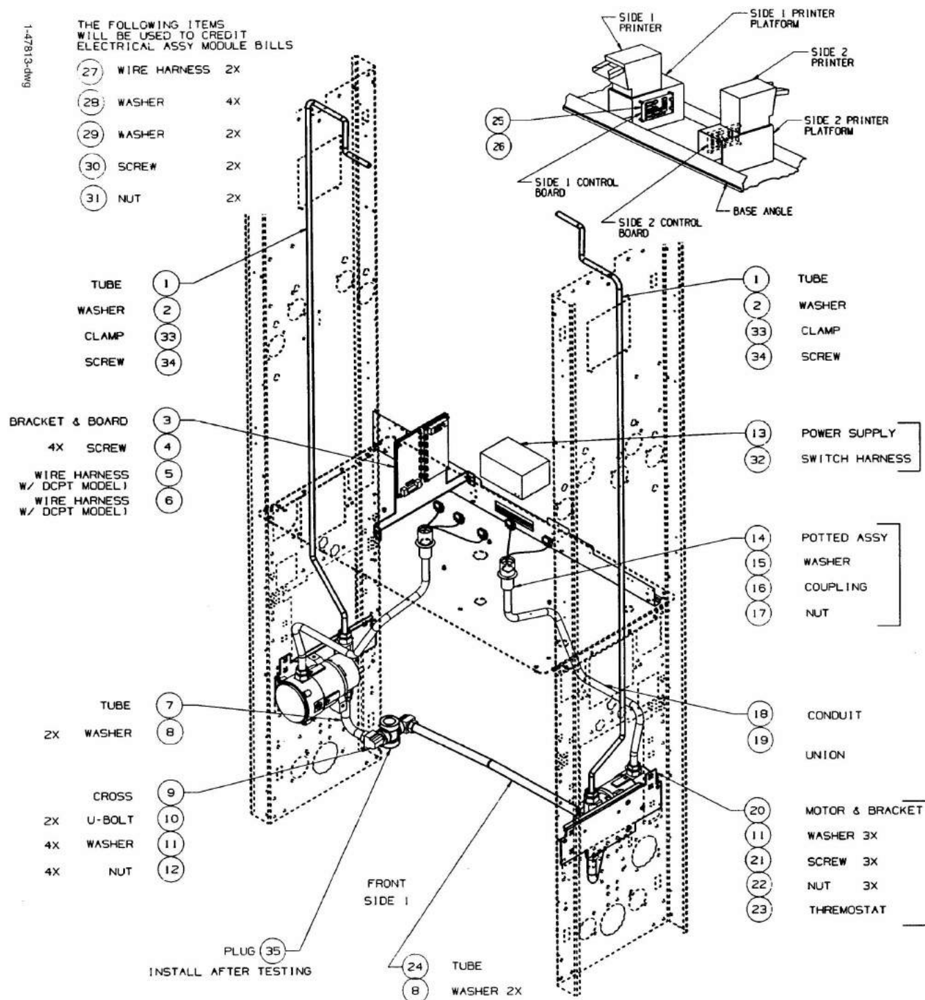
FIGURE 25. 1-47813-DWG - VAPOR RECOVERY MODULE V390
