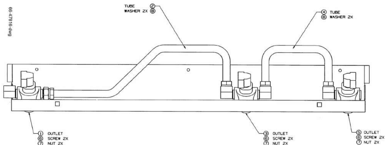
FIGURE 95. 66-47816-DWG - TOP MODULE 1/V390P/D2
