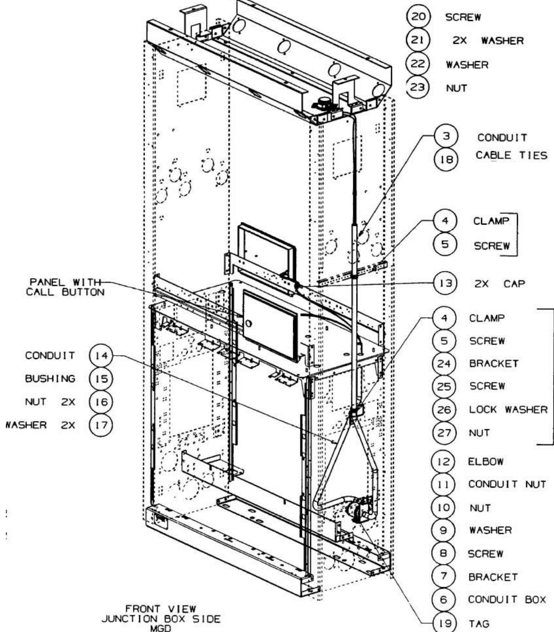
FIGURE 40. 3-47802-S2-DWG - SPEAKER MODULE WITH CALL BUTTON
