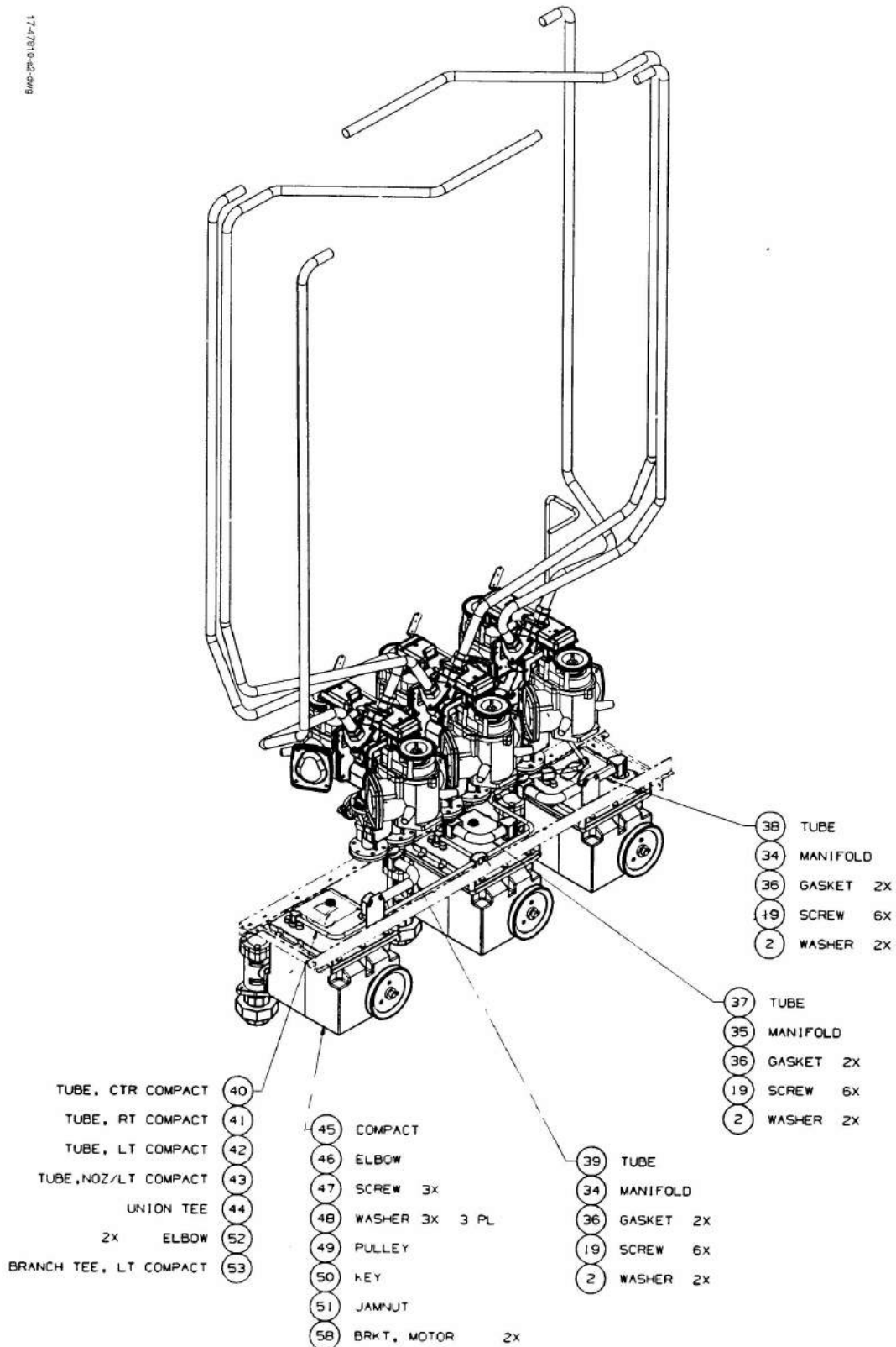
FIGURE 17. 17-47810-S2-DWG - HYDRAULICS MODULE V390P
