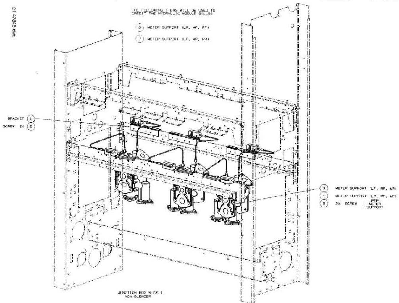
FIGURE 20. 21-47818-DWG - MECHANICAL TOTALIZER MODULE V390D/K/ TOTALIZER NEXT TO NOZZLE BOOT
