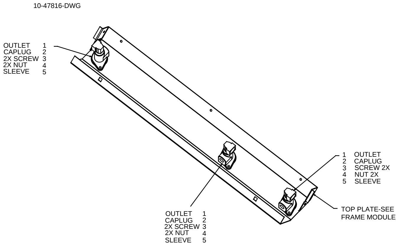
FIGURE 91. 10-47816-DWG - TOP ASSEMBLY MODULE
