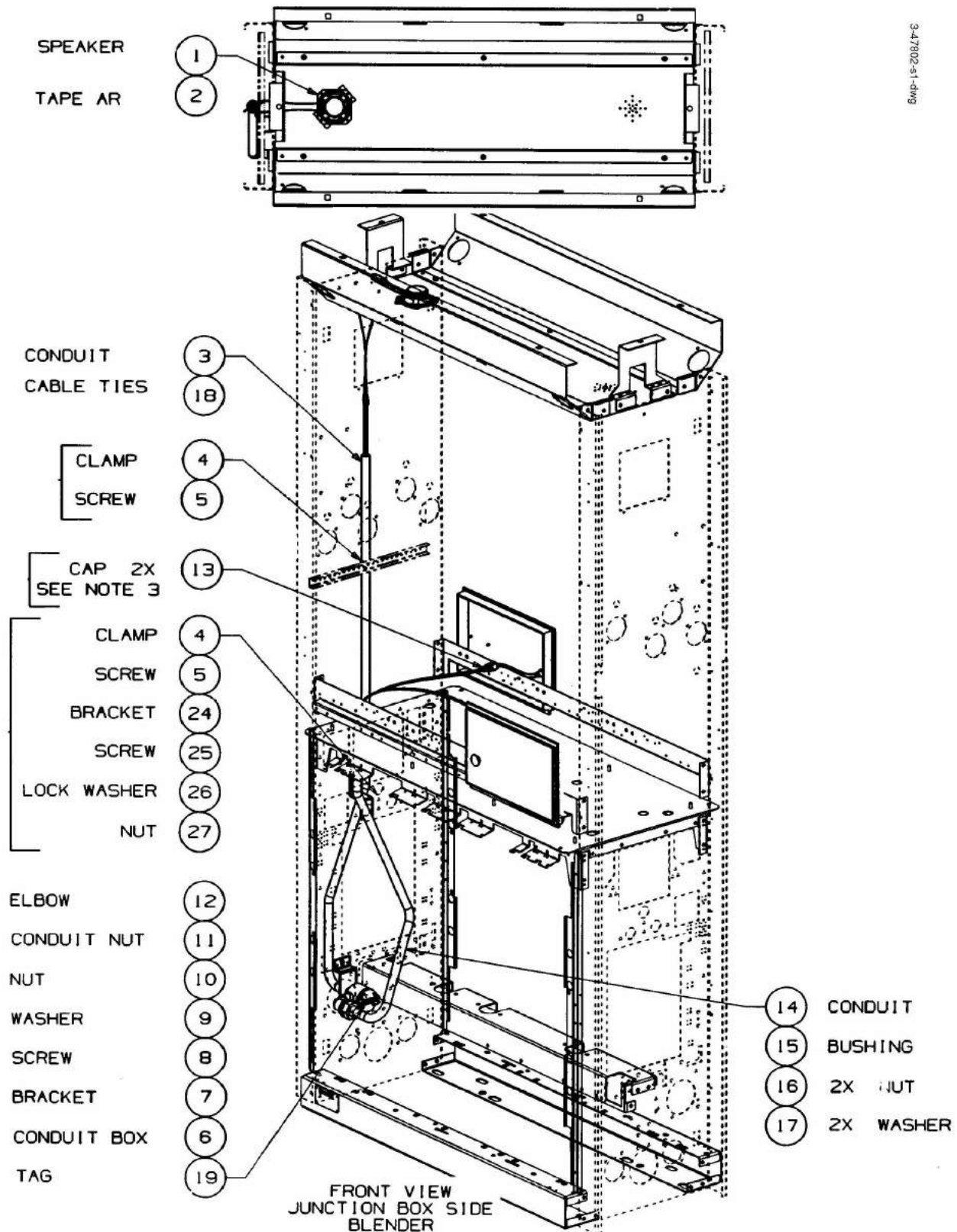
FIGURE 39. 3-47802-S1-DWG - SPEAKER MODULE WITH CALL BUTTON
