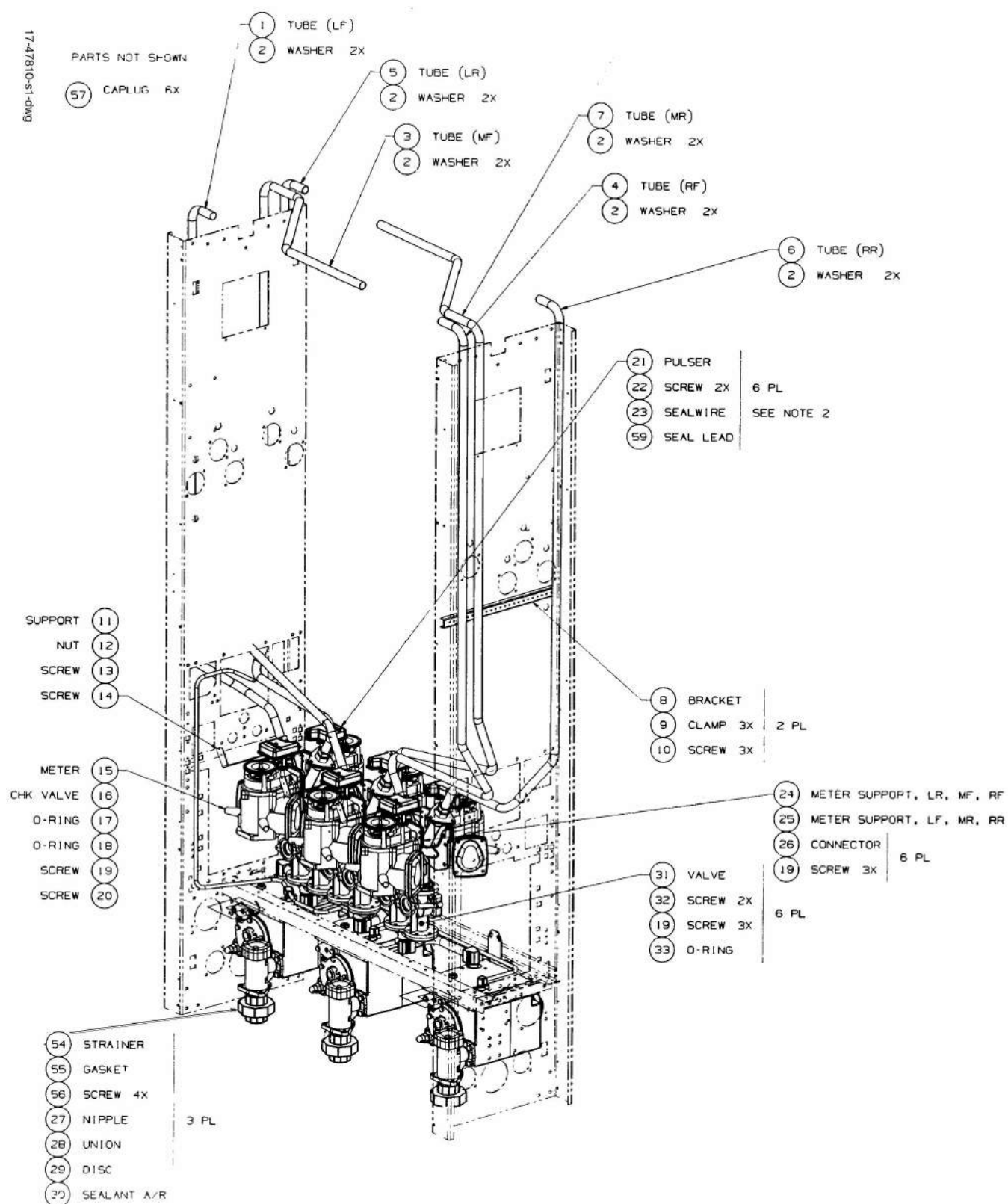
FIGURE 16. 17-47810-S1-DWG - HYDRAULICS MODULE V390P
