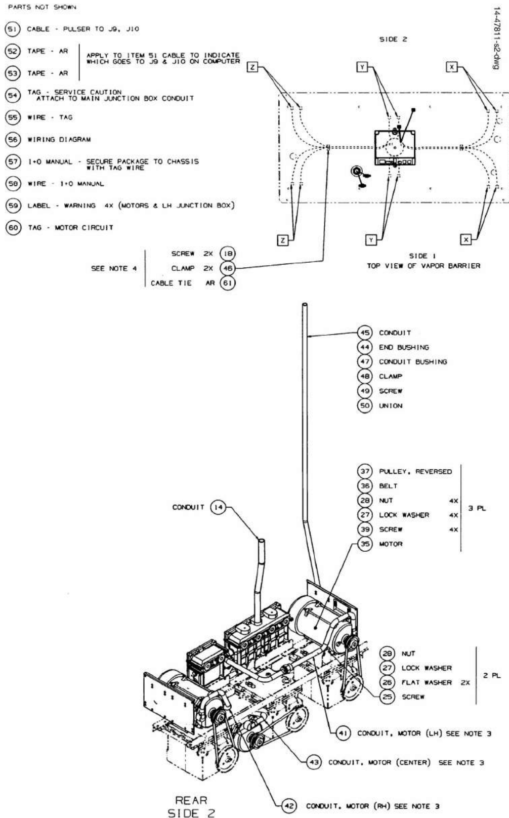
FIGURE 36. 14-47811-S2-DWG - ELECTRICAL MODULE
