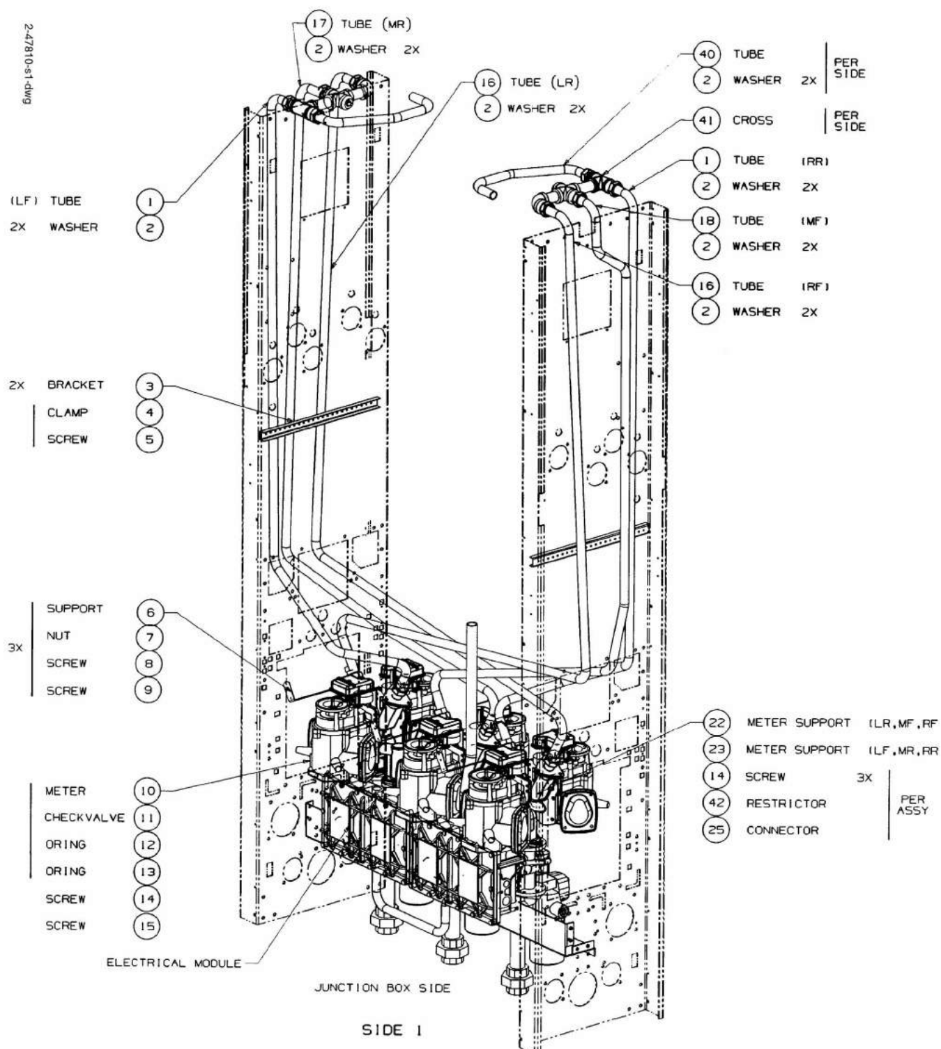
FIGURE 8. 2-47810-S1-DWG - HYDRAULICS MODULE V390D/GU
