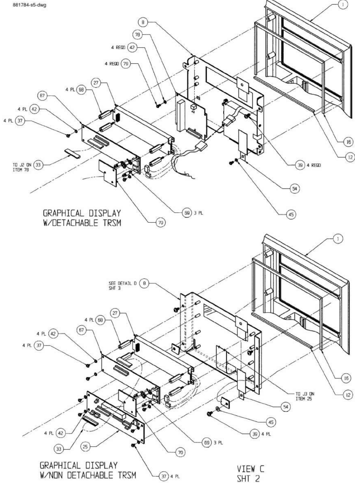
FIGURE 58. 881784-S5 - CUSTOMER PAYMENT MODULE
