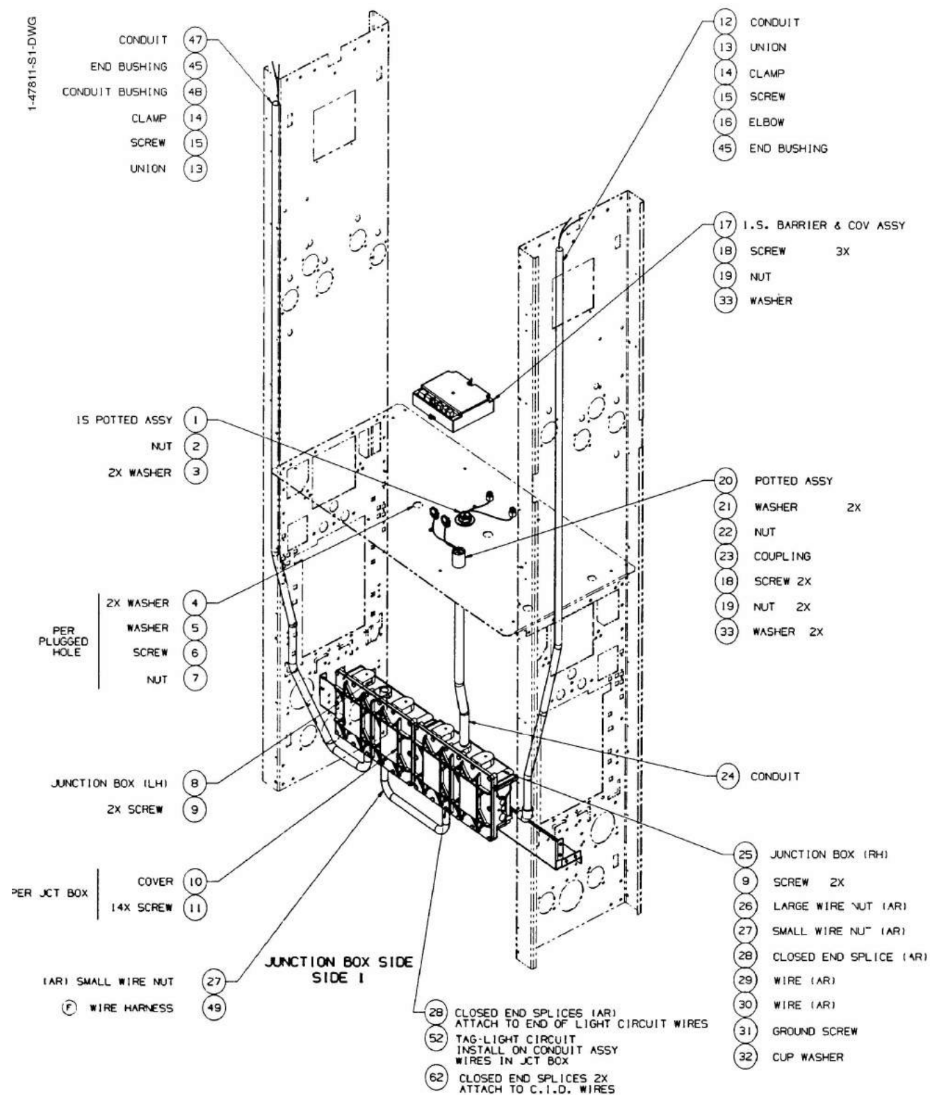
FIGURE 33. 1-47811-S1-DWG - ELECTRICAL MODULE V390D/G
