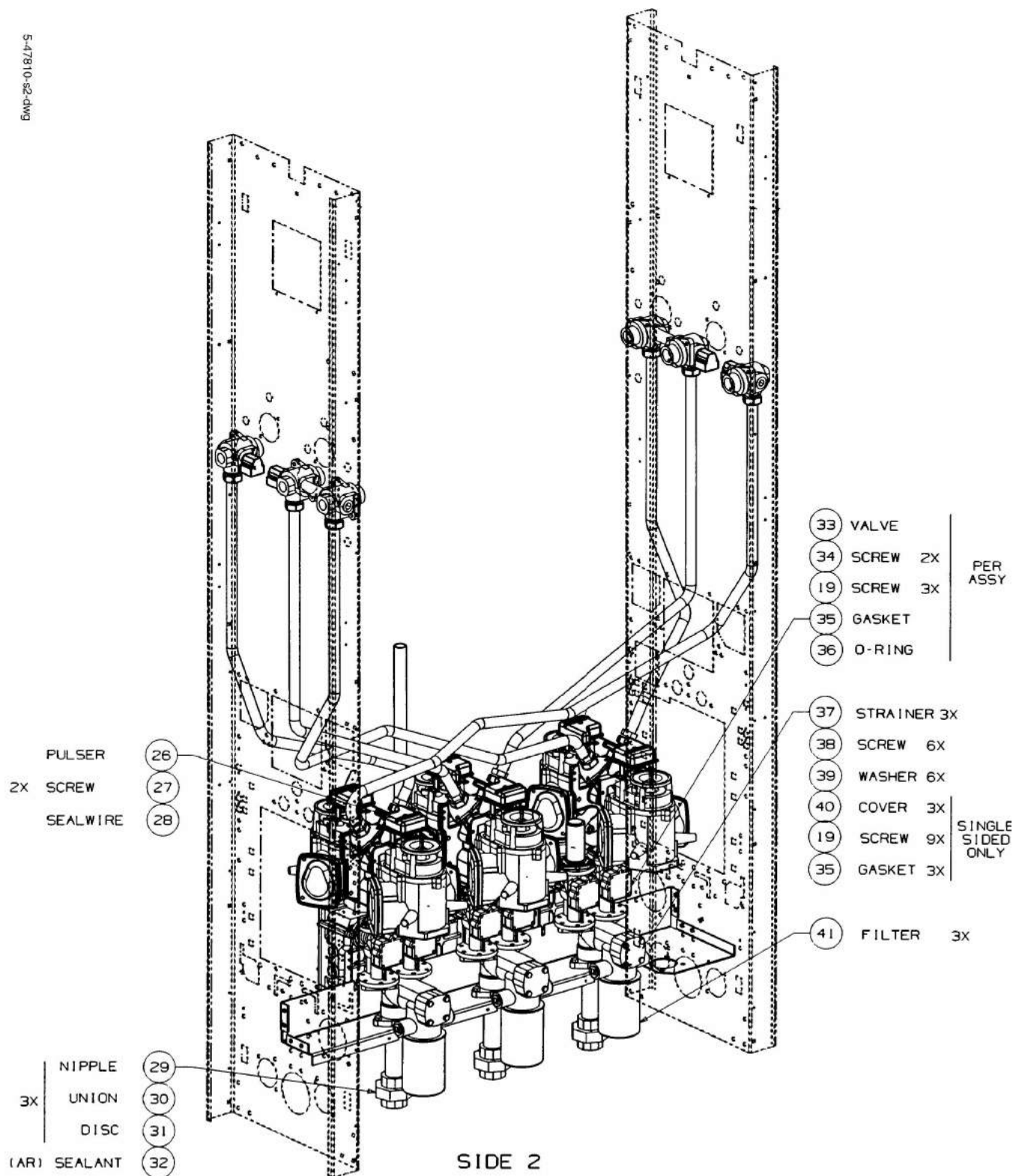
FIGURE 15. 5-47810-S2-DWG - HYDRAULICS MODULE X1/V390D/V
