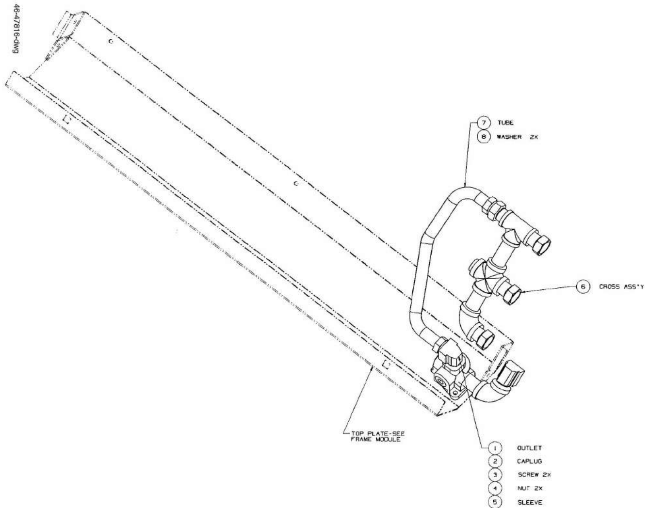
FIGURE 94. 46-47816-DWG - TOP MODULE 1/V390P/QU FRONT
