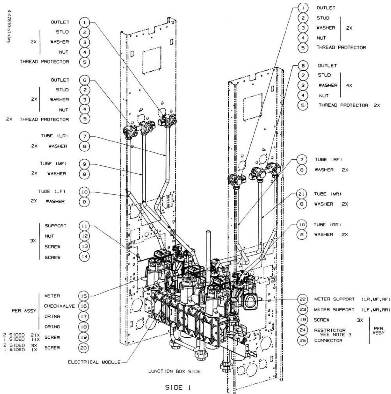
FIGURE 12. 4-47810-S1-DWG- - HYDRAULICS MODULE V390D/V
