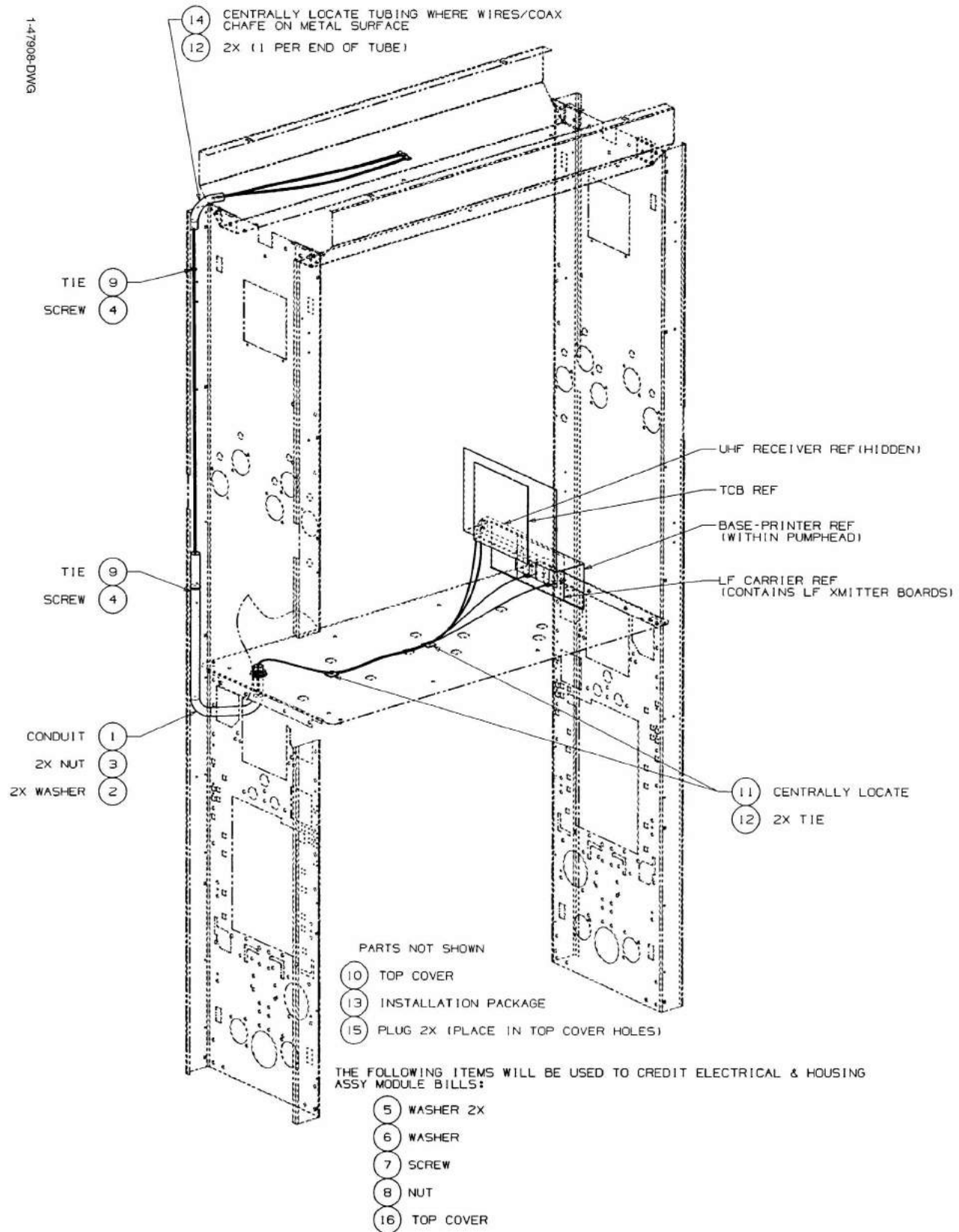
FIGURE 48. 1-47908-DWG - WAYNE TRAC MODULE WIDE
