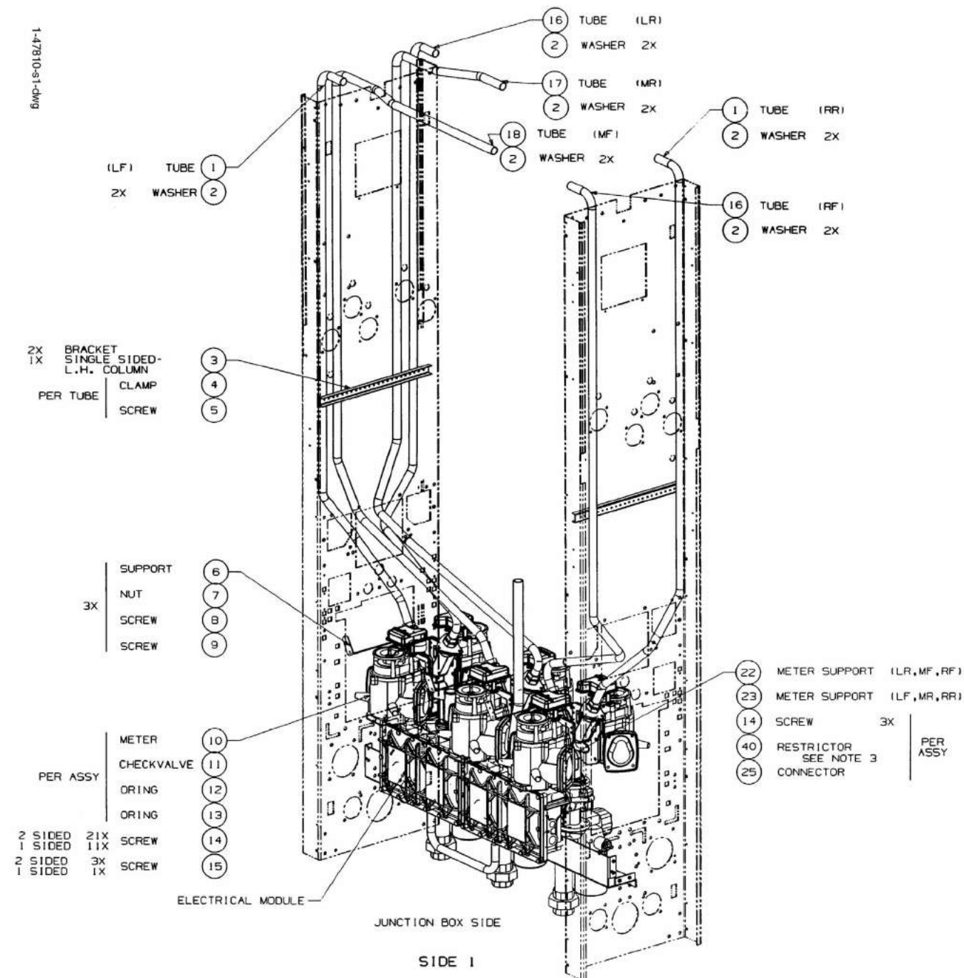
FIGURE 6. 1-47810-S1-DWG - HYDRAULICS MODULE V390D/G
