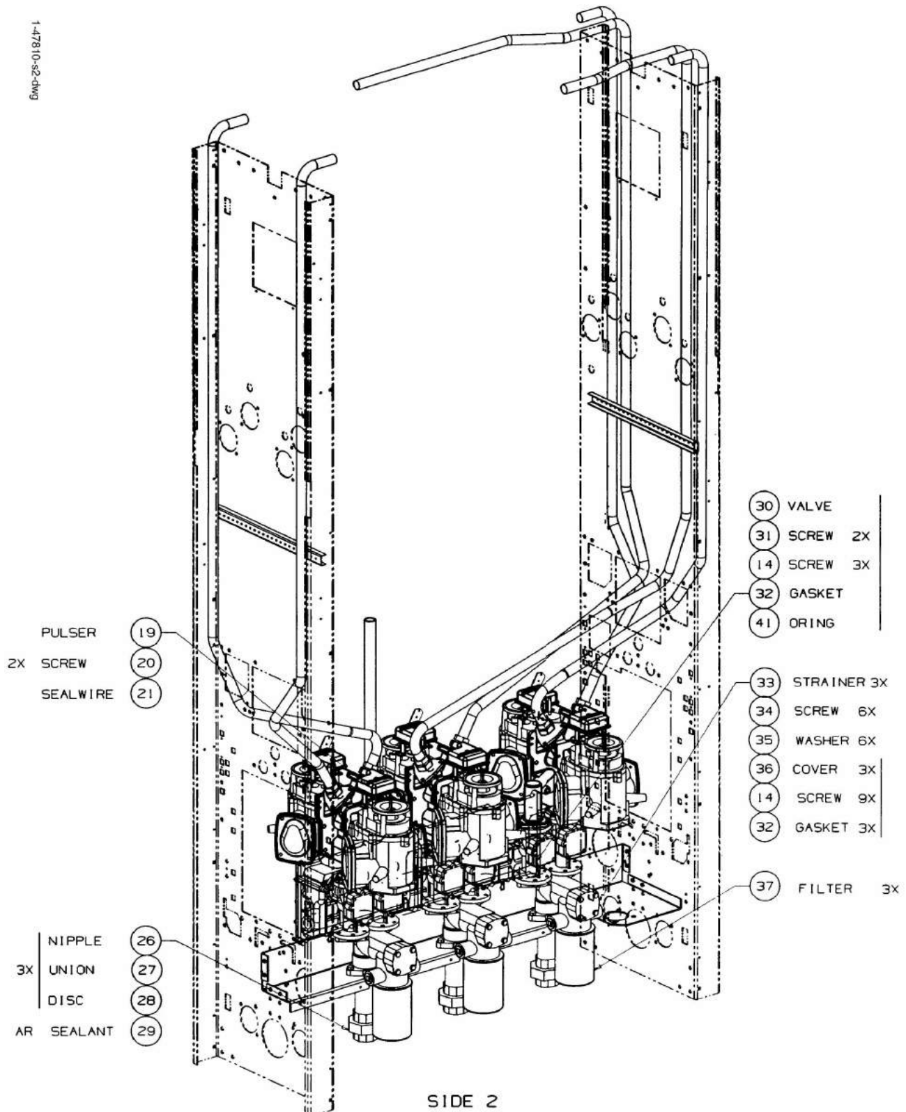
FIGURE 7. 1-47810-S2-DWG - HYDRAULICS MODULE V390D/G
