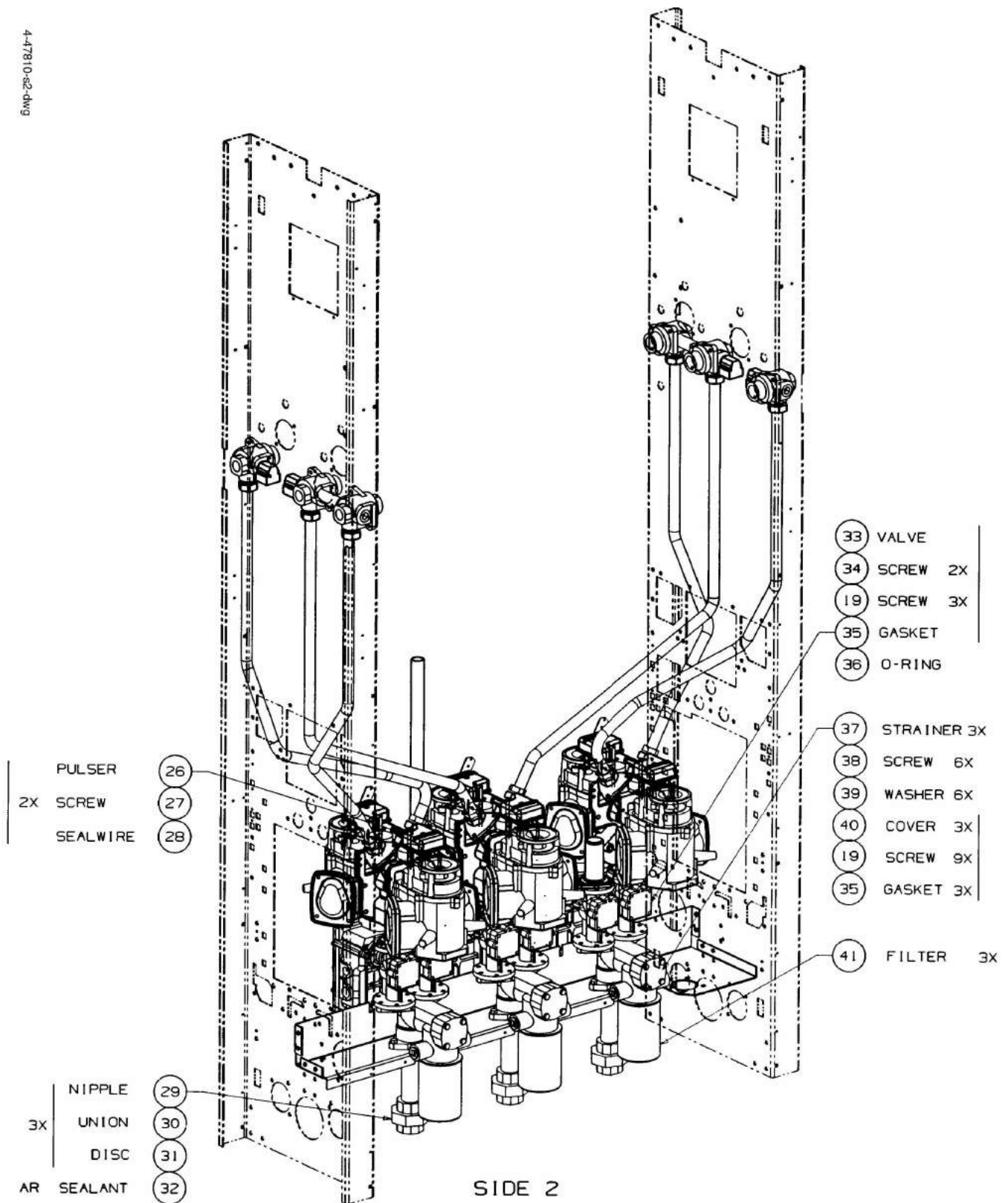
FIGURE 13. 4-47810-S2-DWG - HYDRAULICS MODULE V390D/V
