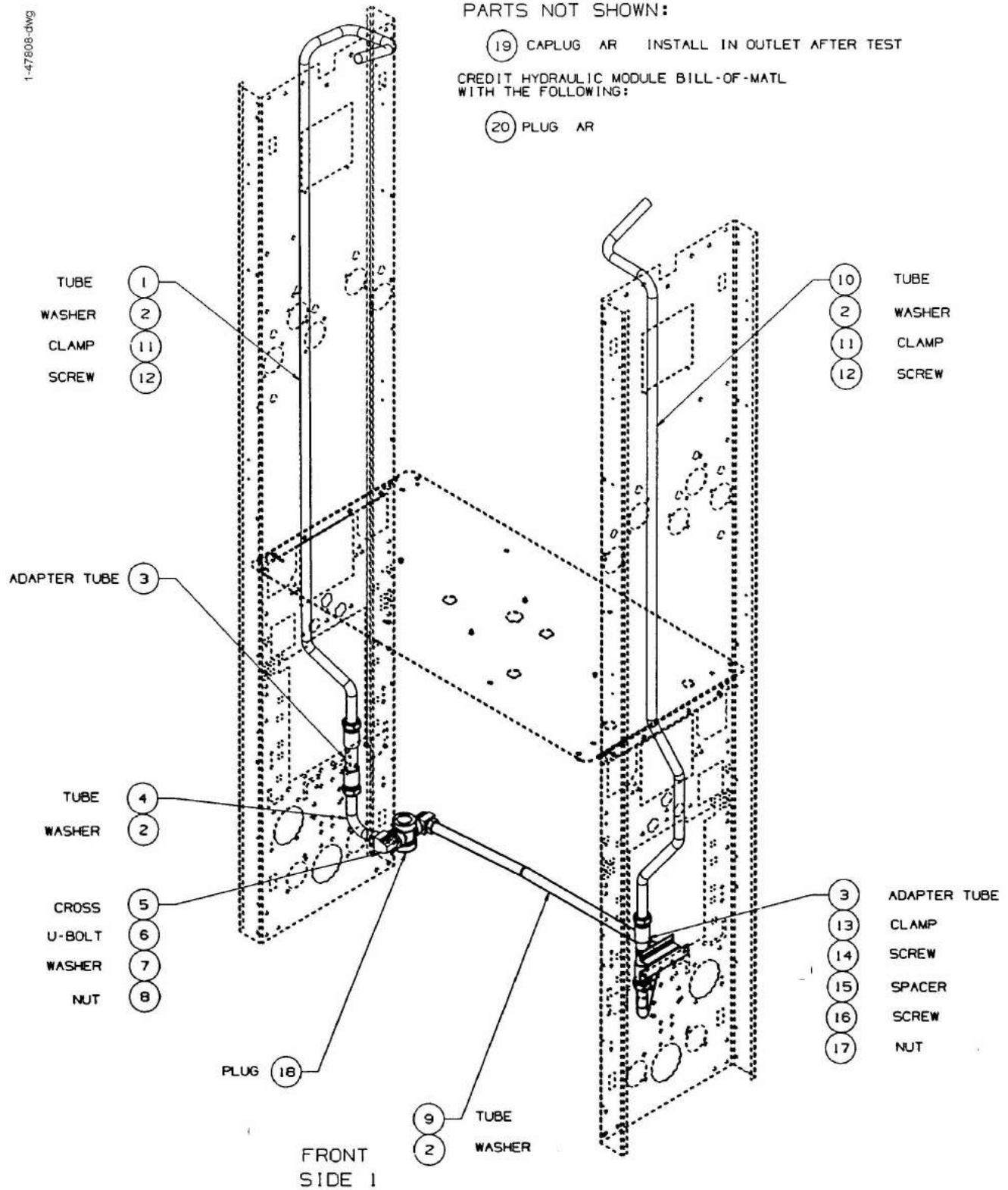
FIGURE 21. 1-47808-DWG - VAPOR RECOVERY BALANCE MODULE
