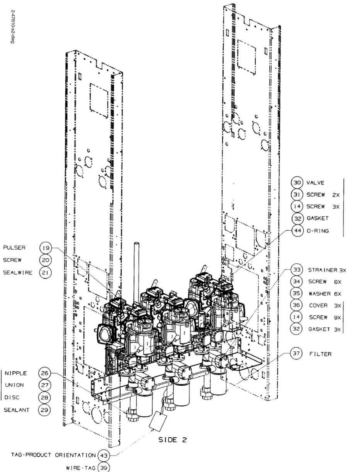
FIGURE 9. 2-47810-S2-DWG - HYDRAULICS MODULE V390D/GU
