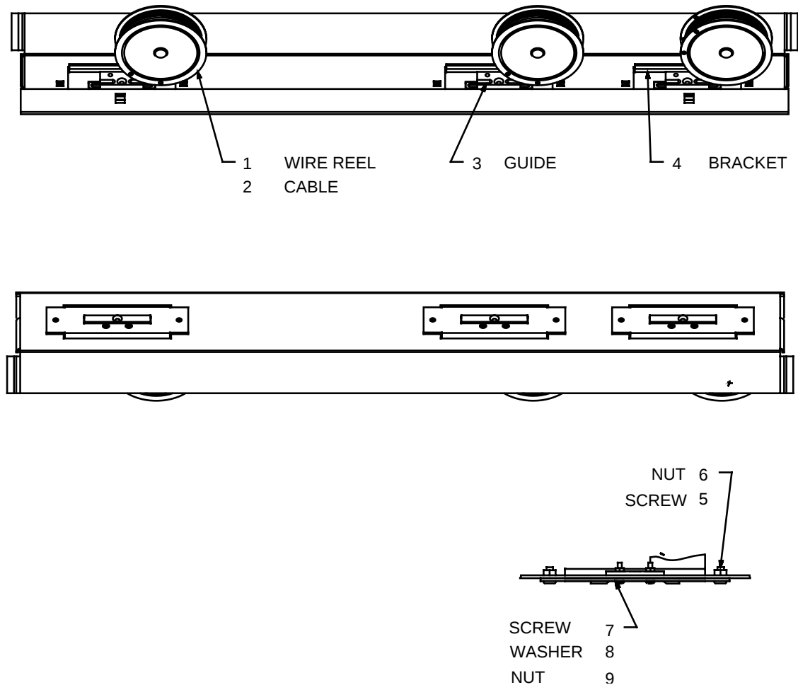
FIGURE 96. 1-47825-DWG - TOP ASSEMBLY MODULE
