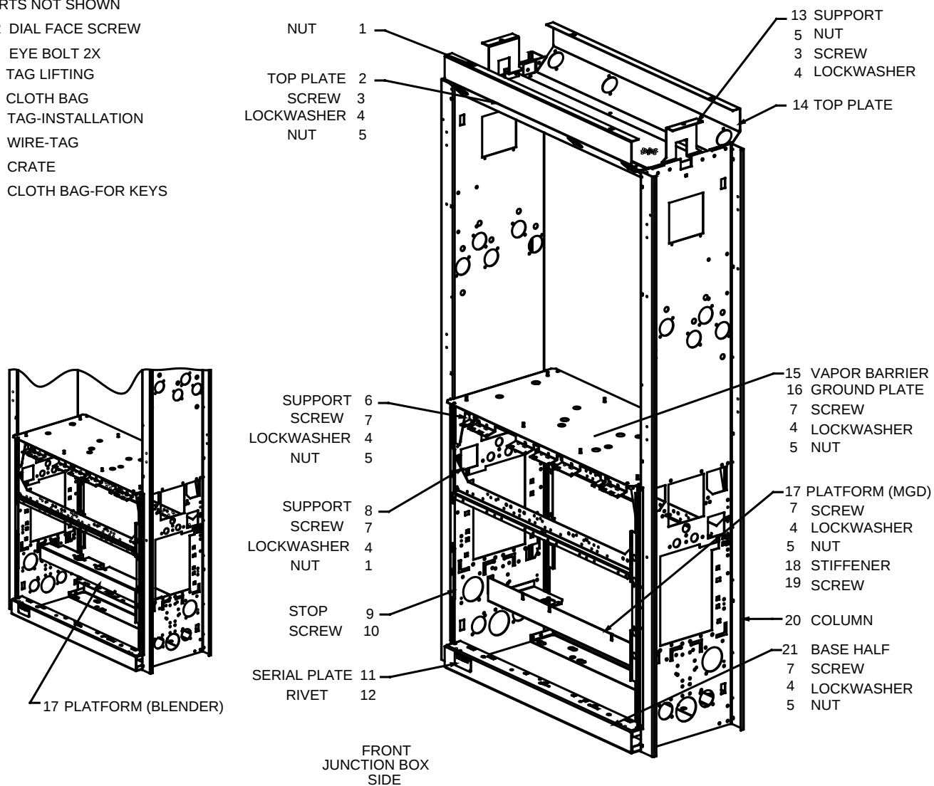
FIGURE 3. 1-47812-DWG - WIDE FRAME MODULE
