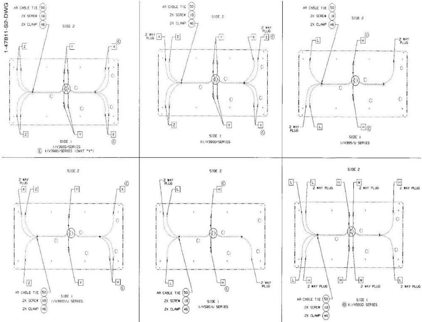
FIGURE 34. 1-47811-S2-DWG - ELECTRICAL MODULE V390D/G
