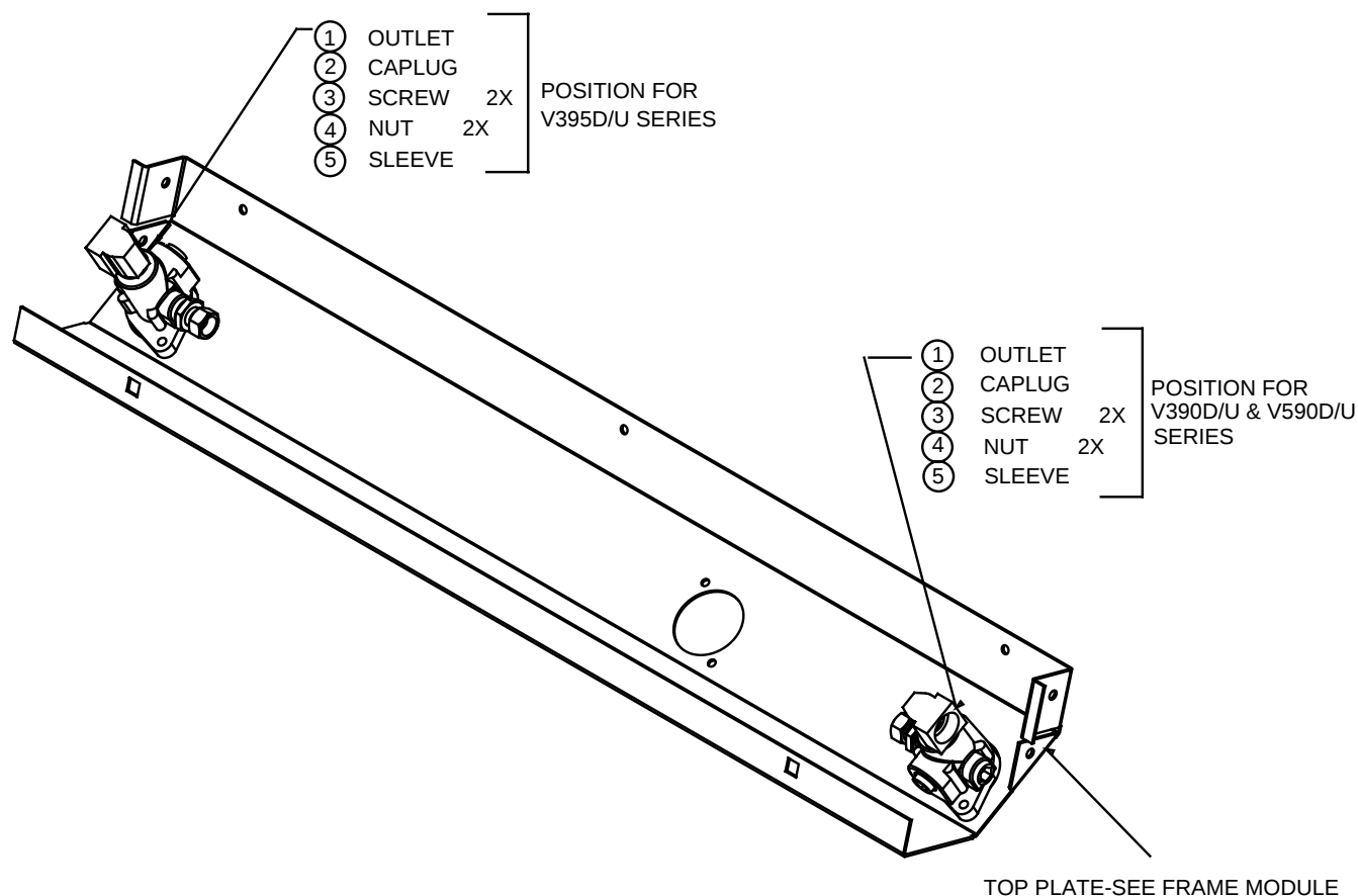
FIGURE 87. 3-47816-DWG - TOP ASSEMBLY MODULE
