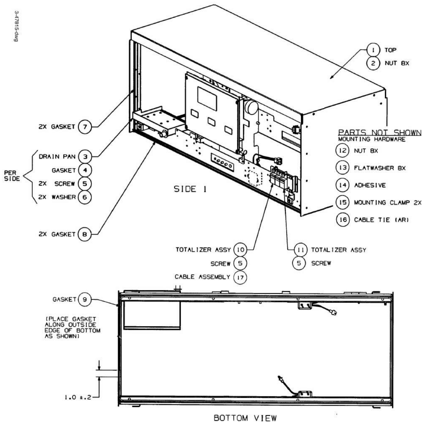
FIGURE 47. 3-47815-DWG - CATS HEAD MODULE PTS
