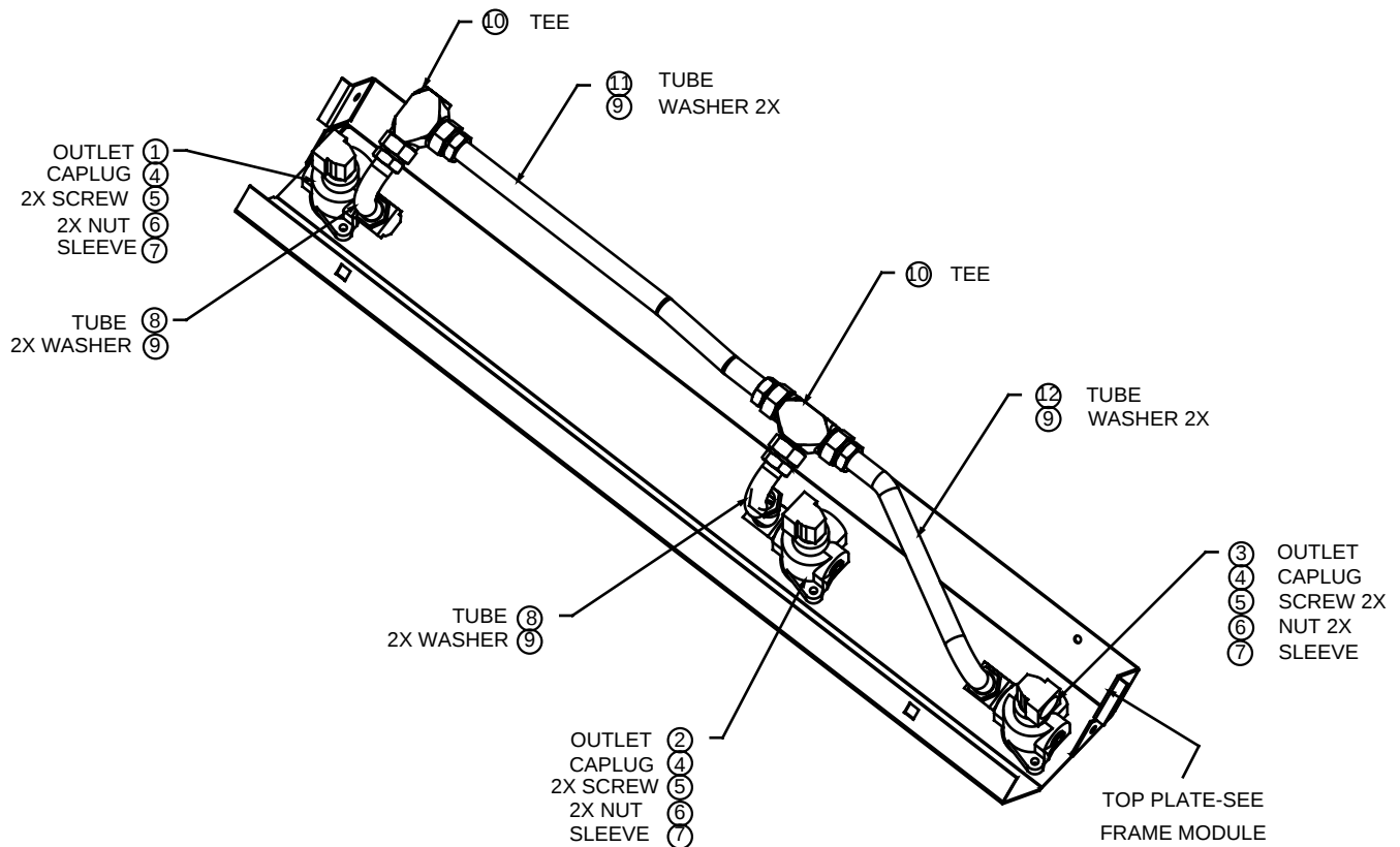
FIGURE 88. 5-47816-DWG - TOP ASSEMBLY MODULE
