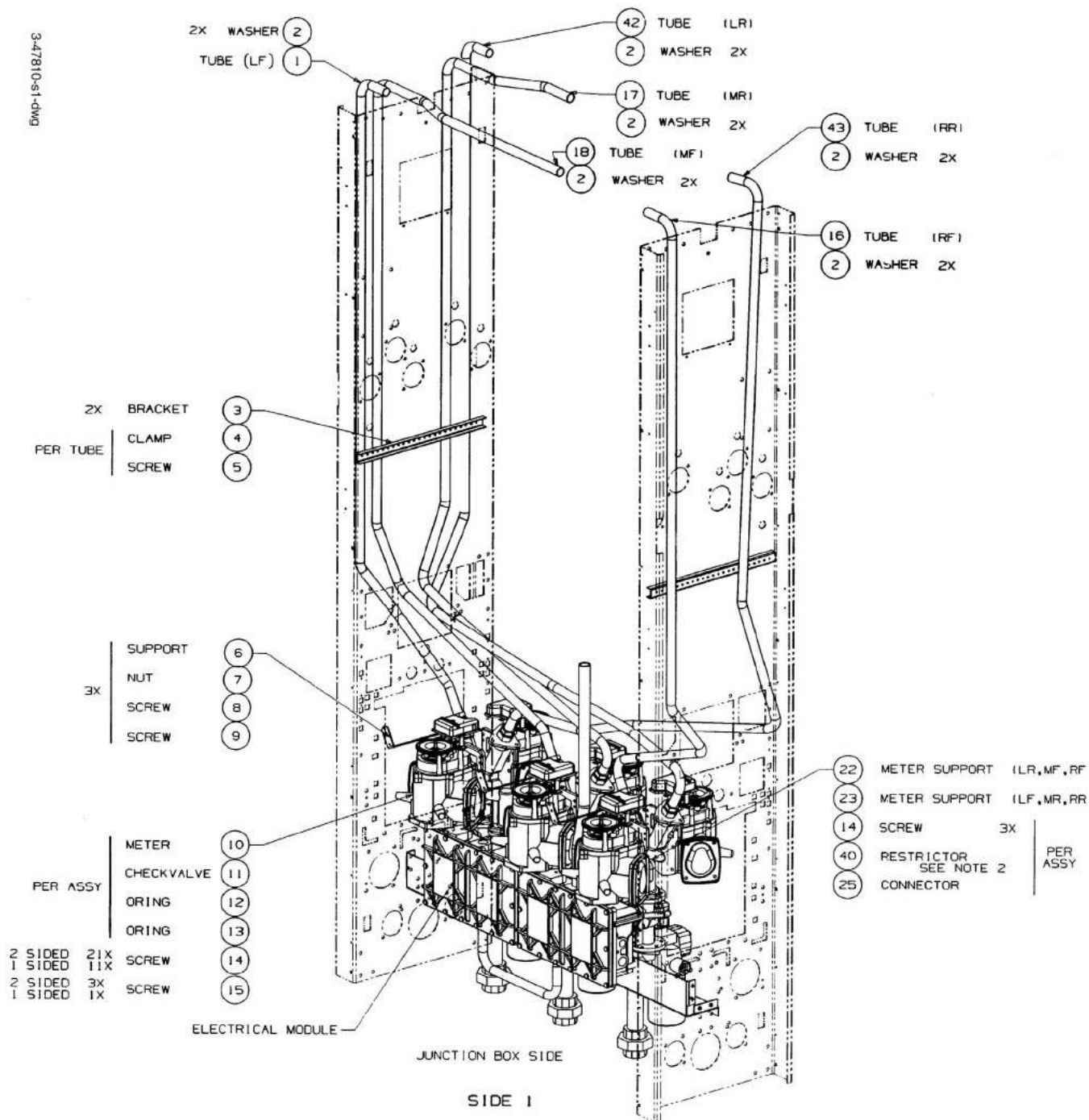
FIGURE 10. 3-47810-S1-DWG - HYDRAULICS MODULE X1/V390/G
