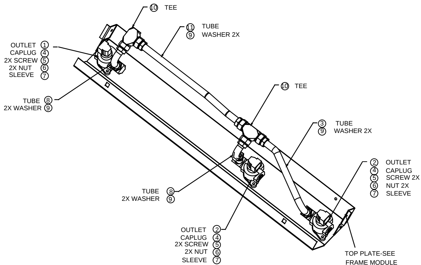
FIGURE 89. 6-47816-DWG - TOP ASSEMBLY MODULE
