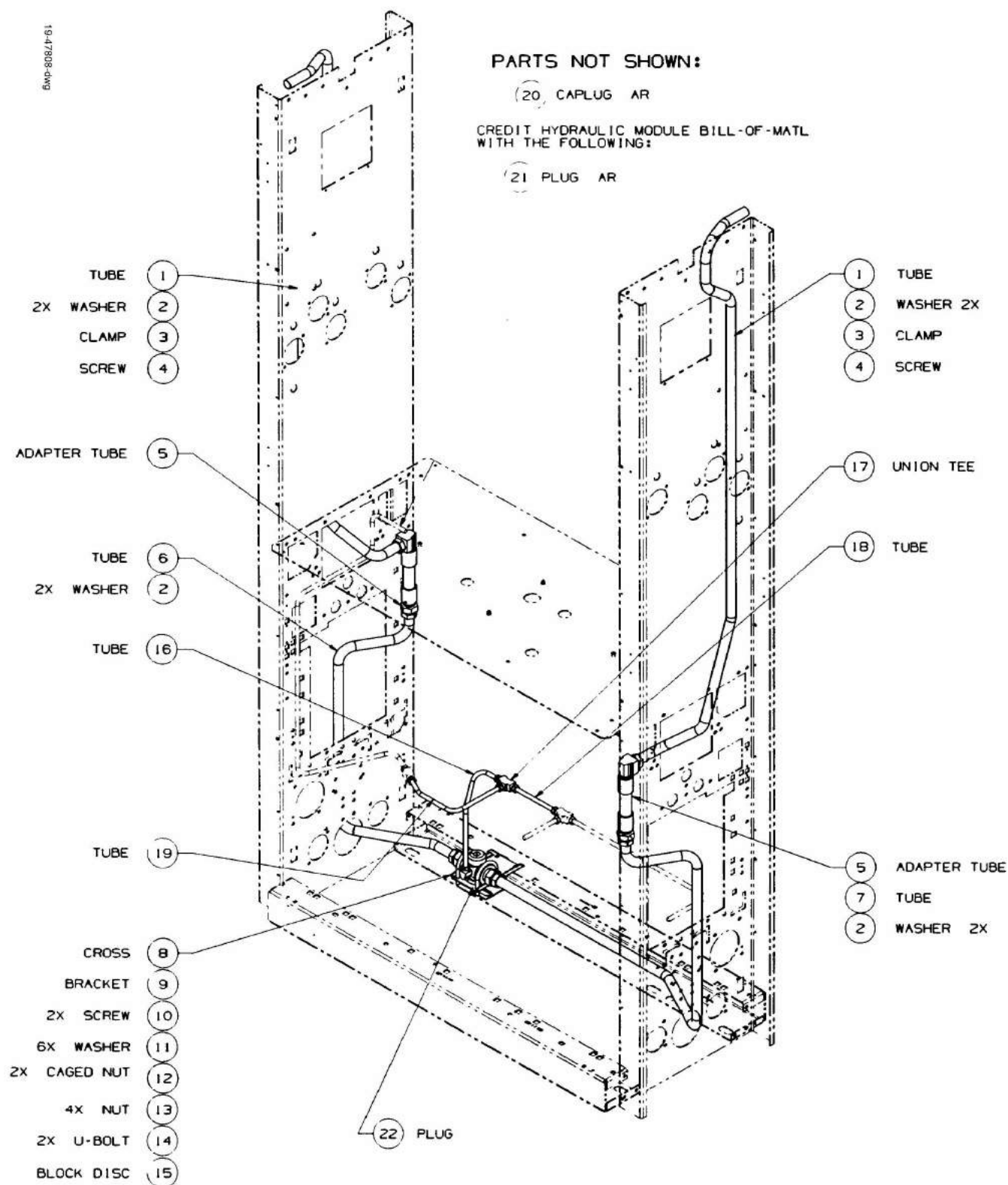
FIGURE 24. 19-47808-DWG - VAPOR RECOVERY BALANCE MODULE V390P/Q
