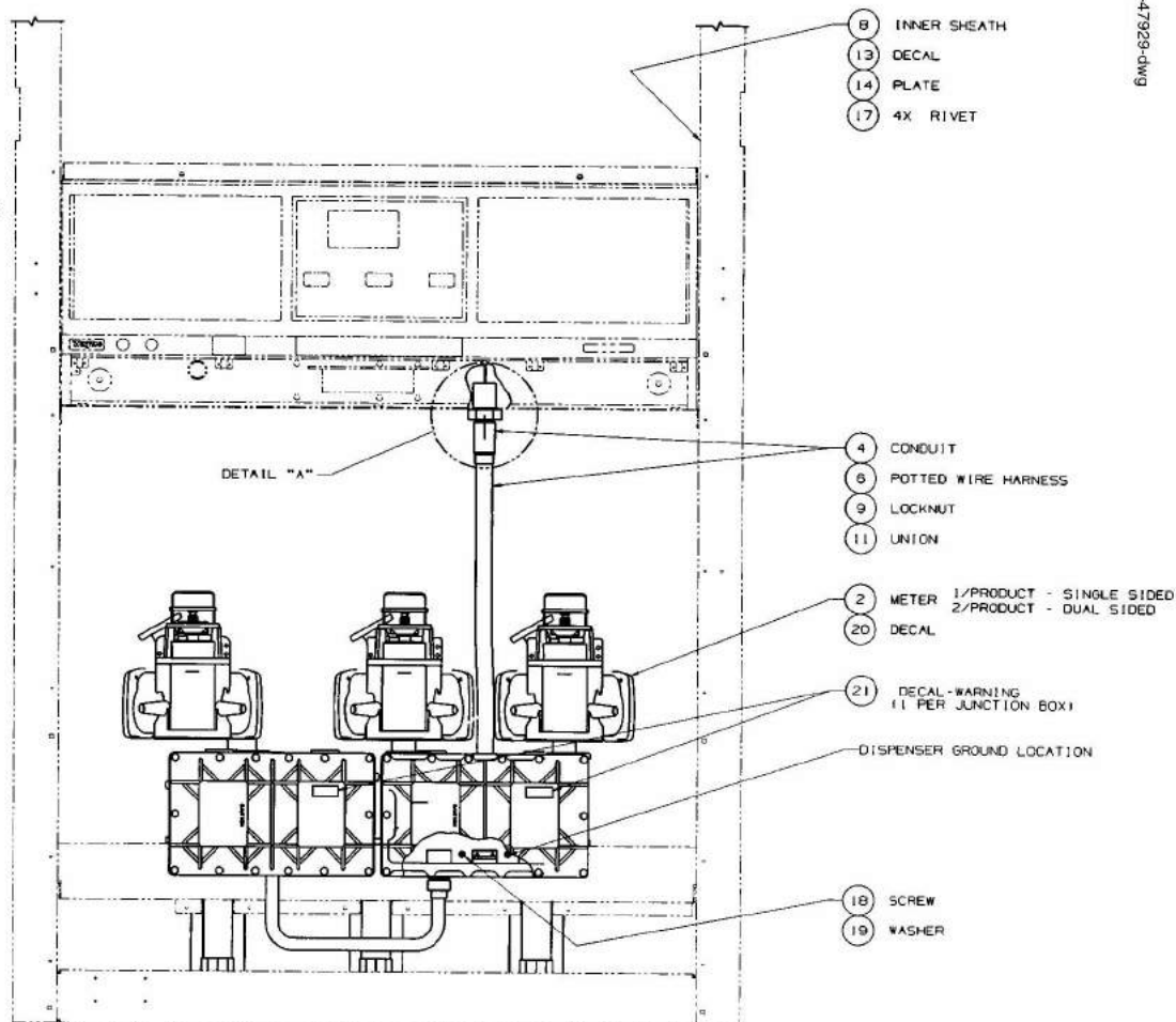
FIGURE 97. 1-47929-DWG - CANADA MODULE 1/V
