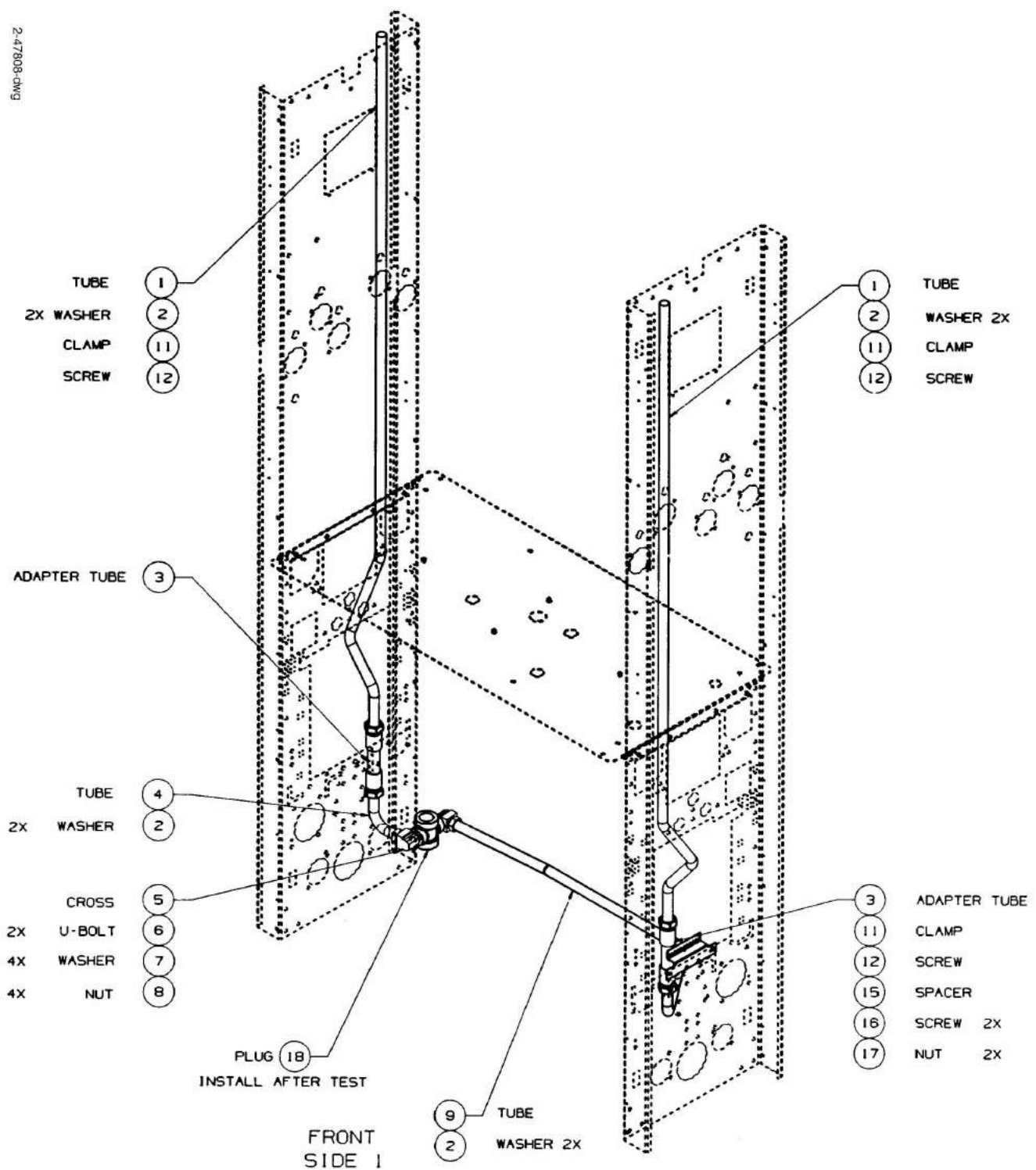
FIGURE 22. 2-47808-DWG - VAPOR RECOVERY BALANCE MODULE V390
