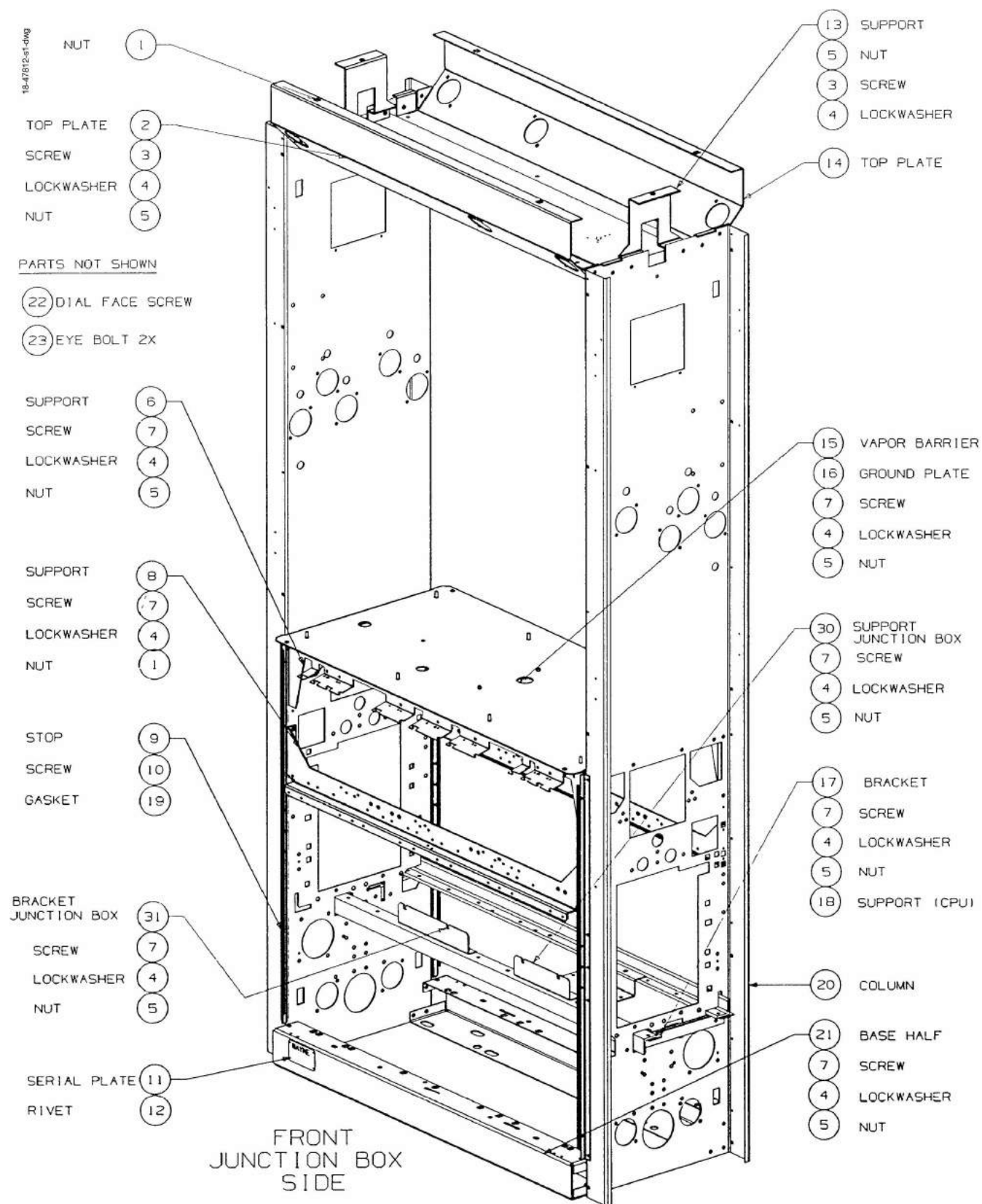
FIGURE 4. 18-47812-DWG - FRAME MODULE
