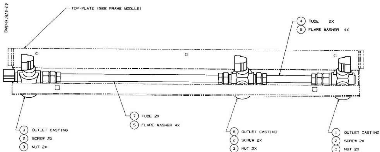
FIGURE 93. 42-47816-DWG - TOP MODULE 1/V390P/Q
