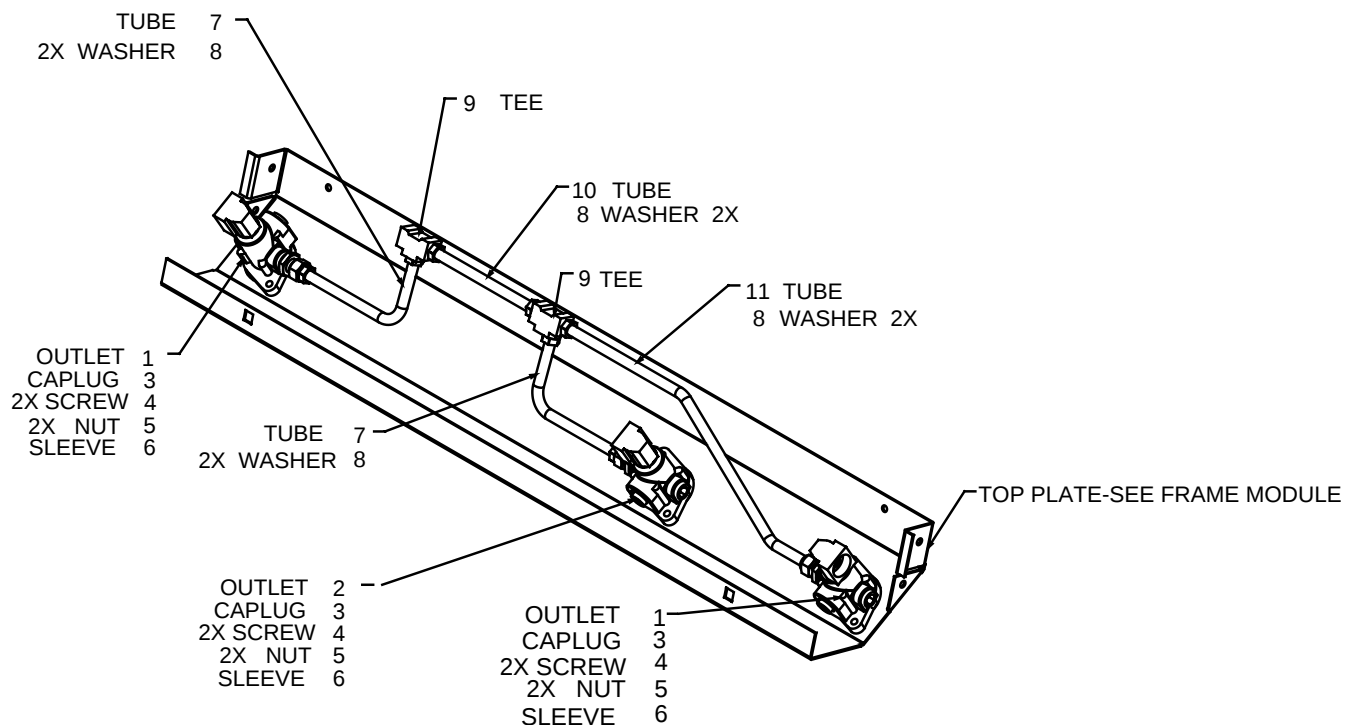
FIGURE 85. 1-47816-DWG - TOP MODULE
