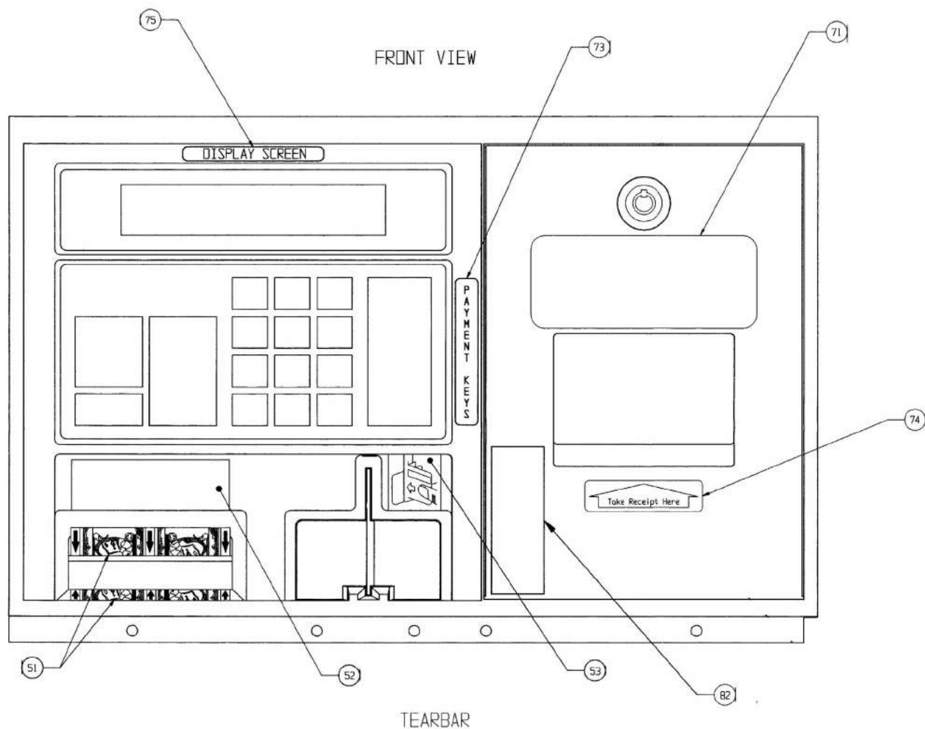
FIGURE 57. 881784-S2 - CUSTOMER PAYMENT MODULE
