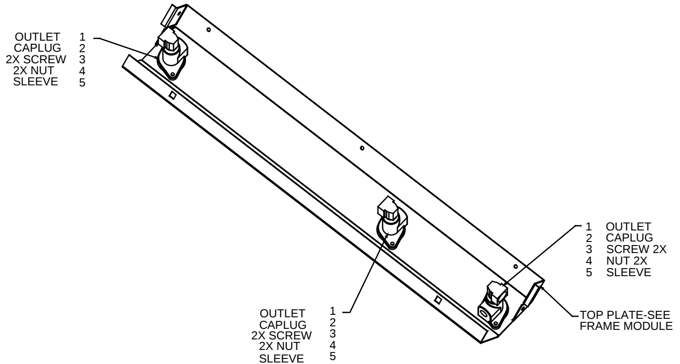
FIGURE 90. 9-47816-DWG - TOP ASSEMBLY MODULE
