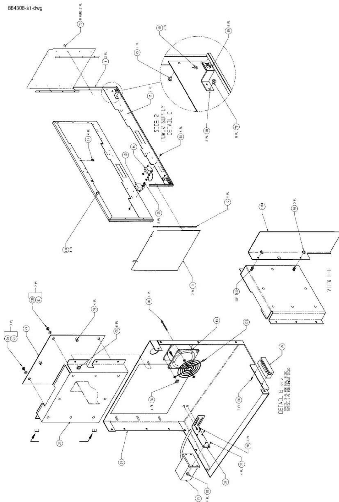
FIGURE 74. 884308-S1 - PUMP HEAD SUBASSEMBLY
