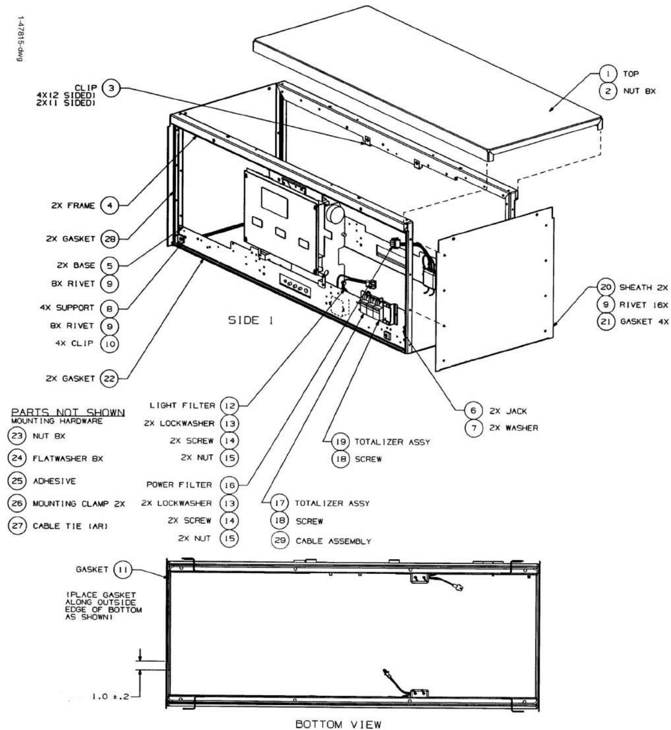
FIGURE 46. 1-47815-DWG - HEAD MODULE V390
