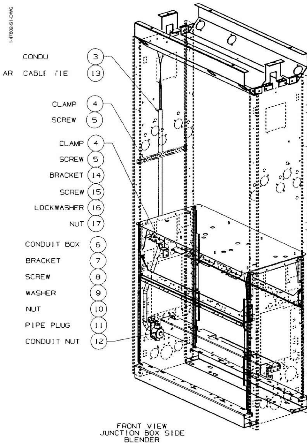
FIGURE 37. 1-47802-S1-DWG - SPEAKER MODULE
