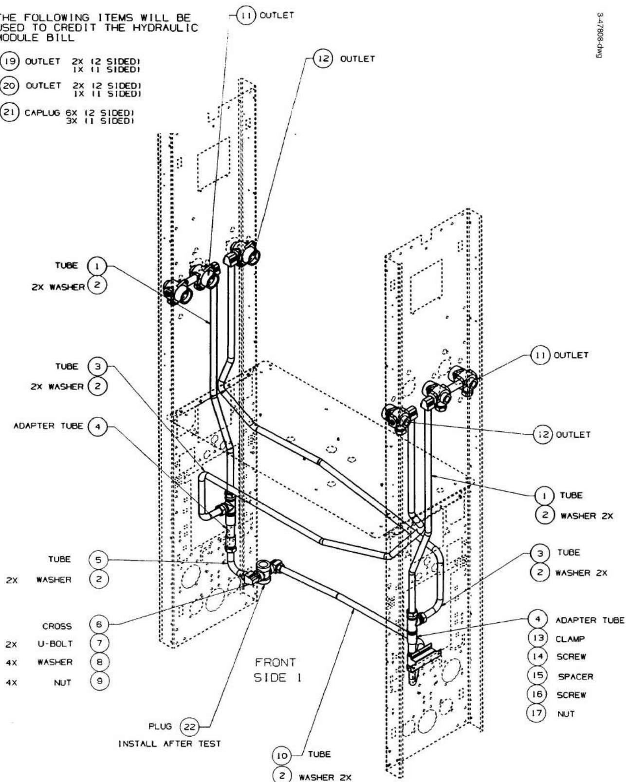
FIGURE 23. 3-47808-DWG - VAPOR RECOVERY BALANCE MODULE V390/V
