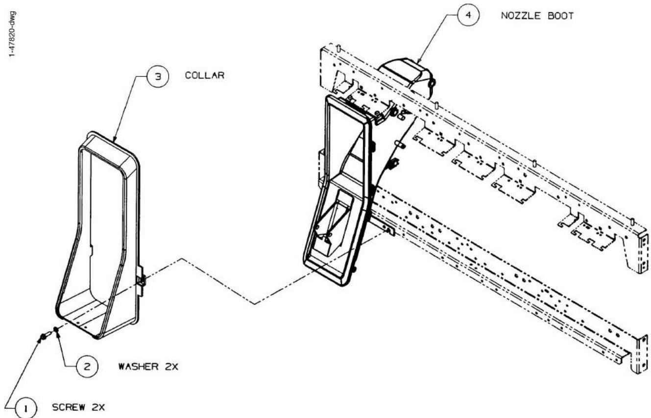
FIGURE 31. 1-47820-DWG - NOZZLE BOOT MODULE LTS
