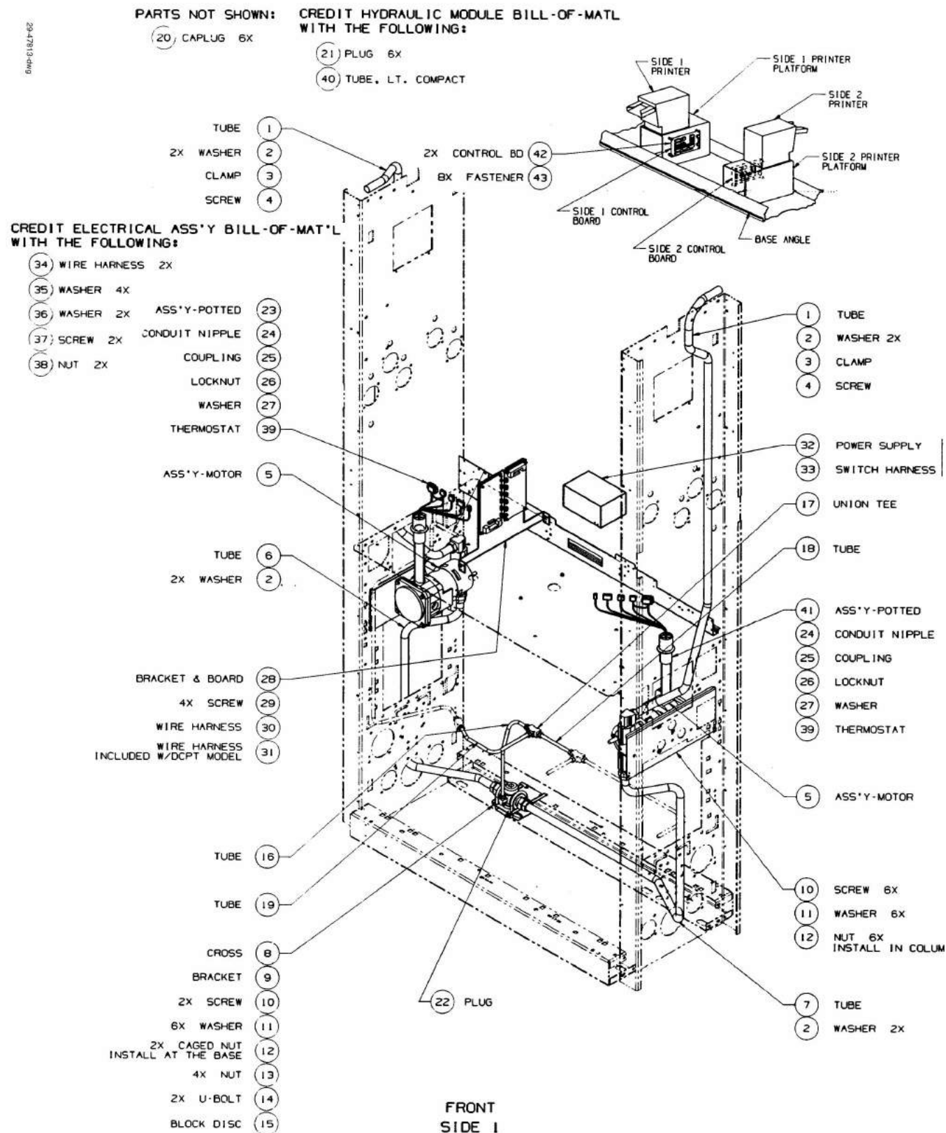
FIGURE 29. 29-47813-DWG - VAPOR RECOVERY MODULE V390P4/D2
