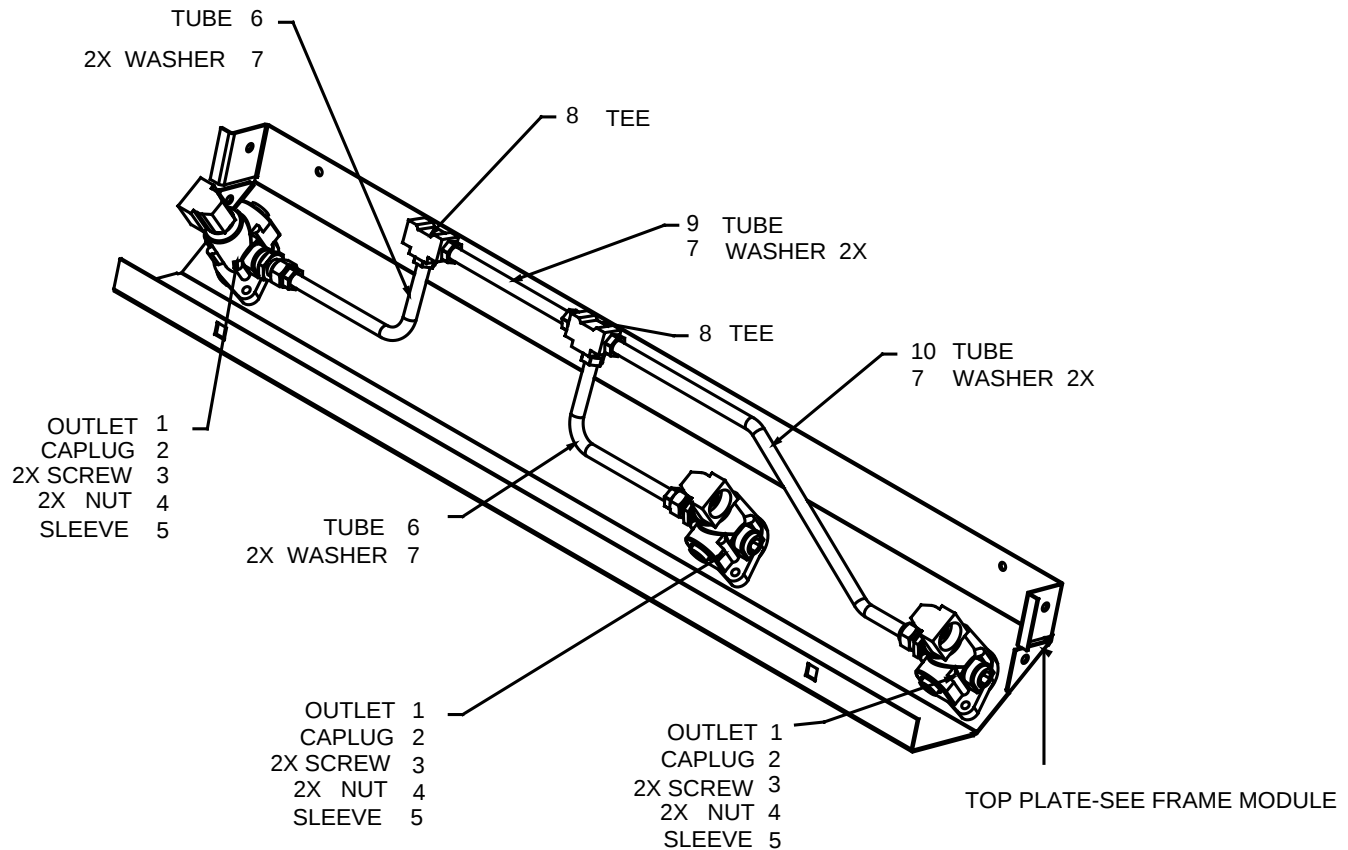
FIGURE 86. 2-47816-DWG - TOP ASSEMBLY MODULE
