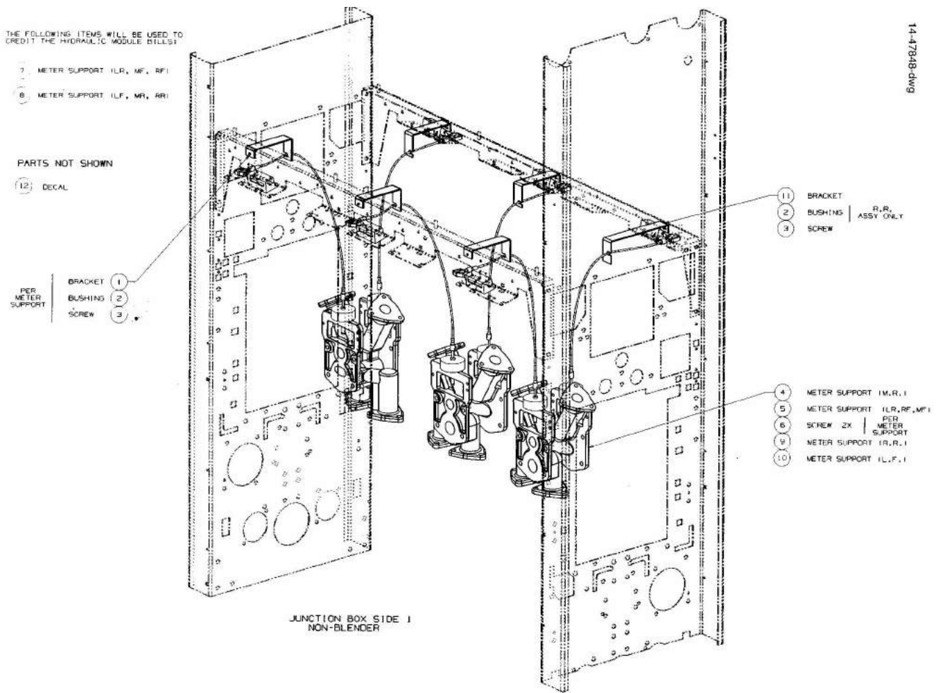
FIGURE 19. 14-47848-DWG - MECHANICAL TOTALIZER MODULE V390P
