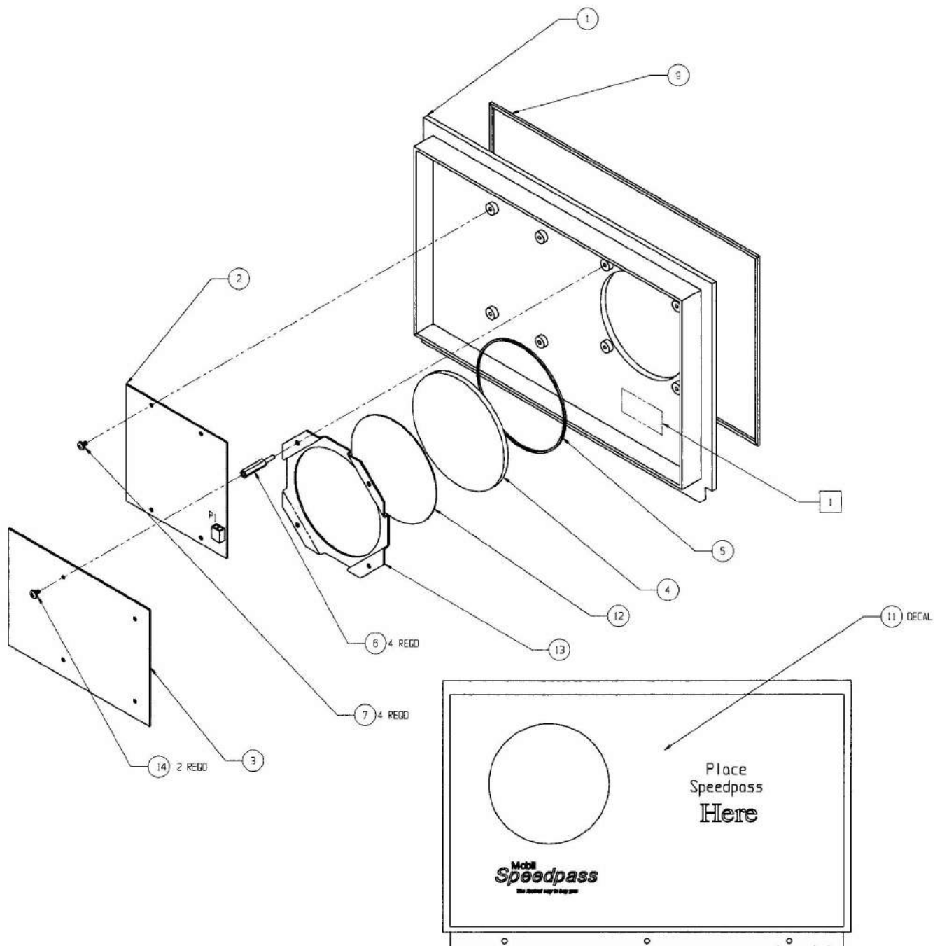
FIGURE 44. 884212 - BEZEL WAYNE TRAC CID SIDE 1 AUTHORIZE LIGHT
