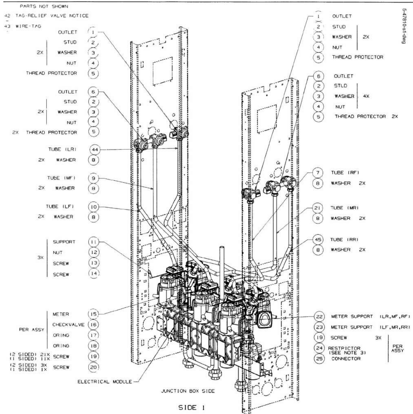
FIGURE 14. 5-47810-S1-DWG - HYDRAULICS MODULE X1/V390D/V
