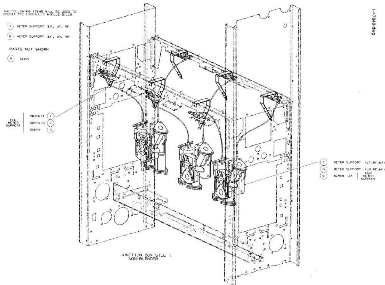
FIGURE 18. 1-47848-DWG - MECHANICAL TOTALIZER MODULE V390
