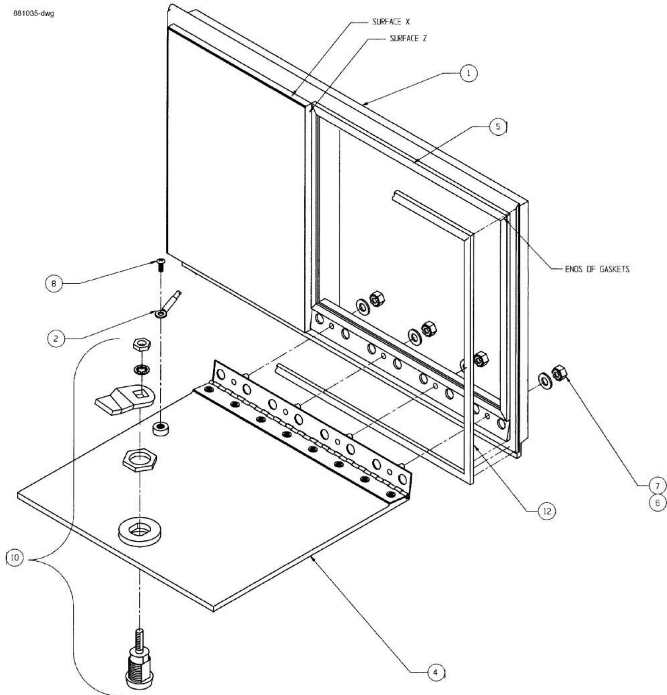
FIGURE 43. 881035 - BEZEL ASSEMBLY
