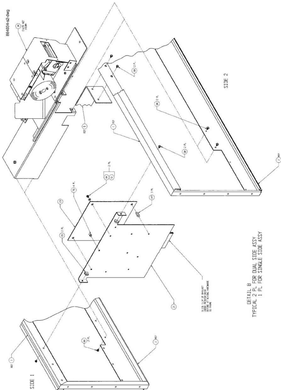
FIGURE 71. 884034-S2 - PUMP HEAD SUBASSEMBLY
