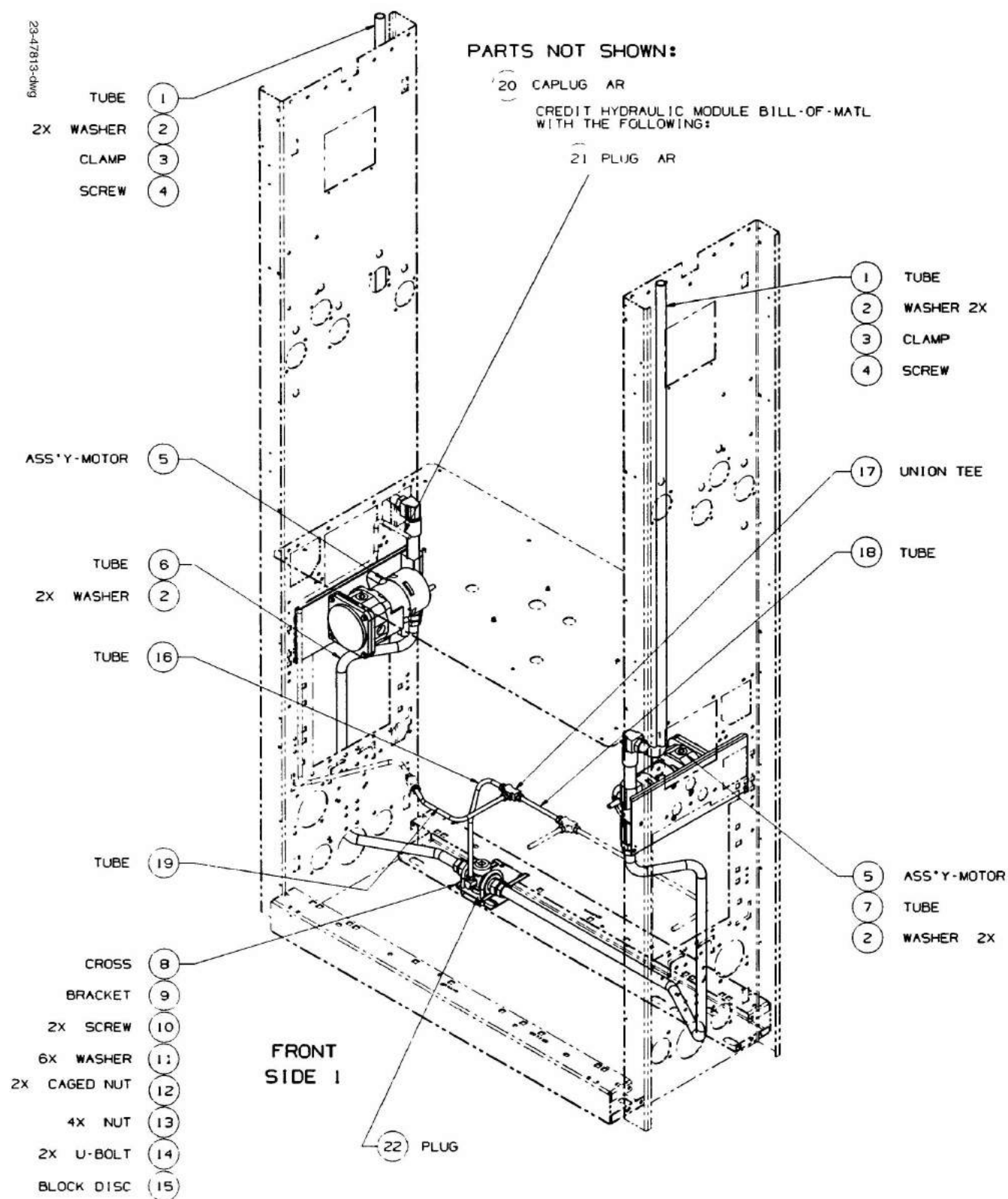
FIGURE 28. 23-47813-DWG - VAPOR RECOVERY MODULE V390P/D2QU
