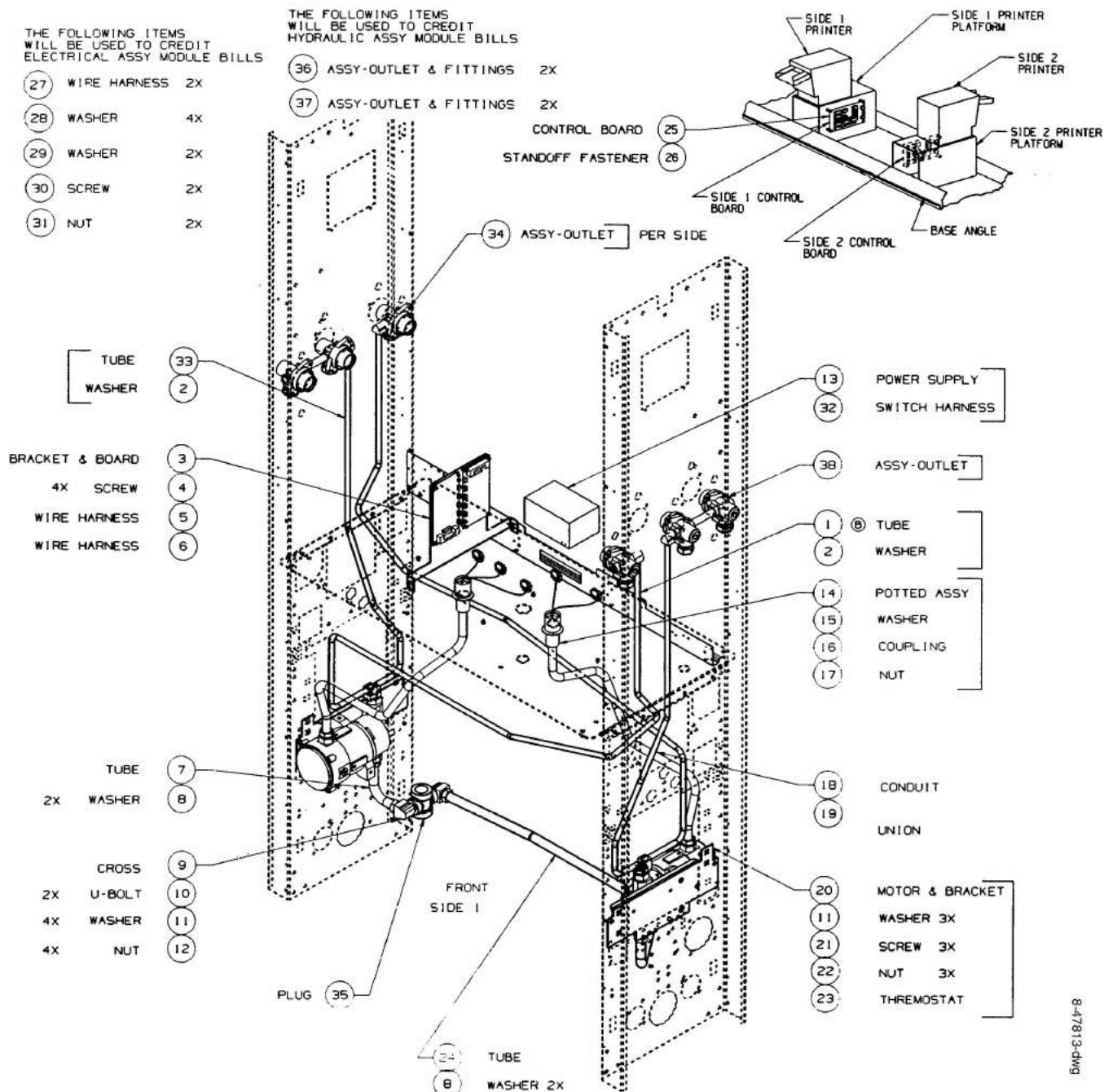
FIGURE 27. 8-47813-DWG - VAPOR RECOVERY MODULE V390/V
