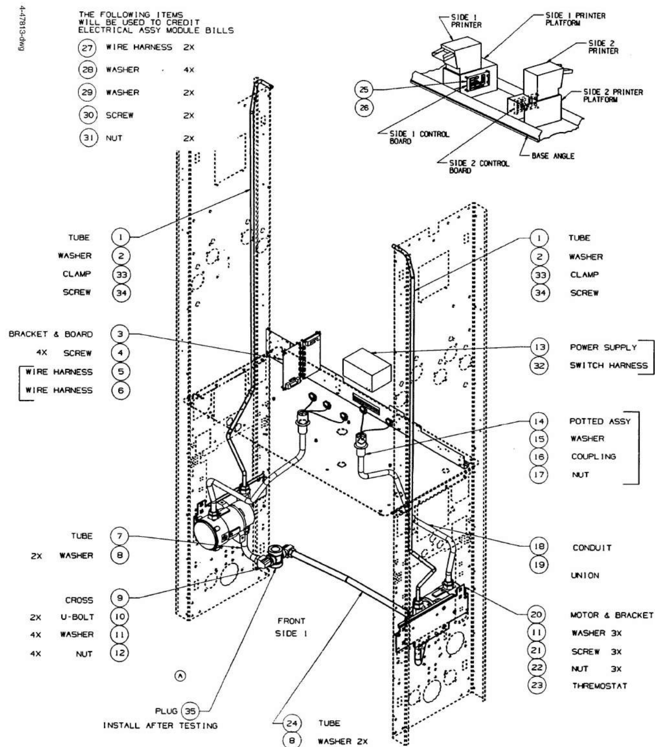
FIGURE 26. 4-47813-DWG - VAPOR RECOVERY MODULE V390D/D2GU
