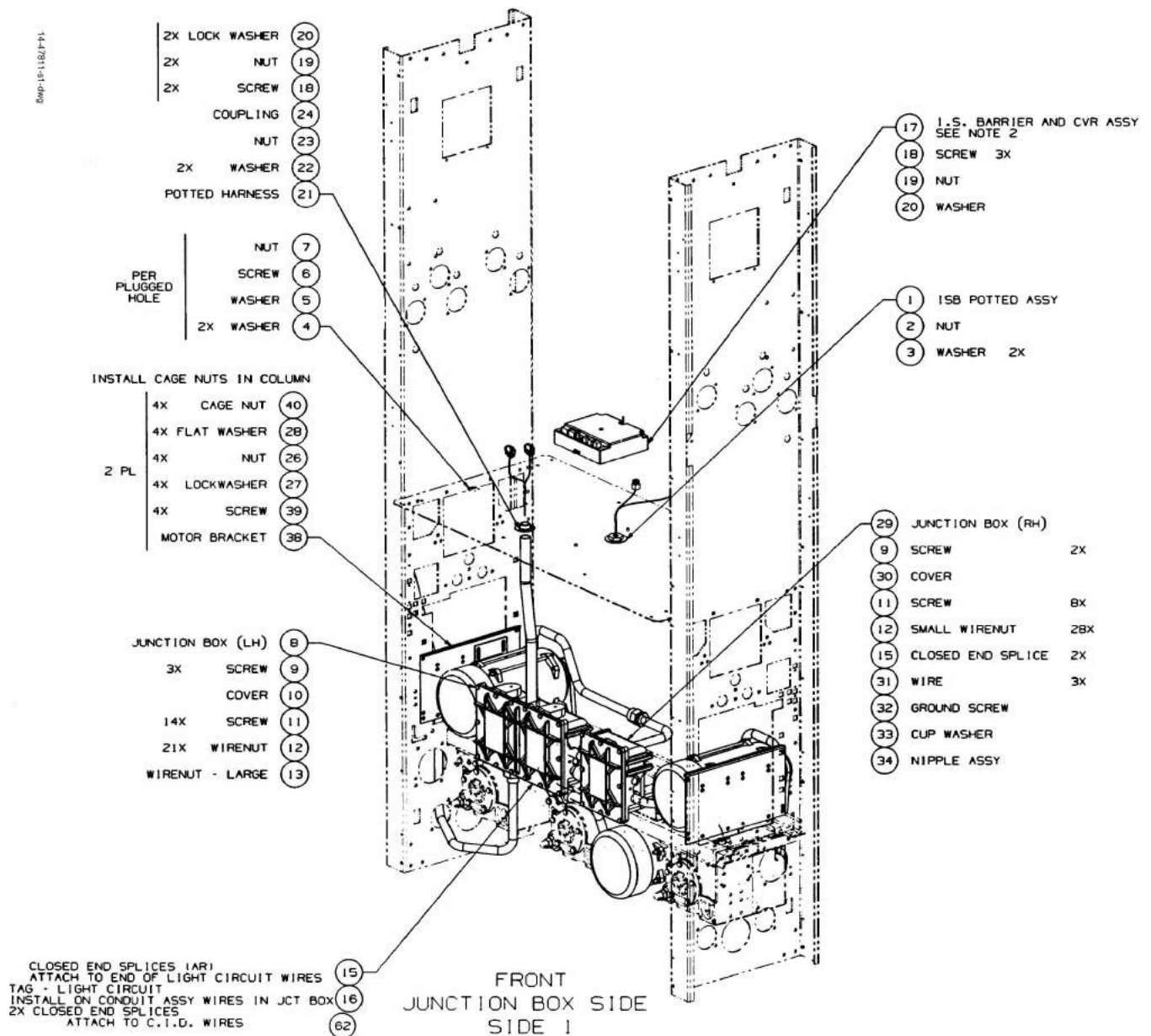
FIGURE 35. 14-47811-S1-DWG - ELECTRICAL MODULE
