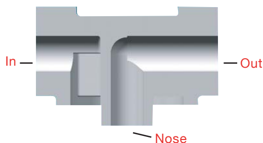
Section View 50003 Adaptor
